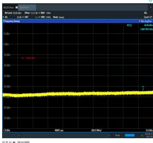
Band13-5MHz-16QAM-23255-1RB#0-1000~300 0-PASS
