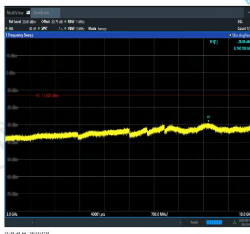
Band13-5MHz-16QAM-23255-25RB#0-3000~10000-PASS
