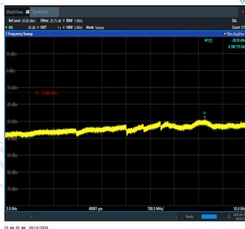
Band13-10MHz-16QAM-23230-1RB#0-3000~10 000-PASS
