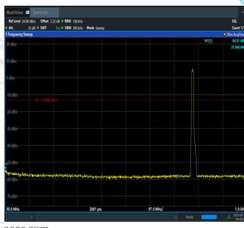
Band13-10MHz-16QAM-23230-50RB#0-30~100 0-PASS
