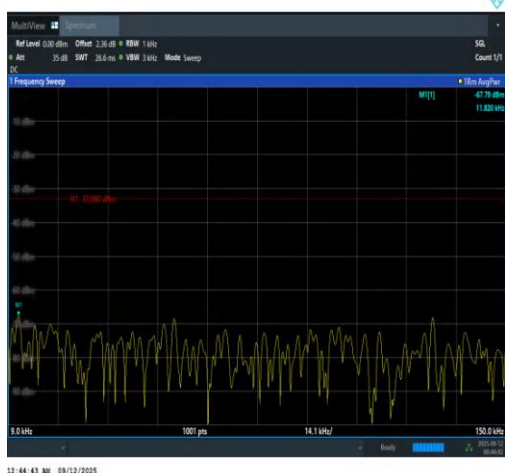
Band13-10MHz-16QAM-23230-1RB#49-0.009~0 .15-PASS
