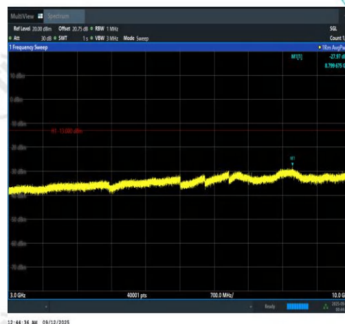
Band13-10MHz-QPSK-23230-1RB#49-3000~10 000-PASS
