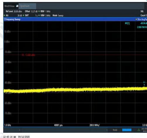
Band13-10MHz-QPSK-23230-1RB#0-1000~300 0-PASS
