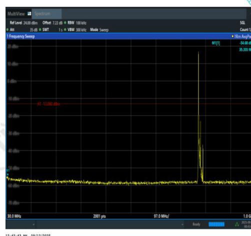
Band13-10MHz-16QAM-23230-1RB#0-30~1000-PASS
