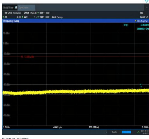
Band13-10MHz-16QAM-23230-50RB#0-1000~3 000-PASS
