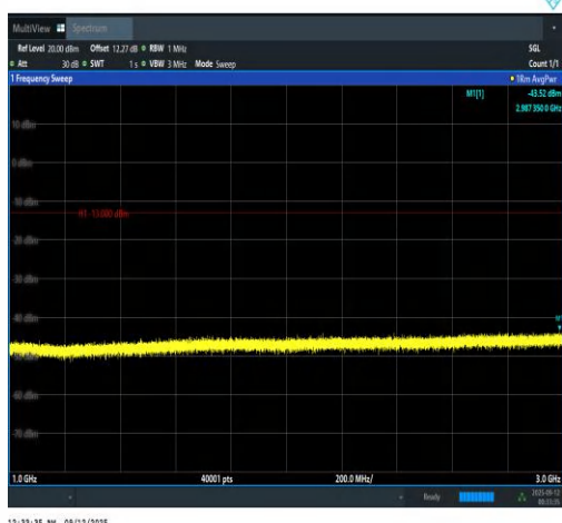
Band13-5MHz-16QAM-23255-25RB#0-1000~3000-PASS
