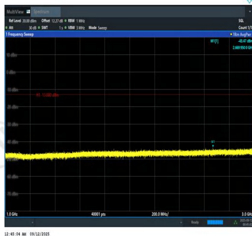
Band13-10MHz-16QAM-23230-1RB#49-1000~3 000-PASS
