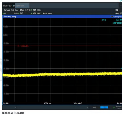
Band13-5MHz-16QAM-23255-1RB#24-1000~30 00-PASS
