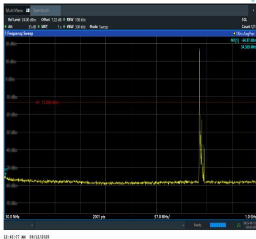
Band13-10MHz-QPSK-23230-1RB#0-30~1000-P ASS
