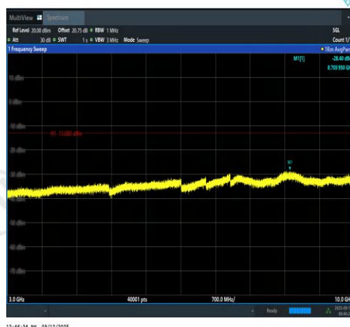
Band13-10MHz-16QAM-23230-50RB#0-3000~1 0000-PASS
