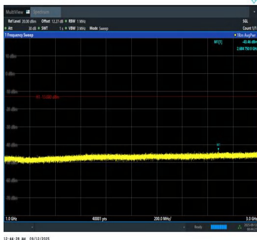
Band13-10MHz-QPSK-23230-1RB#49-1000~30 00-PASS
