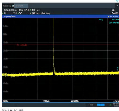
Band2-3MHz-16QAM-18900-15RB#0-1000~300 0-PASS
