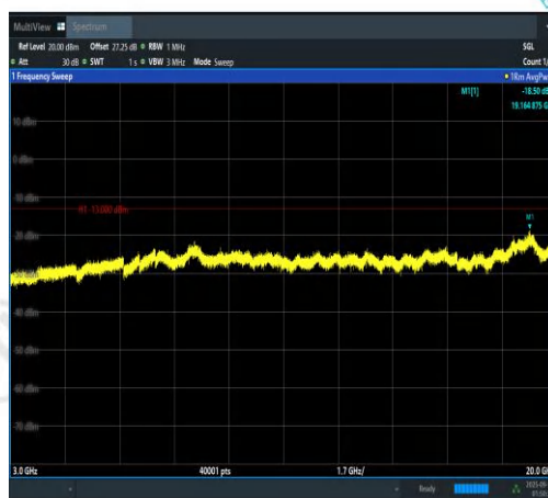
Band2-3MHz-16QAM-18900-15RB#0-3000~200 00-PASS
