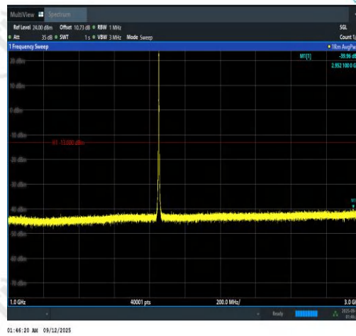
Band2-3MHz-QPSK-18615-15RB#0-1000~3000-PASS
