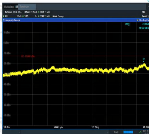
Band2-3MHz-16QAM-18615-15RB#0-3000~200 00-PASS
