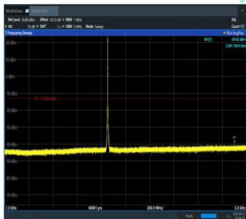
Band2-3MHz-16QAM-18615-15RB#0-1000~300 0-PASS
