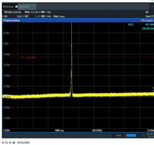
Band2-3MHz-16QAM-19185-1RB#0-1000~3000-
