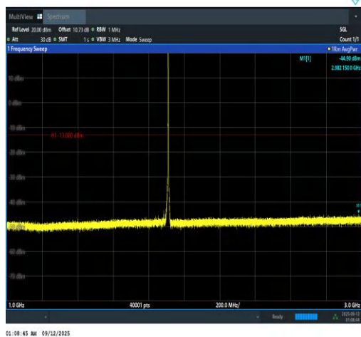
Band2-1.4MHz-16QAM-19193-6RB#0-1000~300
