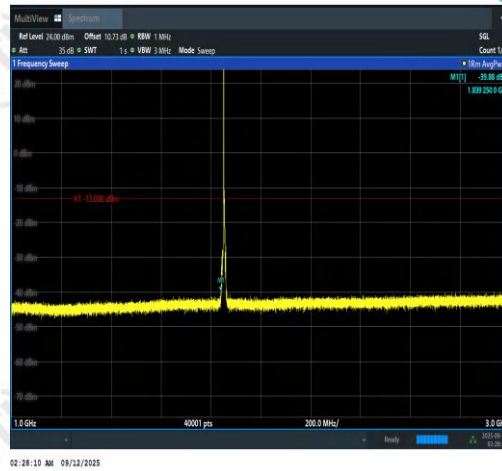
Band2-5MHz-QPSK-18625-1RB#0-1000~3000-P ASS
