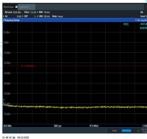
Band2-3MHz-16QAM-18900-1RB#0-30~1000-P
