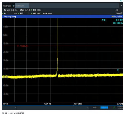
Band2-5MHz-QPSK-19175-1RB#24-1000~3000-PASS
