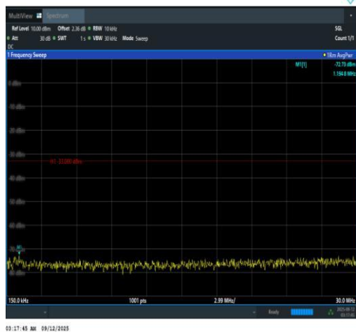
Band2-10MHz-16QAM-18900-50RB#0-0.15~30-PASS
