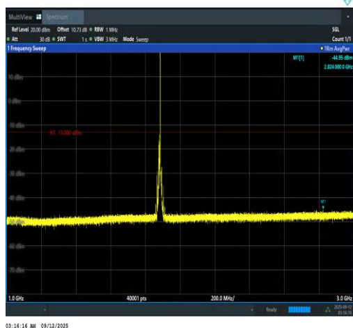
Band2-10MHz-QPSK-18900-1RB#49-1000~300 0-PASS
