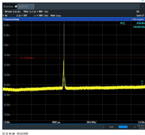
Band2-10MHz-QPSK-18650-1RB#49-1000~300 0-PASS
