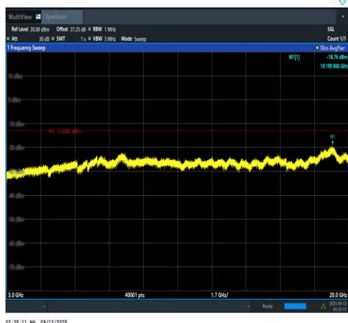
Band2-5MHz-QPSK-19175-1RB#0-3000~20000-PASS
