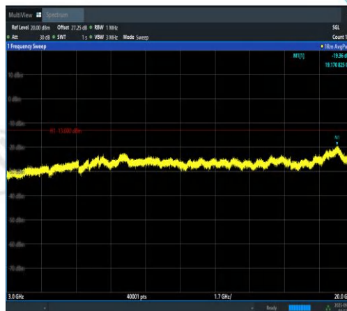
Band2-10MHz-16QAM-18650-1RB#0-3000~200 00-PASS
