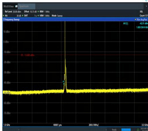
Band2-10MHz-16QAM-18650-1RB#0-1000~300 0-PASS
