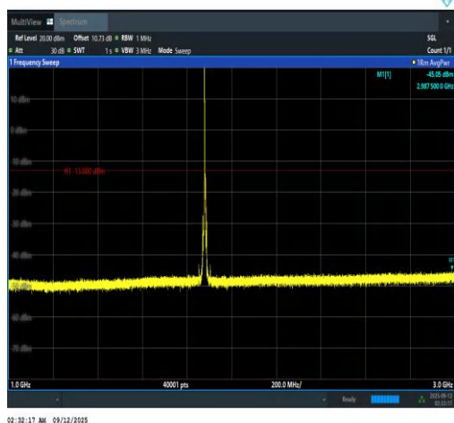
Band2-5MHz-16QAM-18900-1RB#0-1000~3000-PASS
