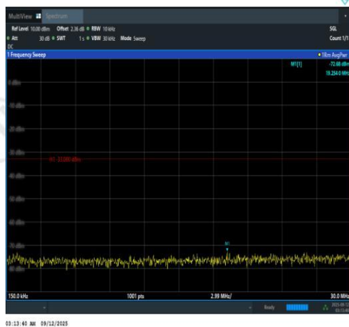
Band2-10MHz-QPSK-18650-50RB#0-0.15~30-P
