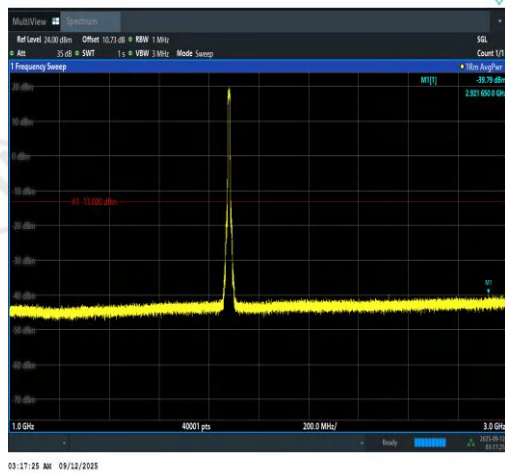
Band2-10MHz-QPSK-18900-50RB#0-1000~300
