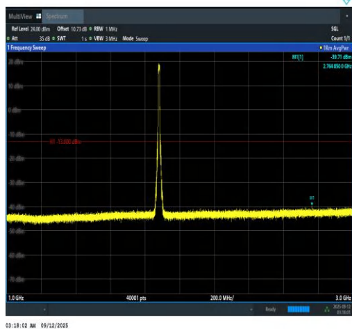
Band2-10MHz-16QAM-18900-50RB#0-1000~3000-PASS
