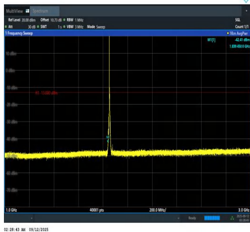
Band2-5MHz-16QAM-18625-1RB#0-1000~3000- PASS
