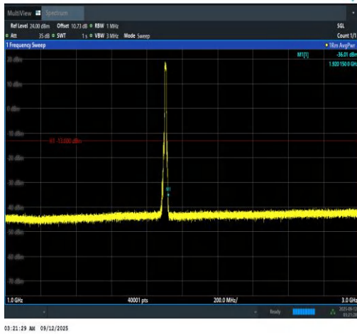
Band2-10MHz-16QAM-19150-50RB#0-1000~3000-PASS
