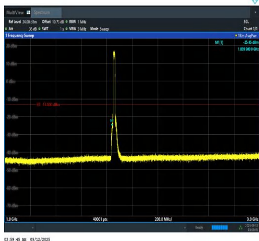
Band2-15MHz-16QAM-18675-75RB#0-1000~30 00-PASS
