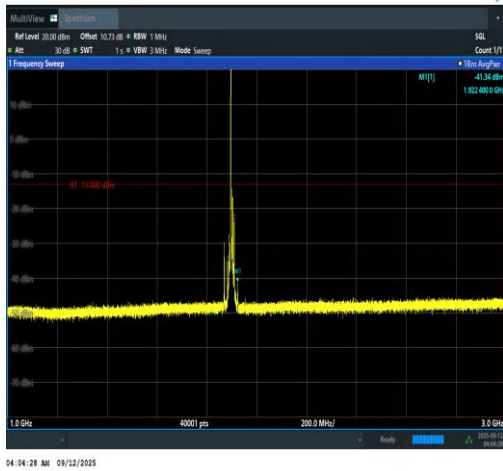
Band2-15MHz-16QAM-19125-1RB#0-1000~300 0-PASS
