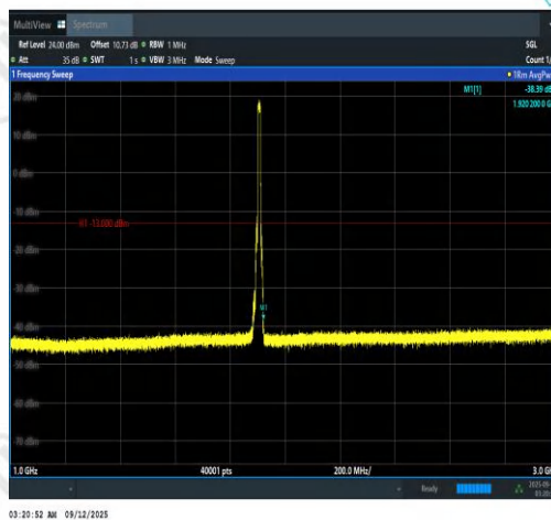
Band2-10MHz-QPSK-19150-50RB#0-1000~300 0-PASS
