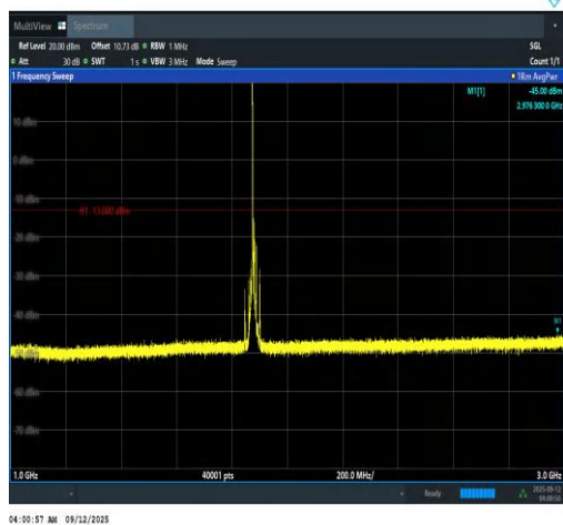
Band2-15MHz-16QAM-18900-1RB#0-1000~300
