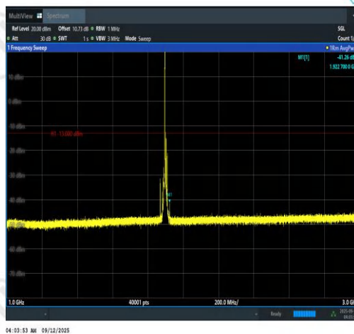
Band2-15MHz-QPSK-19125-1RB#0-1000~3000- PASS
