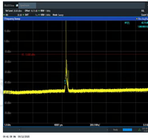
Band2-20MHz-QPSK-18700-1RB#0-1000~3000-P PASS
