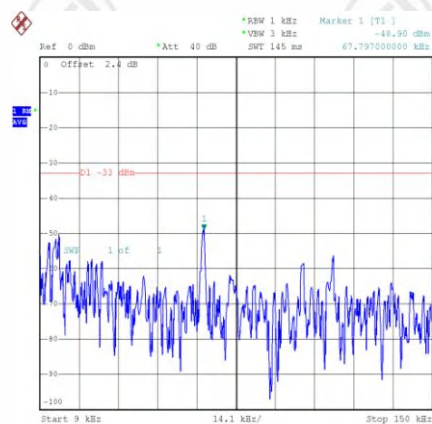
Band26(824-849)-3MHz-16QAM-26805-15RB#0 -1000~3000-PASS
