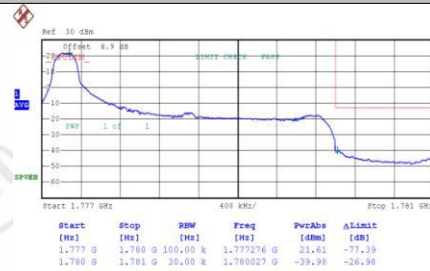
Band66-3MHz-QPSK-132657-1RB#14-PASS
