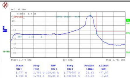
Band66-3MHz-QPSK-132657-15RB#0-PASS
