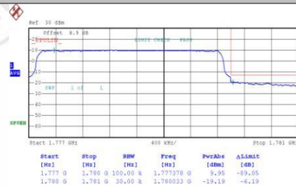
Band66-3MHz-16QAM-132657-1RB#0-PASS
