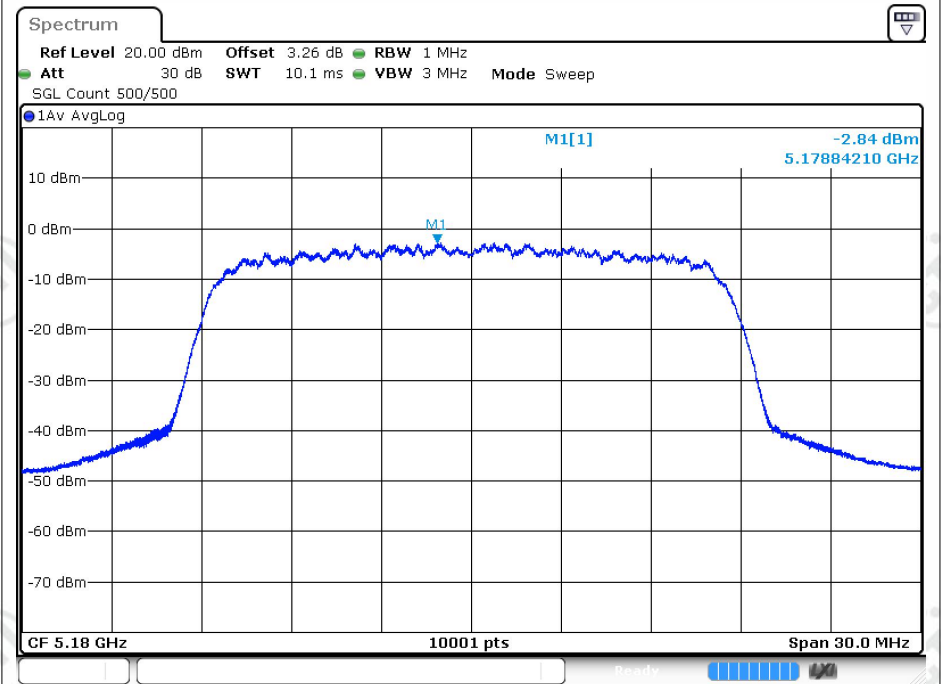
PSD NVNT 11A 5180MHz Ant1
