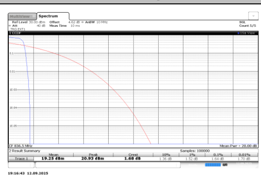
Band5-0.18-QPSK-20525-1@11-15kHz-PASS
