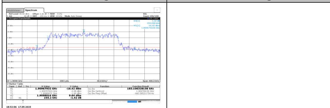
Band2-0.18-BPSK-19198-1@0-15kHz-PASS
