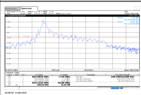
Band5-0.18-BPSK-20402-1@0-15kHz-PASS
