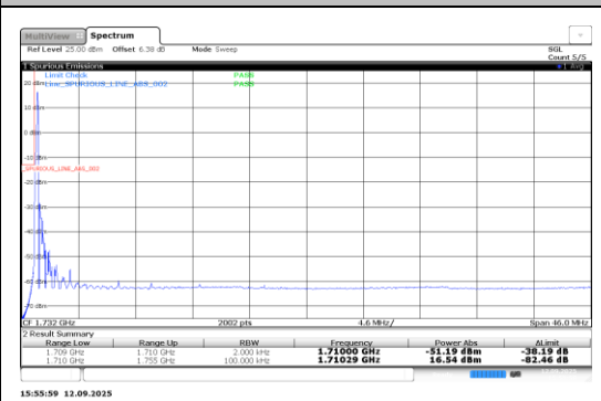
Band4-0.18-QPSK-19952-1@11-15kHz-PASS
