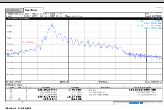
Band26-0.18-QPSK-26915-1@0-15kHz-PASS
