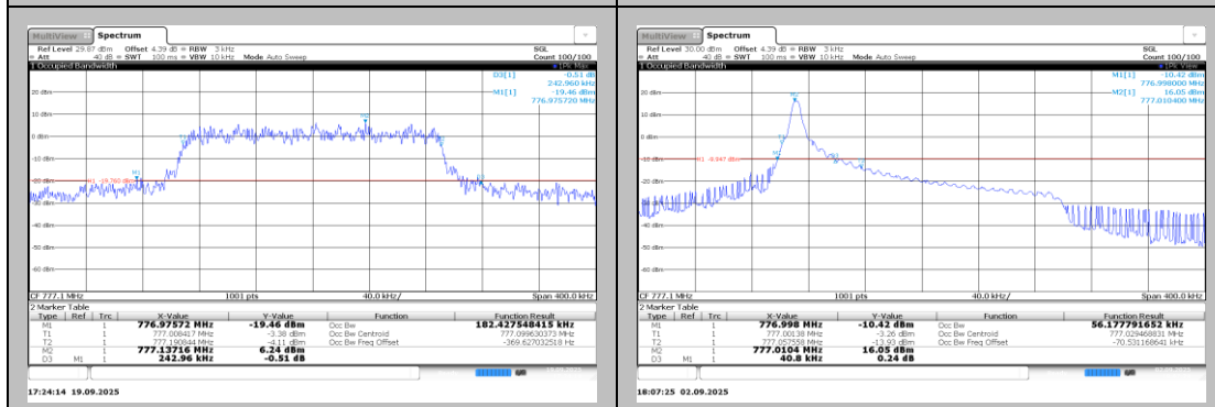
Band13-0.18-QPSK-23181-12@0-15kHz-PASS
