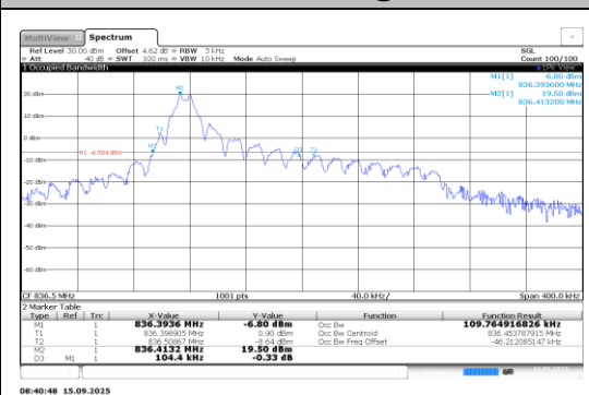
Band26-0.18-BPSK-26915-1@0-15kHz-PASS
