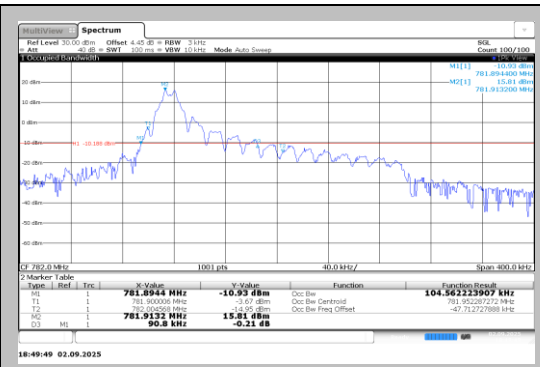
Band13-0.18-BPSK-23230-1@0-15kHz-PASS
