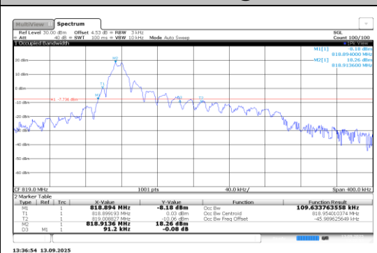
Band26-0.18-BPSK-26740-1@0-15kHz-PASS
