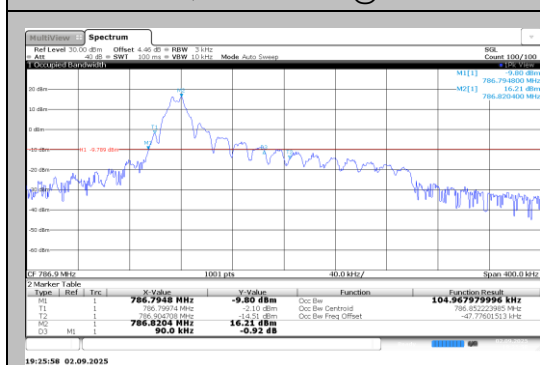
Band13-0.18-BPSK-23279-1@0-15kHz-PASS
