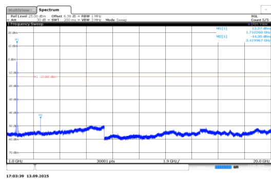
Band66-0.18-QPSK-131974-1@0-3.75kHz- 1000-20000-PASS
