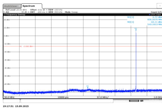
Band26-0.18-QPSK-26915-12@0-15kHz-30- 1000-PASS
