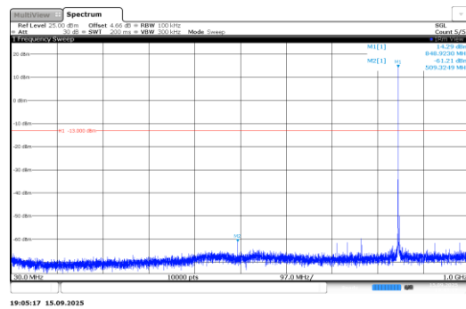
Band26-0.18-QPSK-27038-1@47-3.75kHz-30- 1000-PASS
