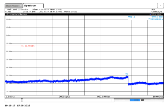
Band26-0.18-QPSK-27038-1@47-3.75kHz- 1000-10000-PASS
