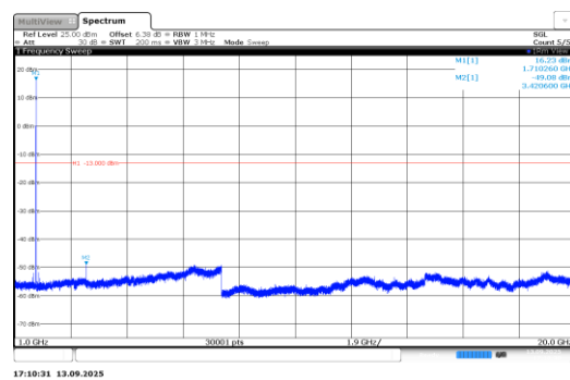
Band66-0.18-BPSK-131974-1@11-15kHz-1000- 20000-PASS
