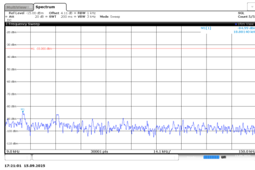
Band71-0.18-QPSK-133124-12@0-15kHz- 0.009-0.15-PASS
