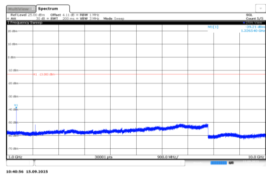
Band71-0.18-QPSK-133124-1@47-3.75kHz- 1000-10000-PASS
