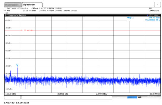
Band66-0.18-QPSK-132670-1@0-3.75kHz-0.15- 30-PASS
