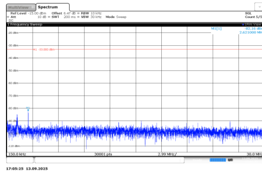
Band66-0.18-QPSK-132322-1@0-3.75kHz-0.15- 30-PASS
