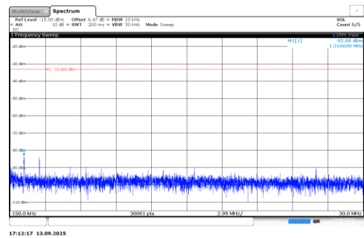
Band66-0.18-BPSK-132322-1@11-15kHz-0.15- 30-PASS
