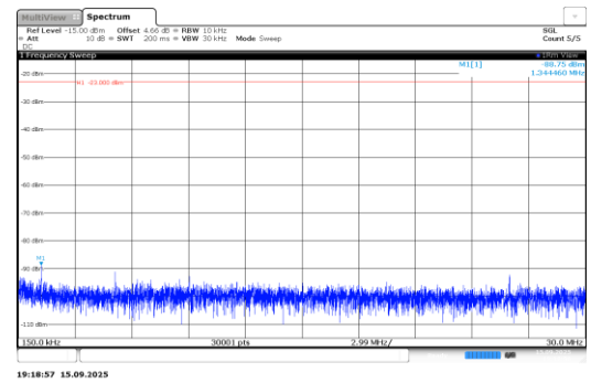
Band26-0.18-QPSK-27038-12@0-15kHz-0.15- 30-PASS
