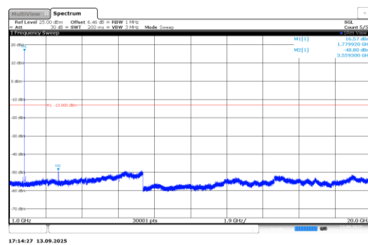
Band66-0.18-BPSK-132670-1@11-15kHz-1000- 20000-PASS
