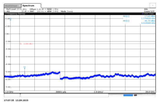
Band66-0.18-QPSK-132670-1@0-3.75kHz- 1000-20000-PASS
