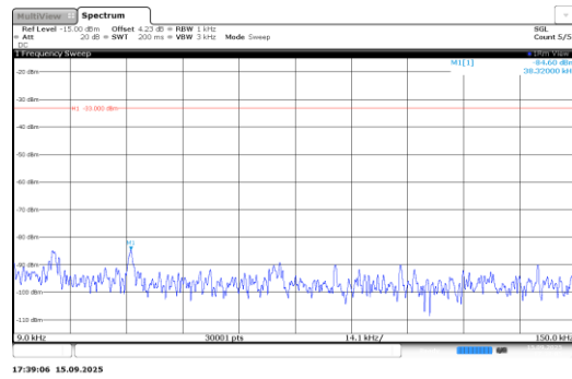
Band71-0.18-QPSK-133470-12@0-15kHz- 0.009-0.15-PASS
