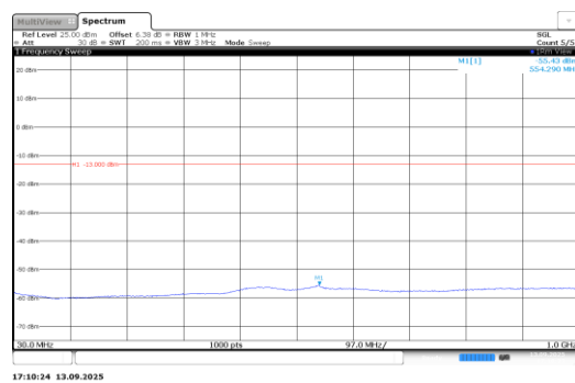
Band66-0.18-BPSK-131974-1@11-15kHz-30- 1000-PASS
