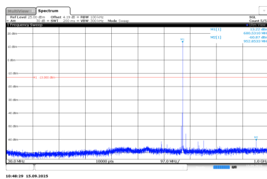
Band71-0.18-BPSK-133297-1@11-15kHz-30- 1000-PASS
