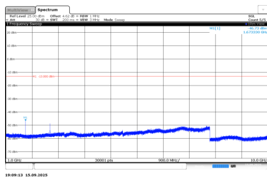
Band26-0.18-BPSK-26915-1@11-15kHz-1000-10000-PASS
