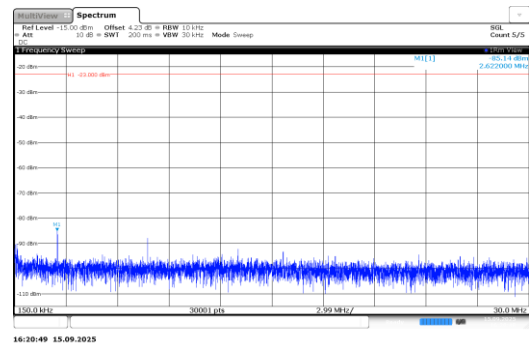
Band71-0.18-BPSK-133470-1@0-15kHz-0.15- 30-PASS
