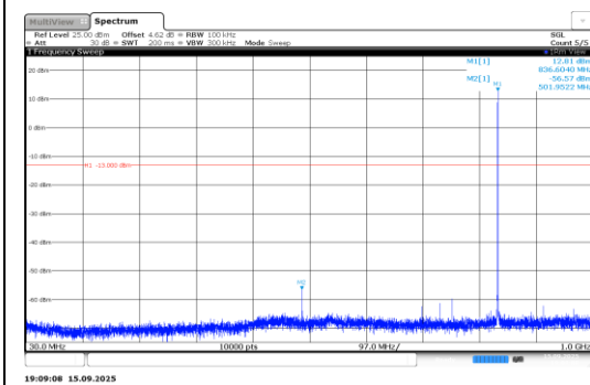
Band26-0.18-BPSK-26915-1@11-15kHz-30-1000-PASS
