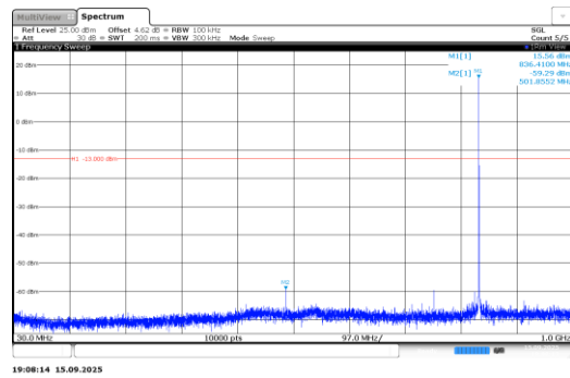
Band26-0.18-BPSK-26915-1@0-15kHz-30-1000-PASS
