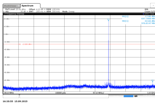
Band71-0.18-BPSK-133470-1@0-15kHz-30- 1000-PASS
