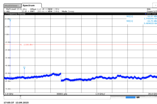
Band66-0.18-QPSK-132322-1@0-3.75kHz-0.15- 30-PASS
