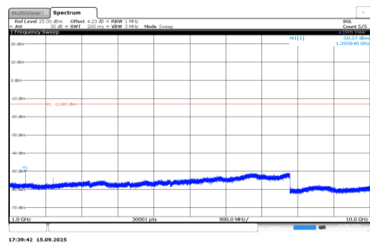
Band71-0.18-QPSK-133470-12@0-15kHz-0.15- 30-PASS
