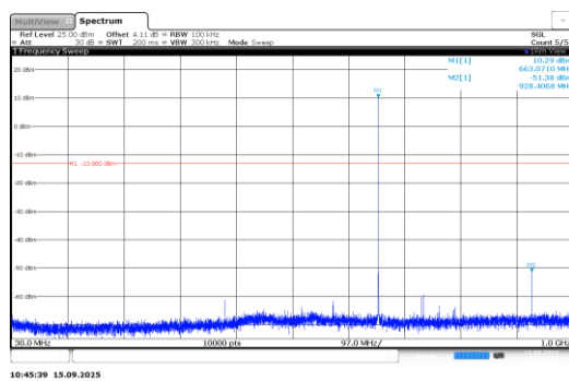
Band71-0.18-BPSK-133124-1@0-15kHz-30- 1000-PASS
