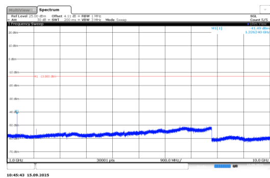
Band71-0.18-BPSK-133124-1@0-15kHz-1000- 10000-PASS
