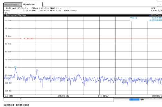
Band66-0.18-QPSK-132322-1@0-3.75kHz- 0.009-0.15-PASS
