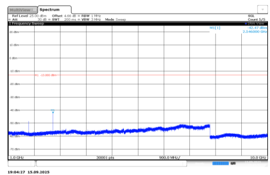
Band26-0.18-QPSK-27038-1@0-3.75kHz-1000- 10000-PASS
