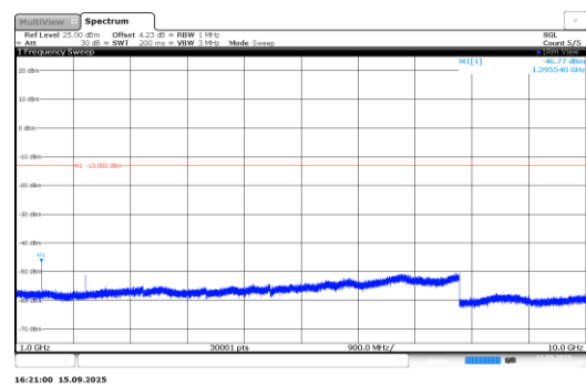
Band71-0.18-BPSK-133470-1@0-15kHz-1000- 10000-PASS
