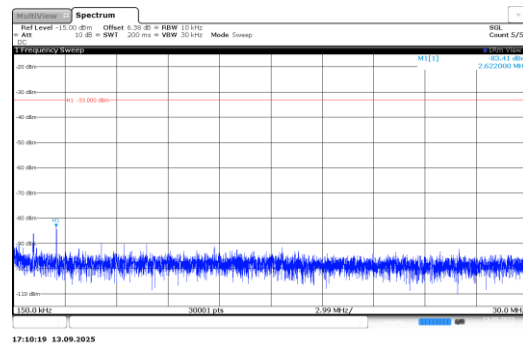
Band66-0.18-BPSK-131974-1@11-15kHz-0.15- 30-PASS
