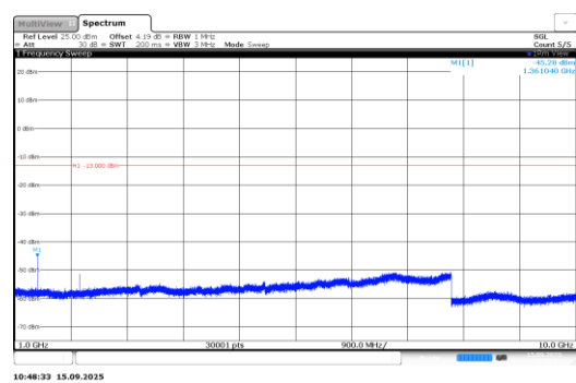
Band71-0.18-BPSK-133297-1@11-15kHz-1000- 10000-PASS
