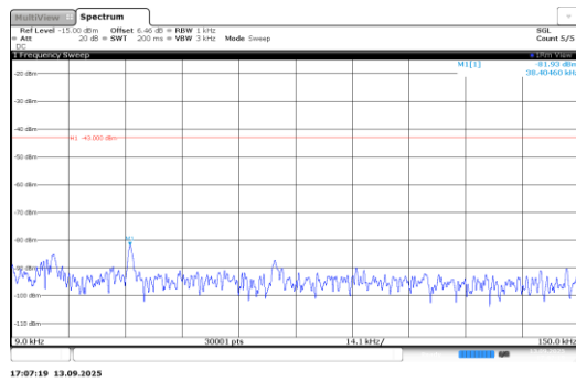
Band66-0.18-QPSK-132670-1@0-3.75kHz- 0.009-0.15-PASS
