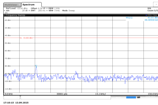
Band66-0.18-BPSK-131974-1@11-15kHz-0.009- 0.15-PASS
