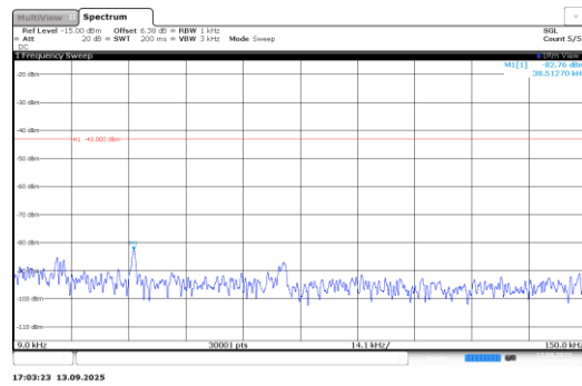
Band66-0.18-QPSK-131974-1@0-3.75kHz- 0.009-0.15-PASS
