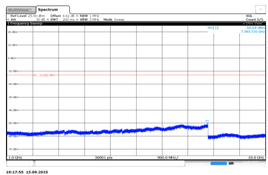
Band26-0.18-QPSK-26915-12@0-15kHz-1000- 10000-PASS
