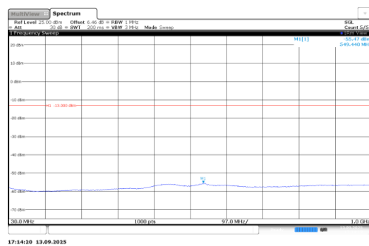
Band66-0.18-BPSK-132670-1@11-15kHz-30- 1000-PASS
