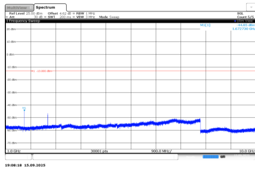
Band26-0.18-BPSK-26915-1@0-15kHz-1000-10000-PASS
