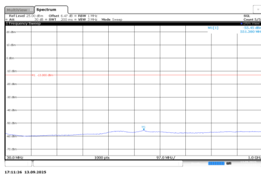
Band66-0.18-BPSK-132322-1@0-15kHz-30- 1000-PASS
