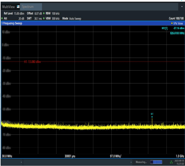
DH5-Ant1-2480-30~1000-PASS
