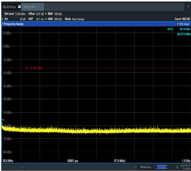
2DH5-Ant1-2480-30~1000-PASS
