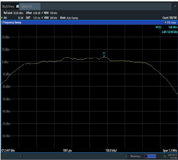
2DH5-Ant1-2441-0~Reference-PASS
