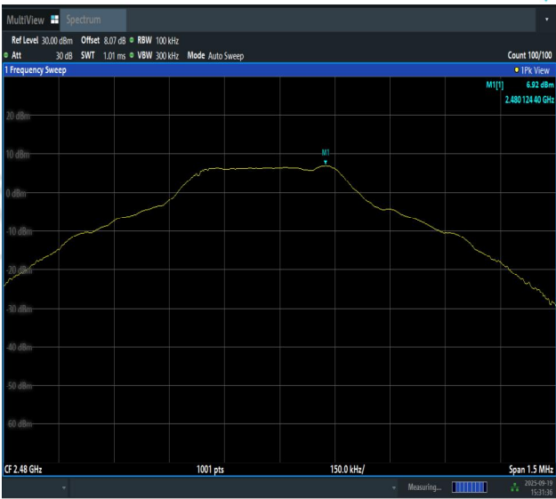
DH5-Ant1-2480-0~Reference-PASS
