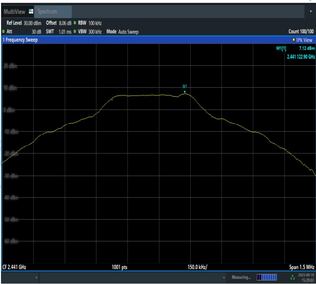
DH5-Ant1-2441-0~Reference-PASS
