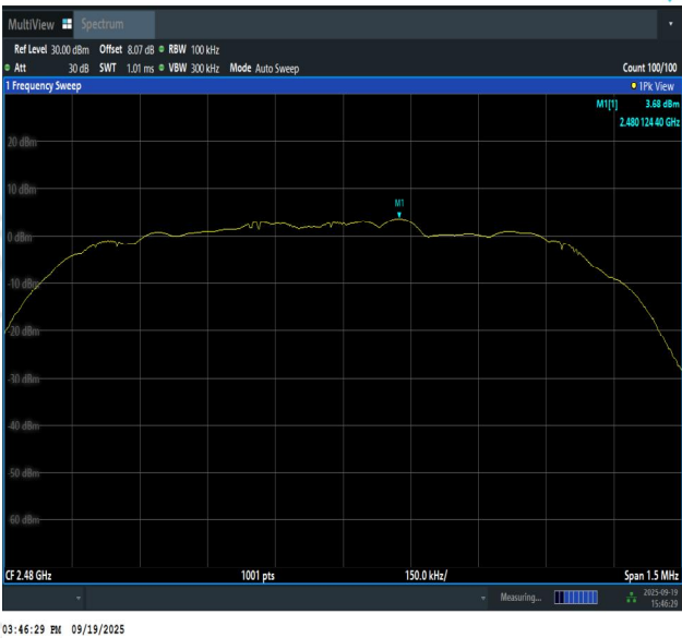
3DH5-Ant1-2480-0~Reference-PASS
