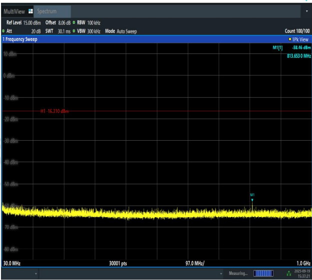
2DH5-Ant1-2441-30~1000-PASS
