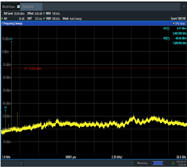
DH5-Ant1-2402-1000~26500-PASS
