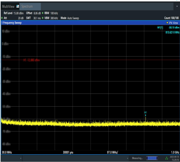
DH5-Ant1-2441-30~1000-PASS
