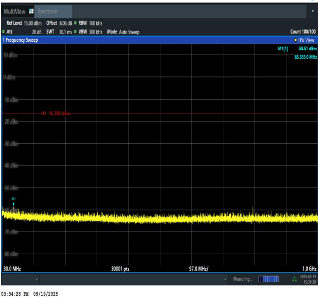
2DH5-Ant1-2402-30~1000-PASS
