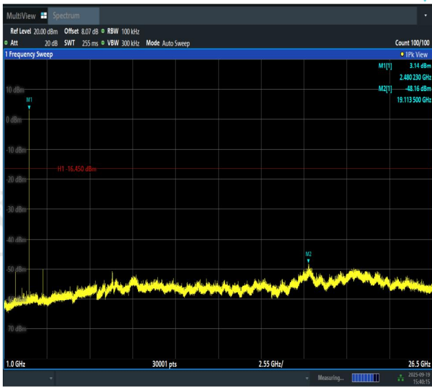
2DH5-Ant1-2480-1000~26500-PASS
