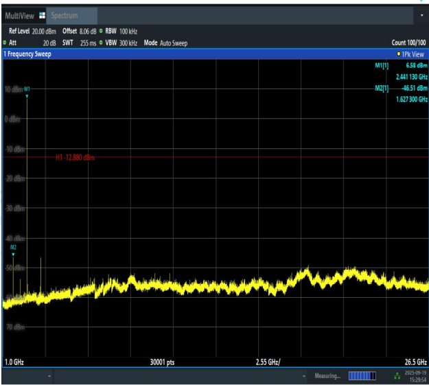
DH5-Ant1-2441-1000~26500-PASS
