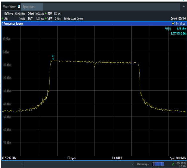
11AX40SISO-Ant1-5795-PASS
