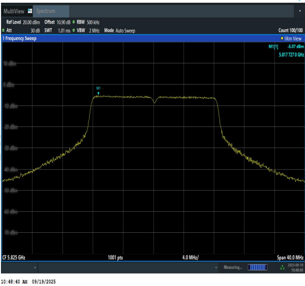
11A-Ant1-5825-PASS
