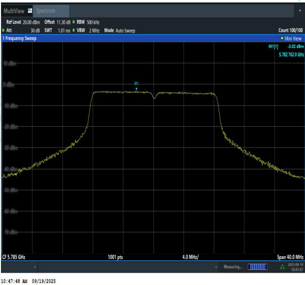
11A-Ant1-5785-PASS
