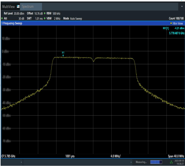
11AC20SISO-Ant1-5785-PASS
