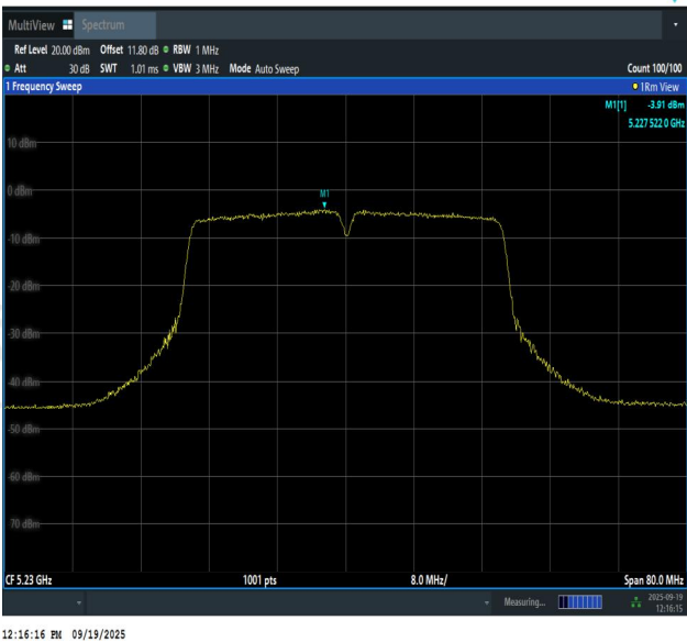
11AC40SISO-Ant1-5230-PASS
