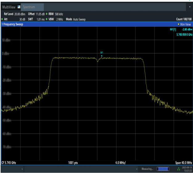
11AX20SISO-Ant1-5745-PASS
