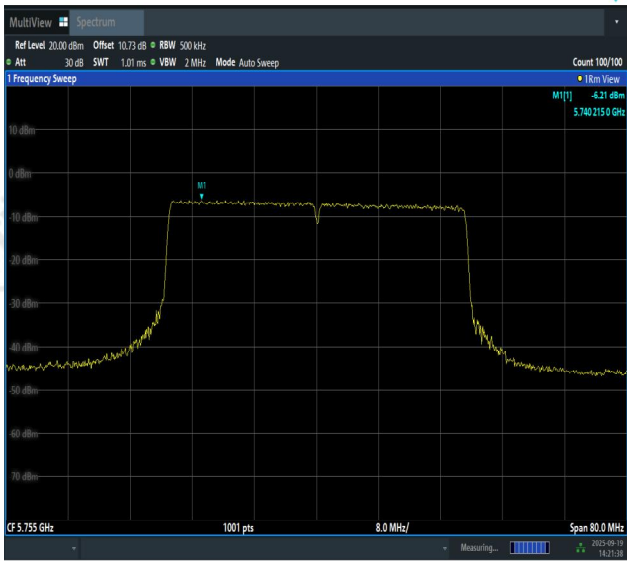
11AX40SISO-Ant1-5755-PASS
