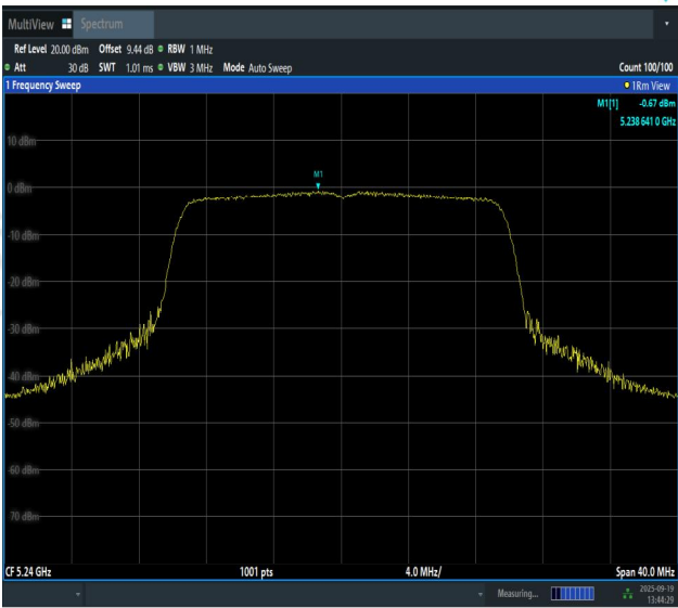
11AX20SISO-Ant1-5240-PASS
