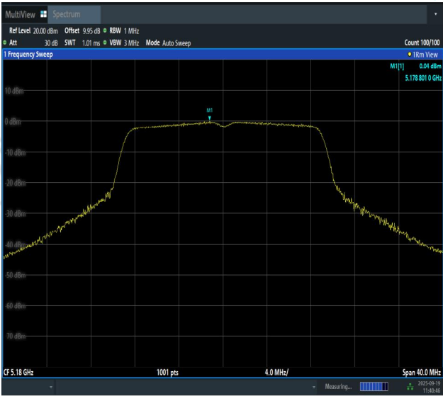
11AC20SISO-Ant1-5180-PASS
