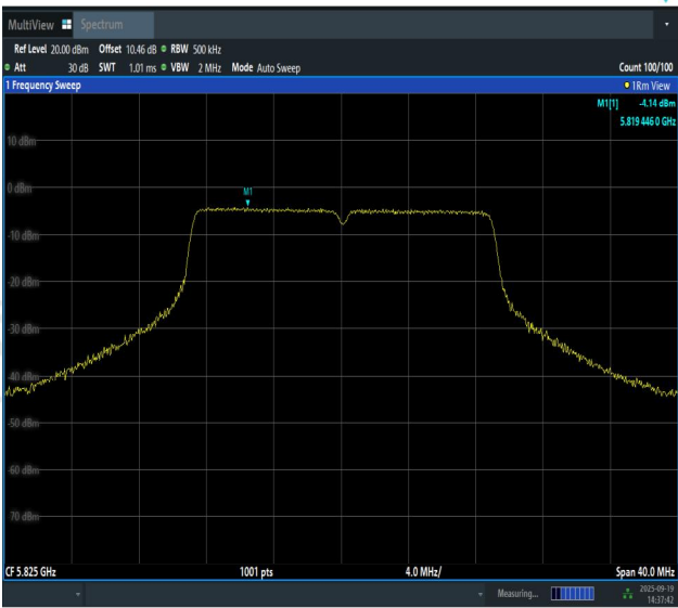
11AC20SISO-Ant1-5825-PASS
