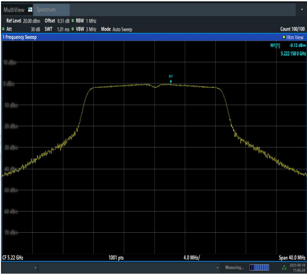
11AC20SISO-Ant1-5220-PASS
