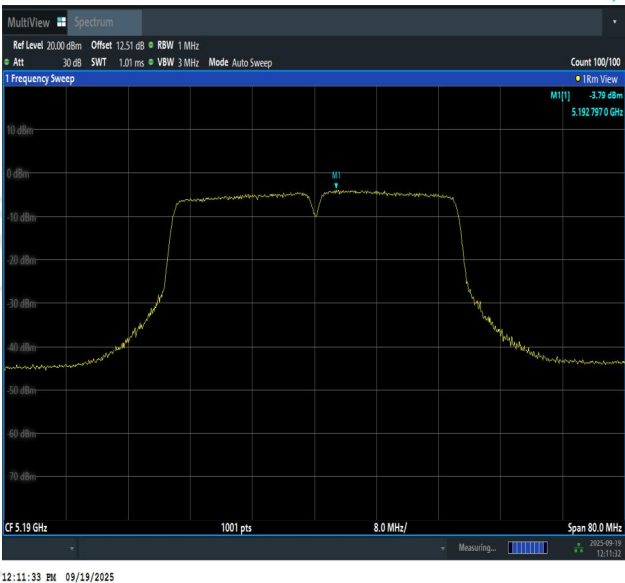
11AC40SISO-Ant1-5190-PASS
