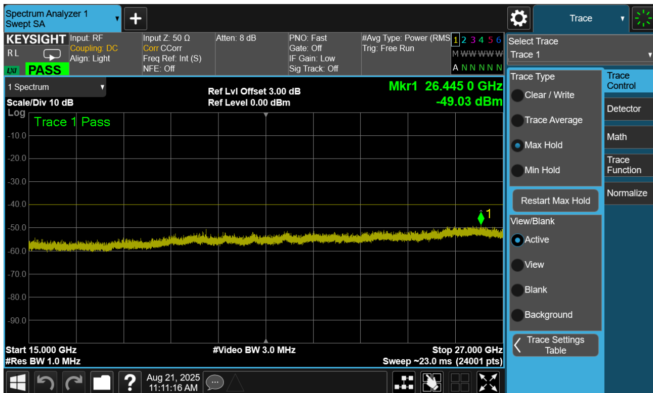
Plot 7.33. Conducted Spurious Plot (20MHz TM1.1, Mid Channel)
