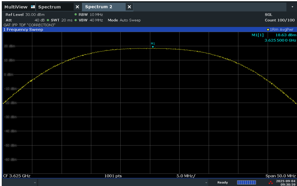
Plot 7.16. Power/10MHz Plot (20MHz TM3.1a – Mid Channel)
