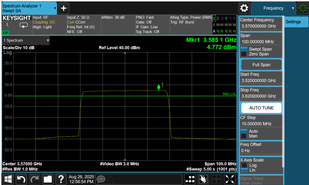
Plot 7.17. Power Spectral Density Plot (40MHz TM1.1 – Low Channel)
