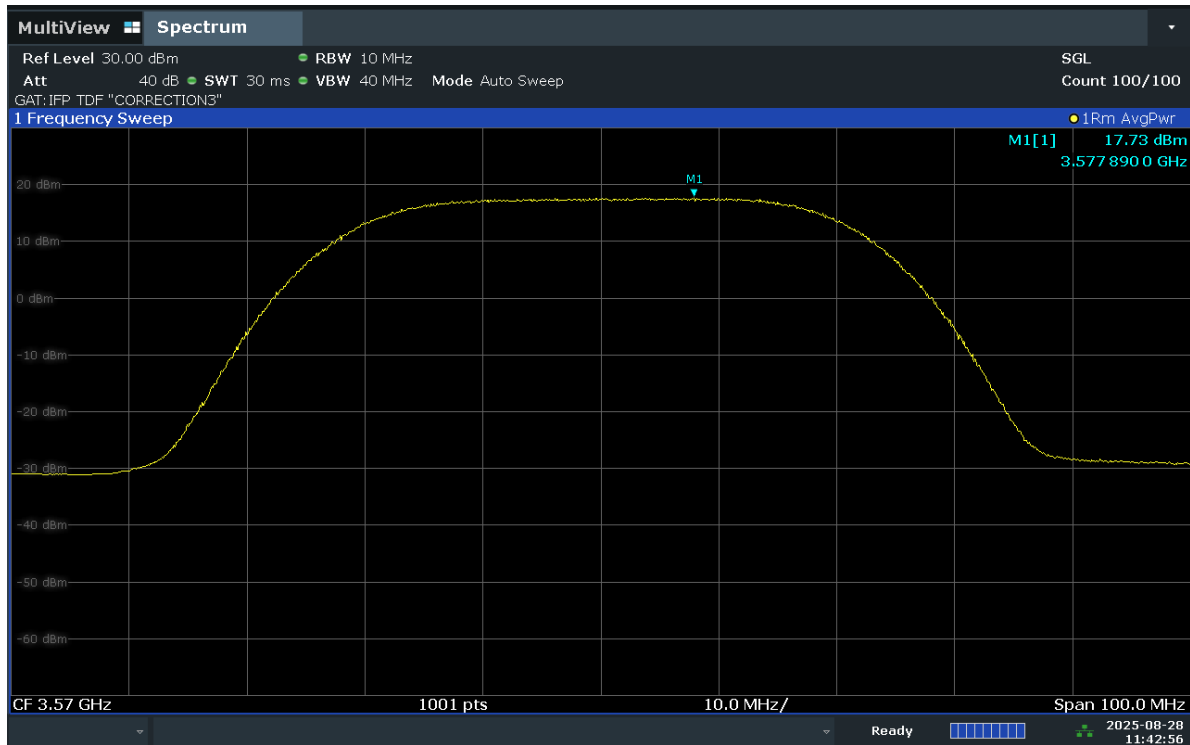
Plot 7.12. Power/10MHz Plot (40MHz TM3.1a – Low Channel)
