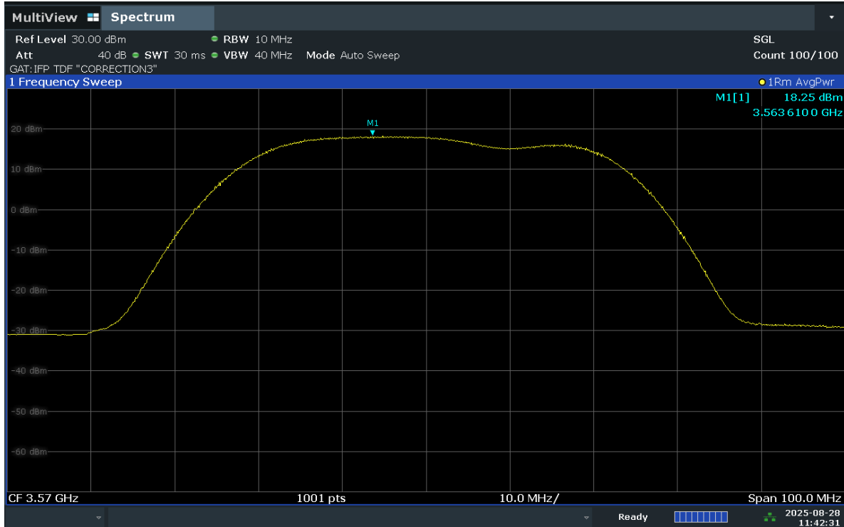
Plot 7.10. Power/10MHz Plot (40MHz TM1.2 – Low Channel)
