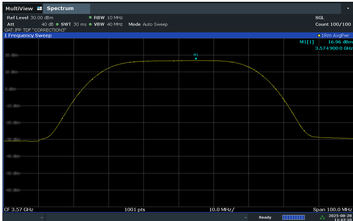
Plot 7.9. Power/10MHz Plot (40MHz TM1.1 – Low Channel)
