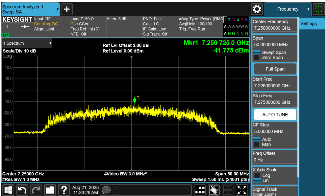
Plot 7.32. Conducted Spurious Plot (20MHz TM1.1, Mid Channel)
