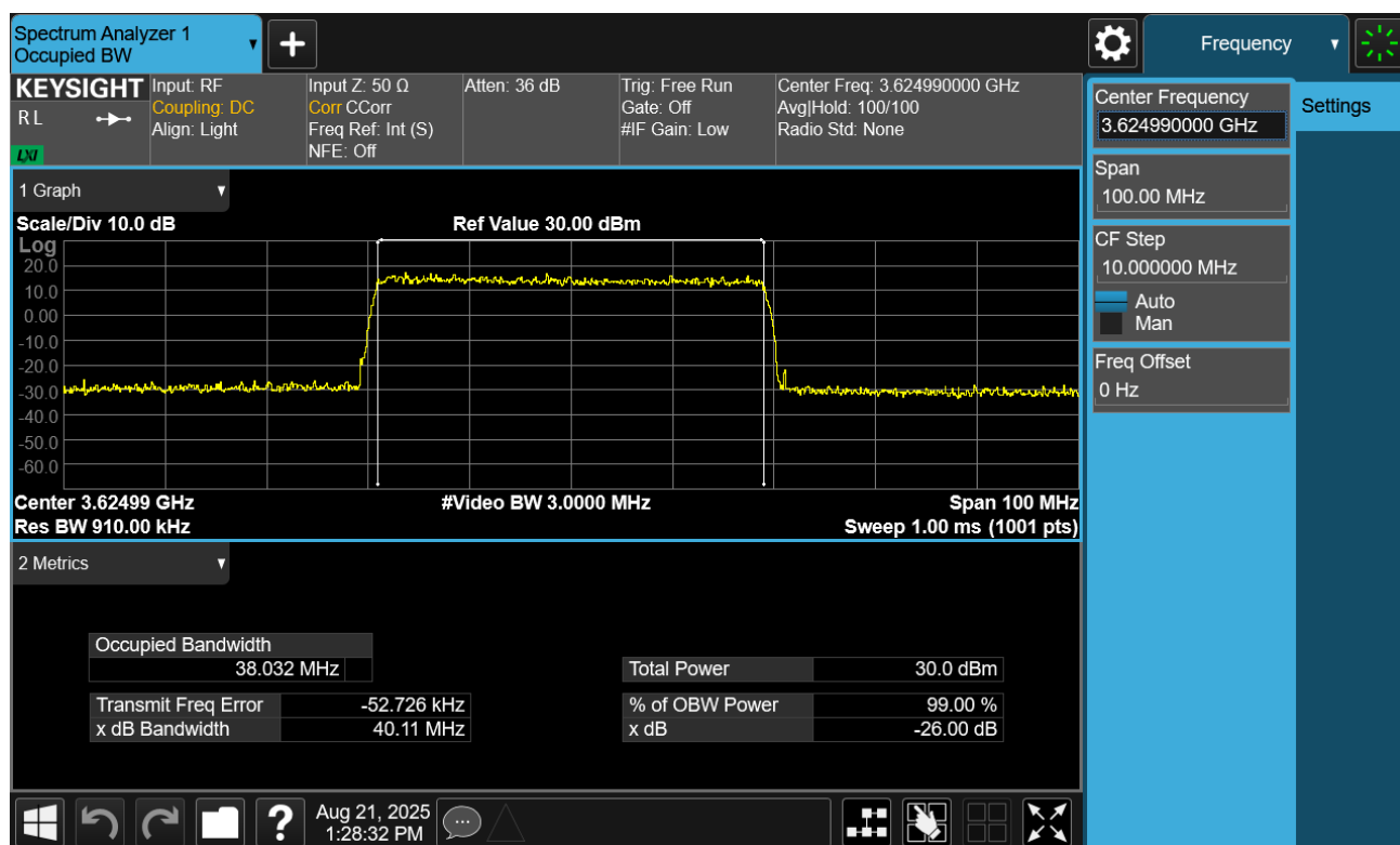
Plot 7.1. Occupied Bandwidth Plot (40MHz TM1.1)
