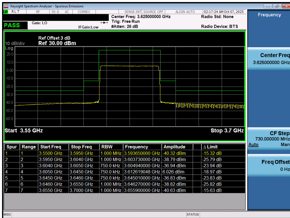
Plot 7.40. Conducted Band Edge Plot (40MHz, TM1.1, Mid Channel)
