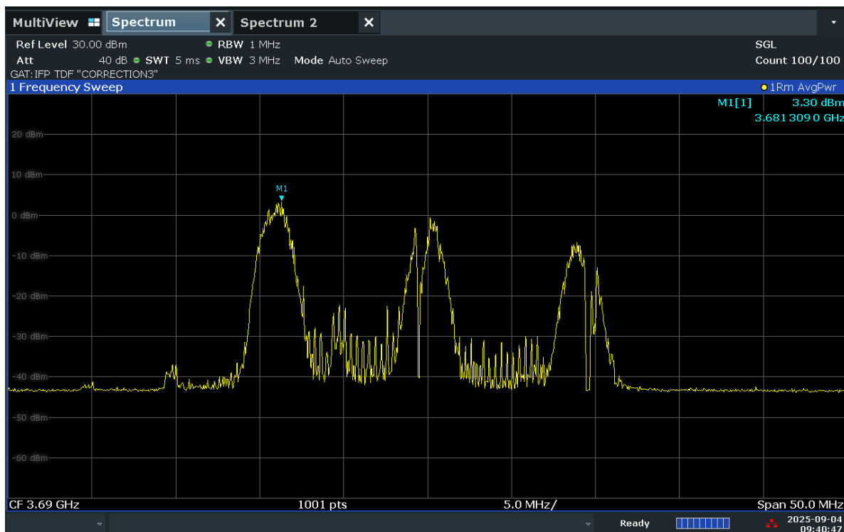
Plot 7.23. Power Spectral Density Plot (20MHz TM2a – High Channel)
