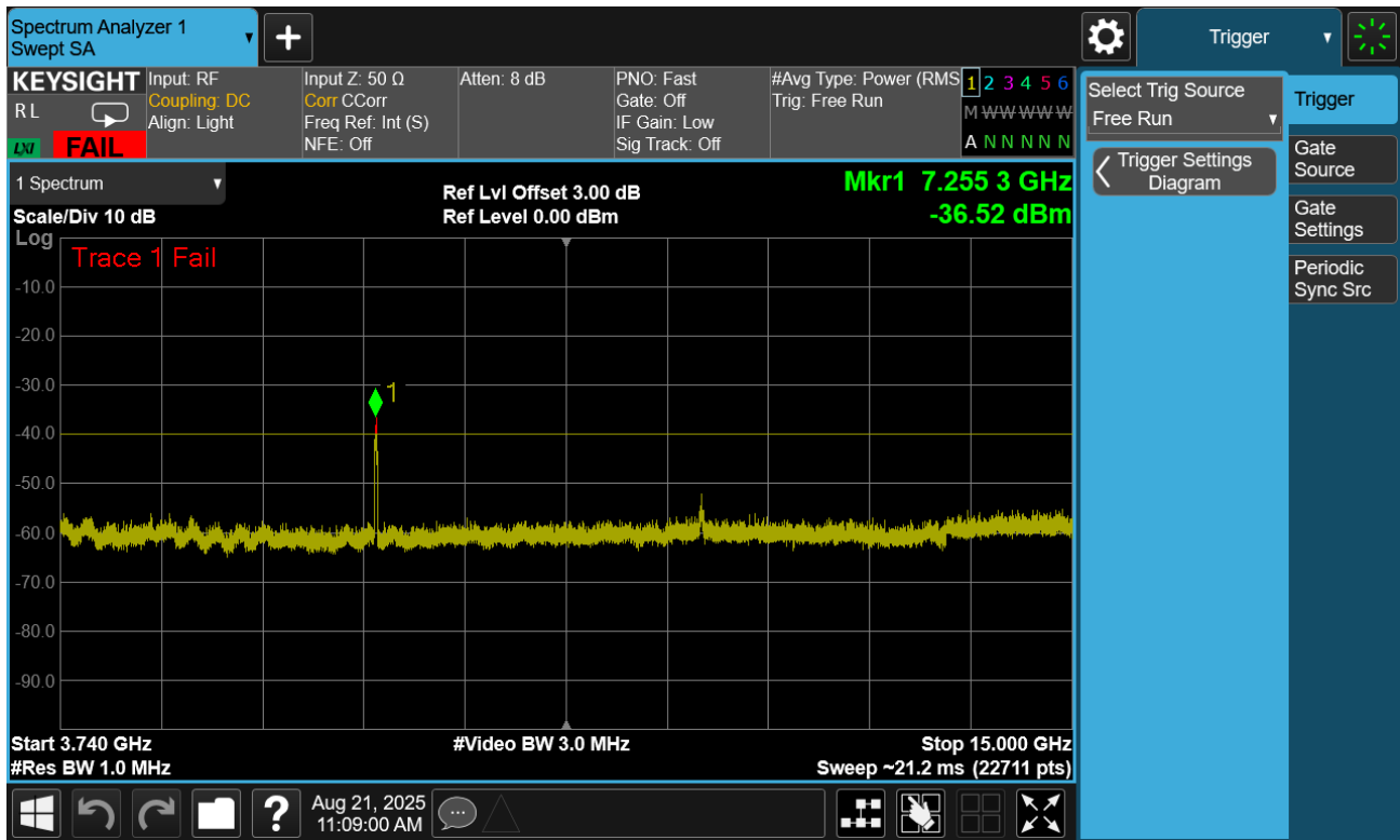
Plot 7.31. Conducted Spurious Plot (20MHz TM1.1, Mid Channel)
