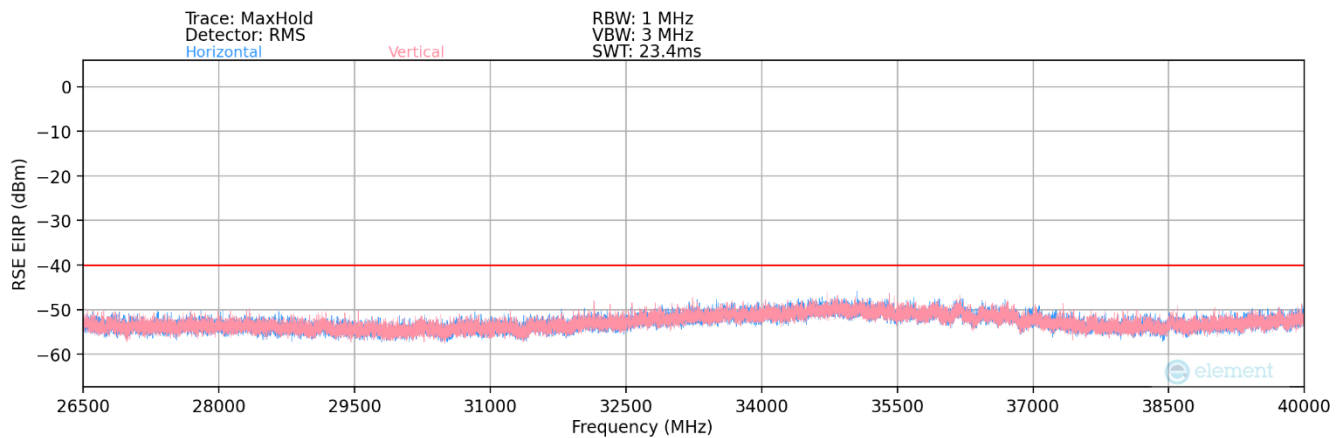
Plot 7.56. Radiated Spurious Plot 26.5-40GHz – Mid Channel
