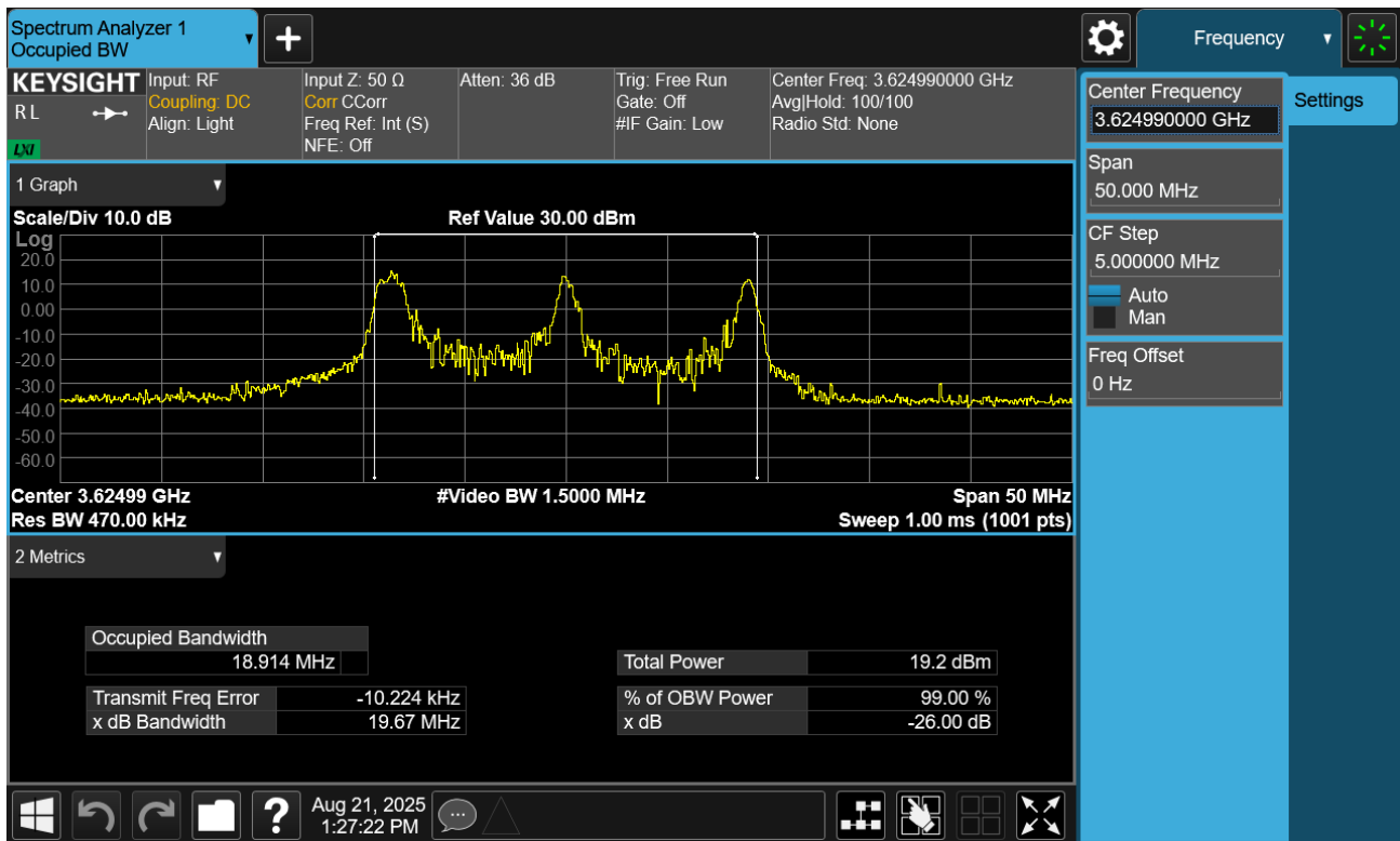
Plot 7.7. Occupied Bandwidth Plot (20MHz TM2a)
