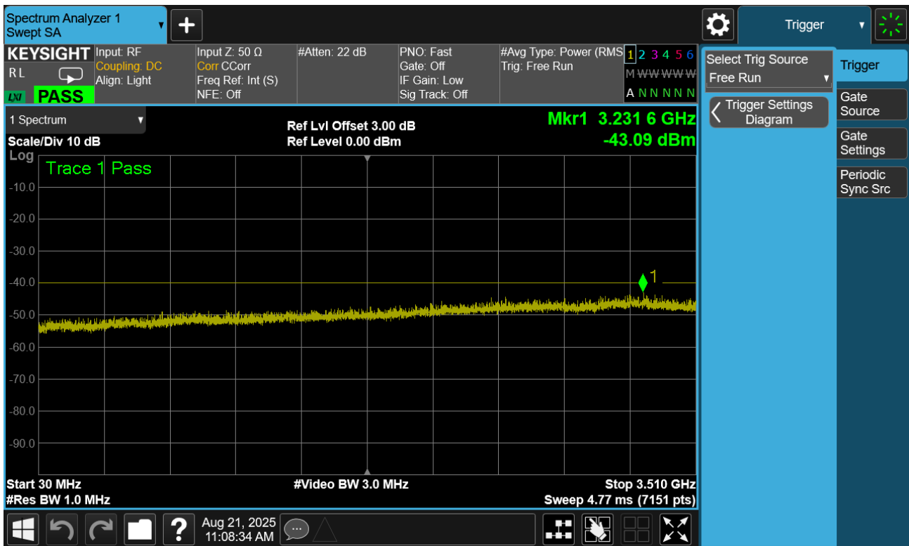
Plot 7.30. Conducted Spurious Plot (20MHz TM1.1, Mid Channel)
