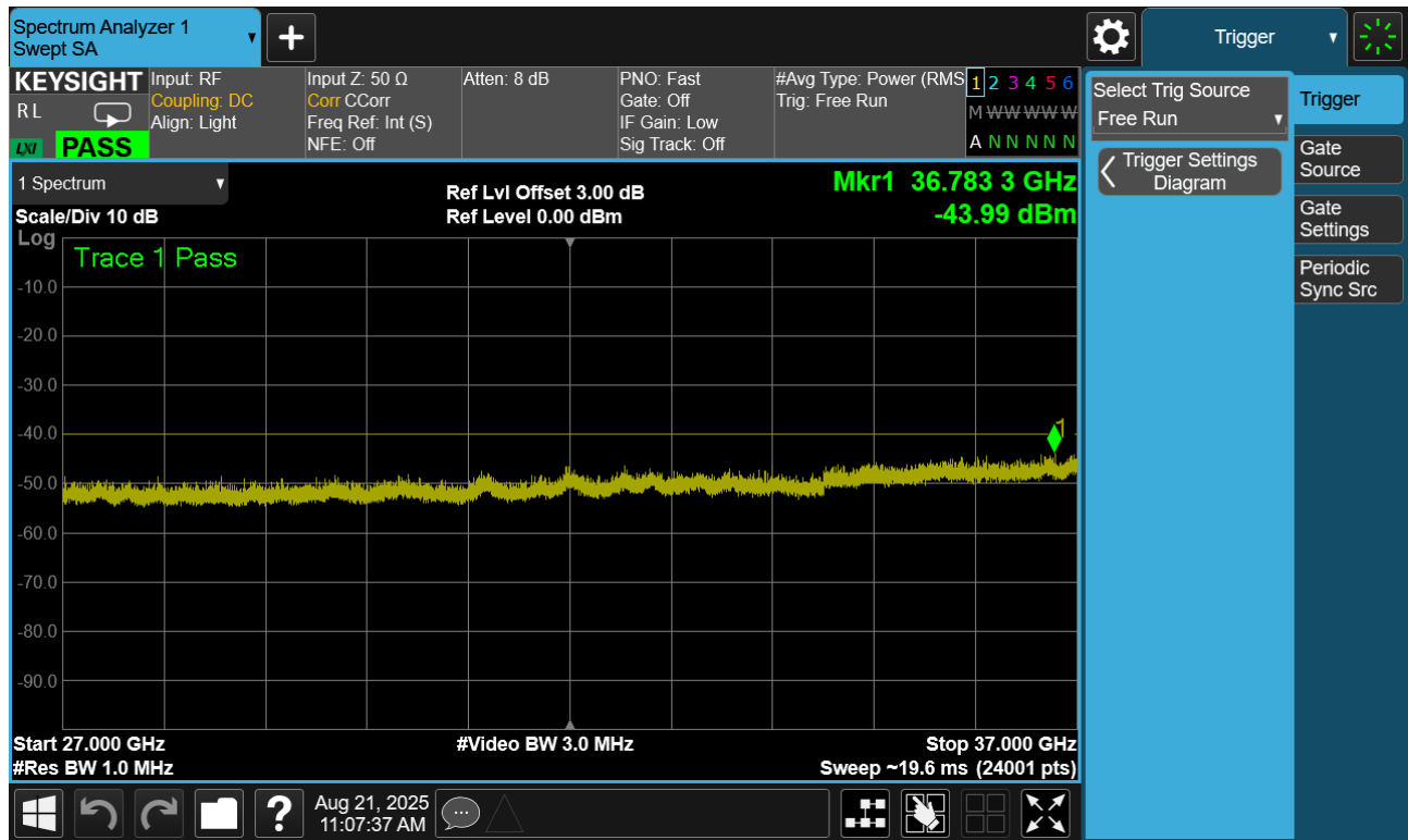
Plot 7.29. Conducted Spurious Plot (20MHz TM1.1, Low Channel)
