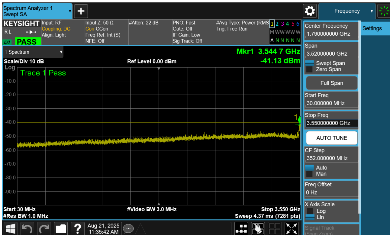
Plot 7.35. Conducted Spurious Plot (20MHz TM1.1, High Channel)
