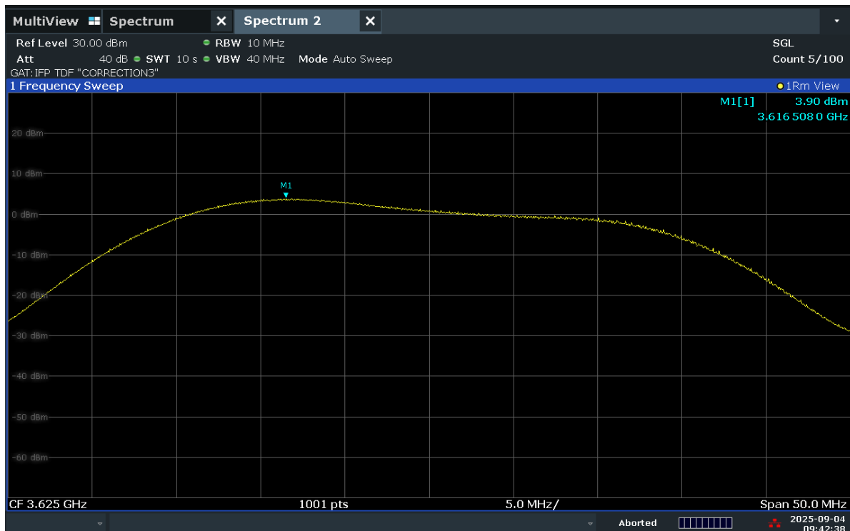
Plot 7.15. Power/10MHz Plot (20MHz TM2a – Mid Channel)
