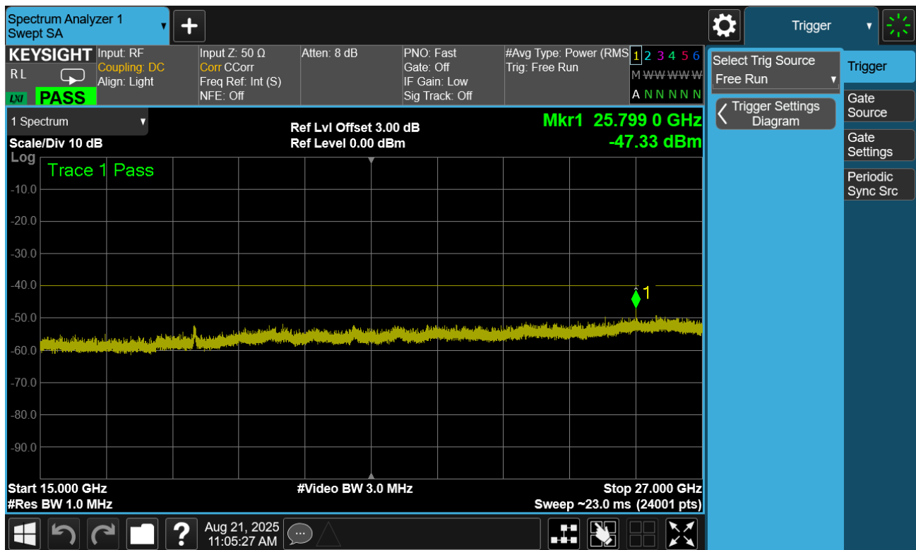
Plot 7.28. Conducted Spurious Plot (20MHz TM1.1, Low Channel)
