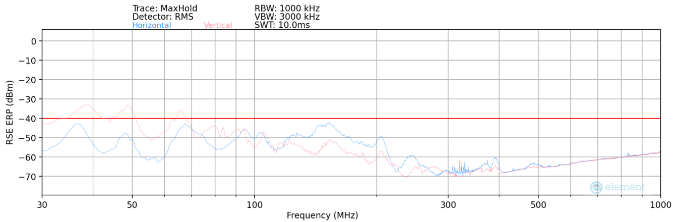
Plot 7.53. Radiated Spurious Plot 30MHz-1GHz – Mid Channel
