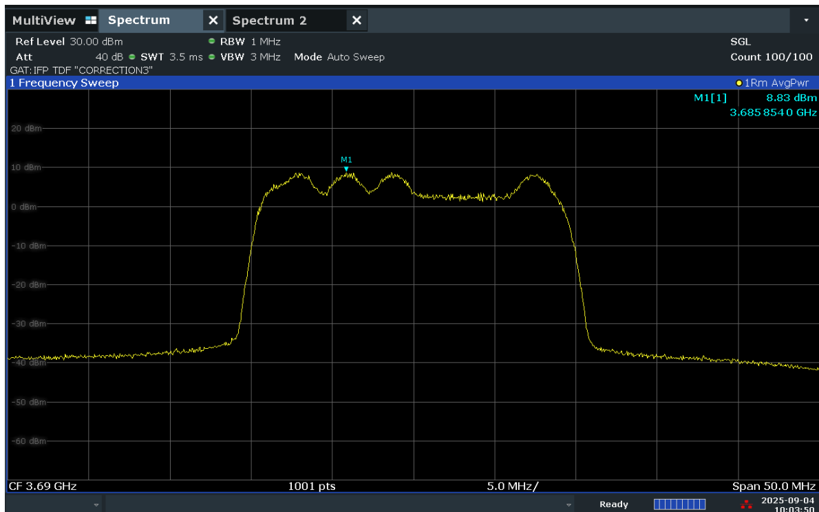
Plot 7.22. Power Spectral Density Plot (20MHz TM1.2 - High Channel)
