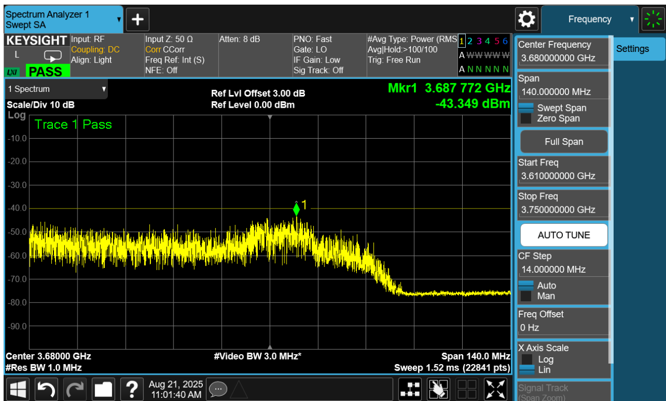
Plot 7.26. Conducted Spurious Plot (20MHz TM1.1, Low Channel)
