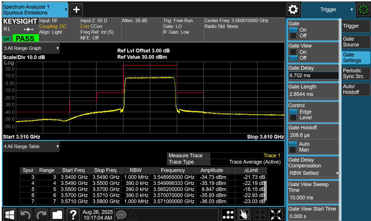
Plot 7.42. Conducted Band Edge Plot (20MHz, TM1.1, Low Channel)
