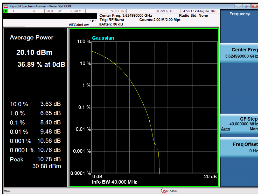
Plot 7.52. Peak-Average Ratio Plot (40MHz TM3.1a)
