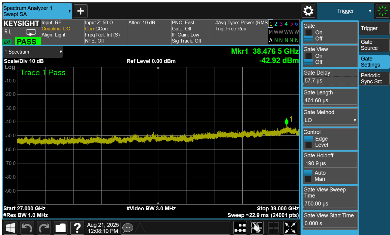
Plot 7.38. Conducted Spurious Plot (20MHz TM1.1, High Channel)
