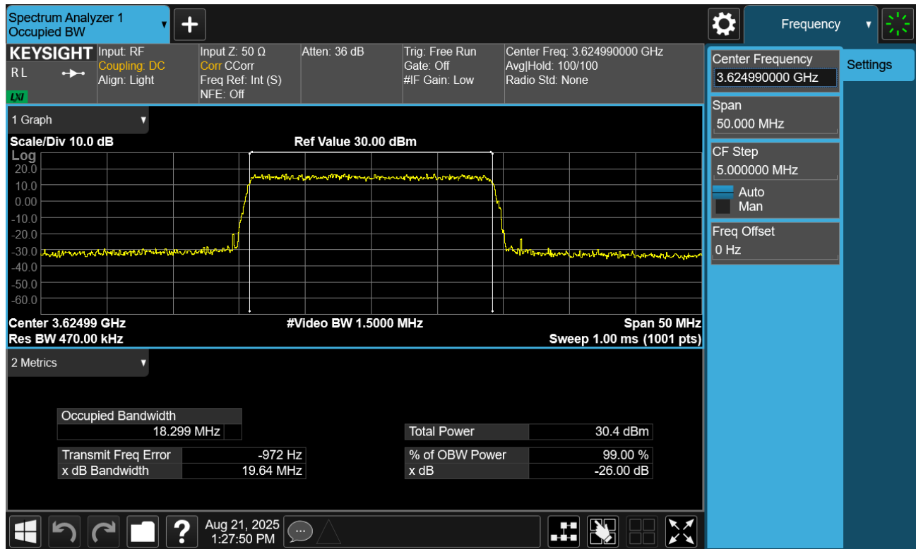
Plot 7.8. Occupied Bandwidth Plot (20MHz TM3.1a)
