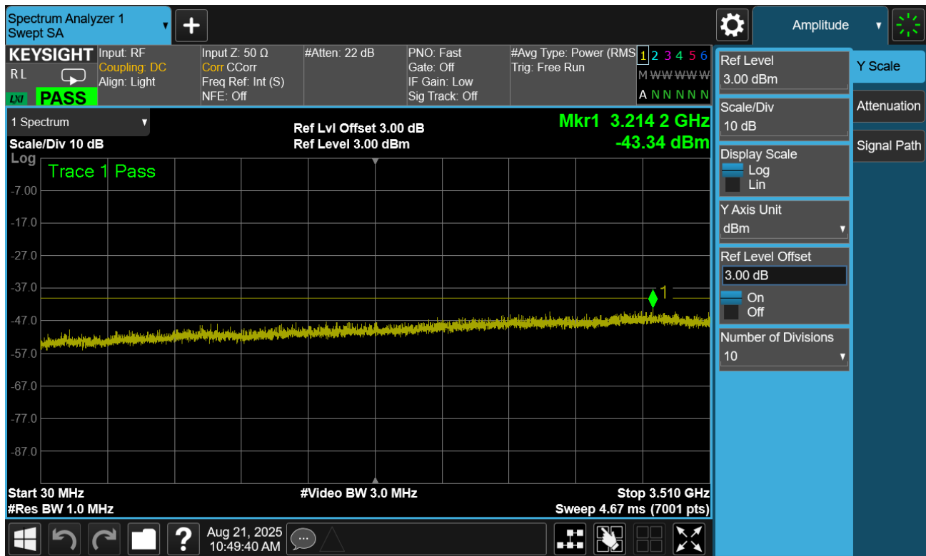
Plot 7.25. Conducted Spurious Plot (20MHz TM1.1, Low Channel)
