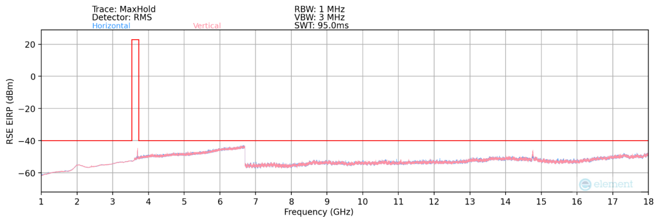
Plot 7.54. Radiated Spurious Plot 1-18GHz – Mid Channel
