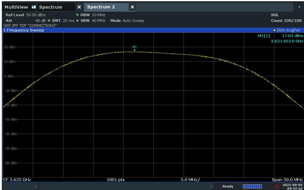
Plot 7.14. Power/10MHz Plot (20MHz TM1.2 – Mid Channel)
