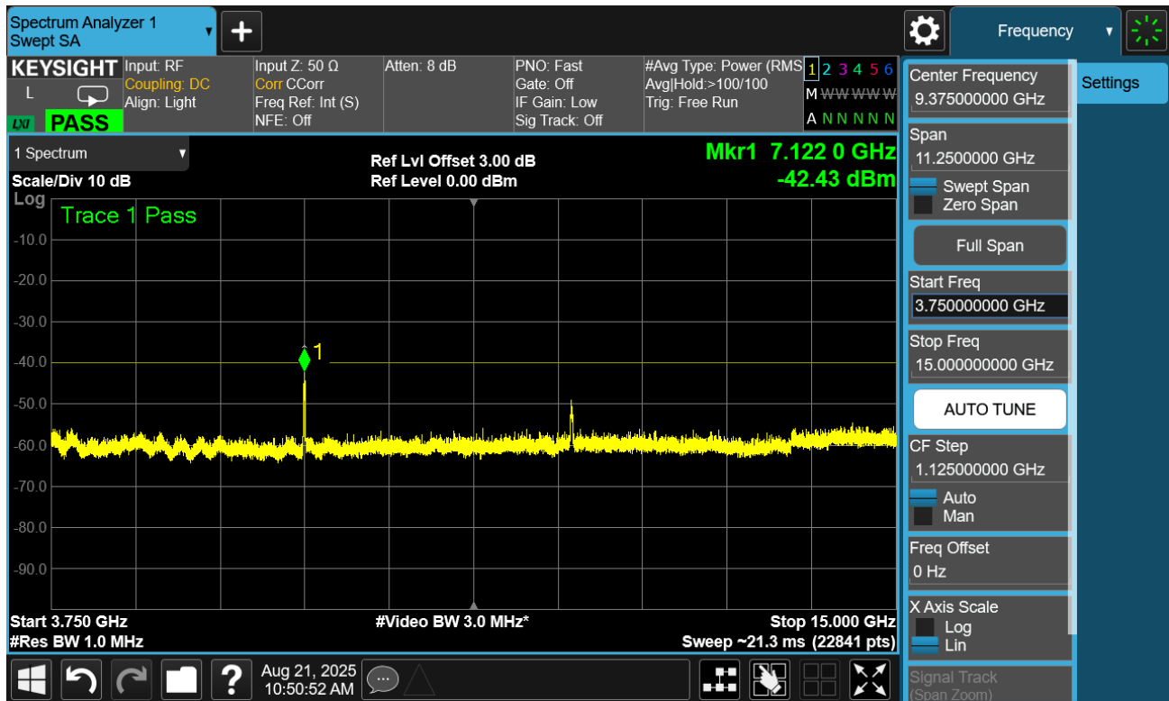
Plot 7.27. Conducted Spurious Plot (20MHz TM1.1, Low Channel)
