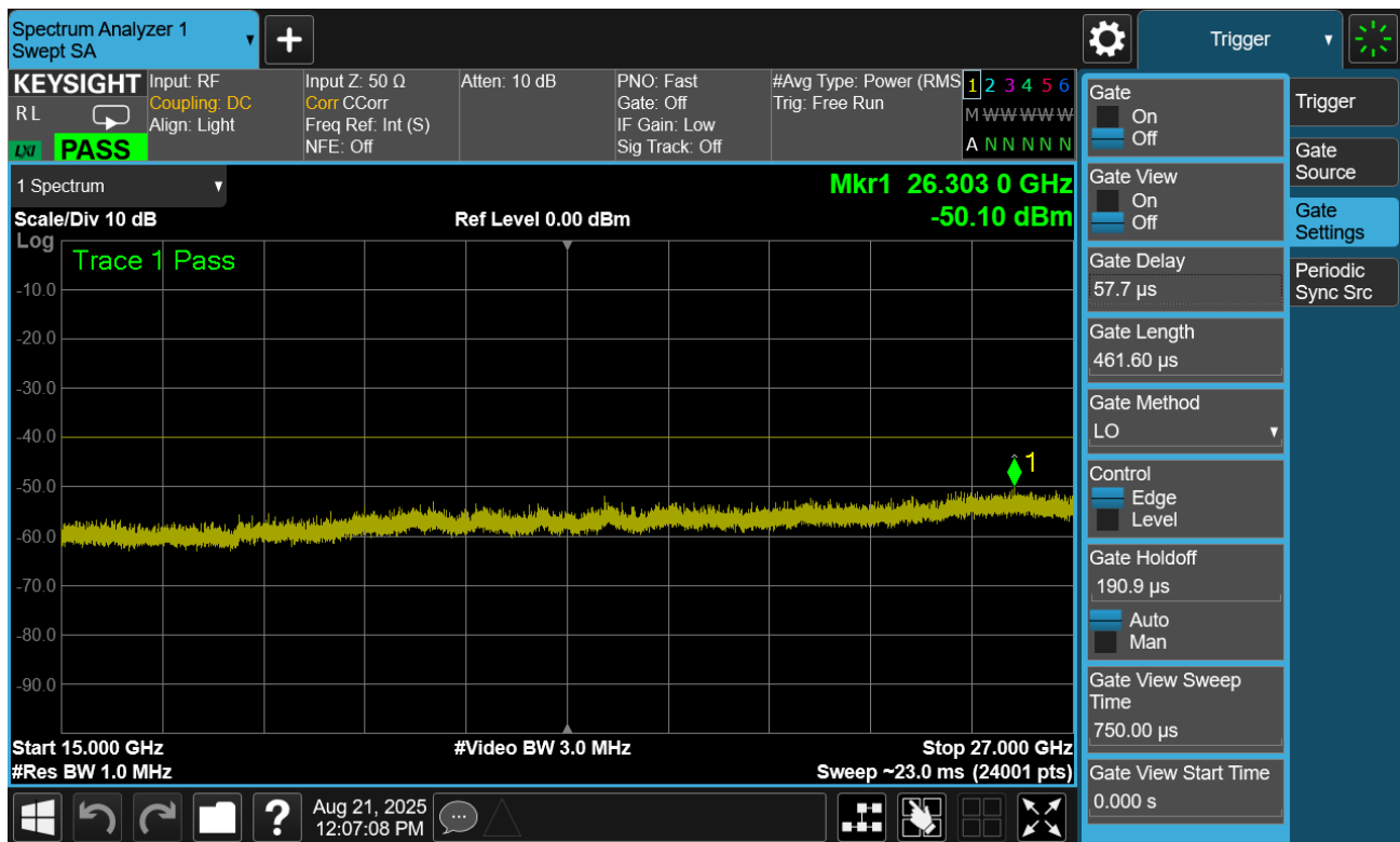
Plot 7.37. Conducted Spurious Plot (20MHz TM1.1, High Channel)
