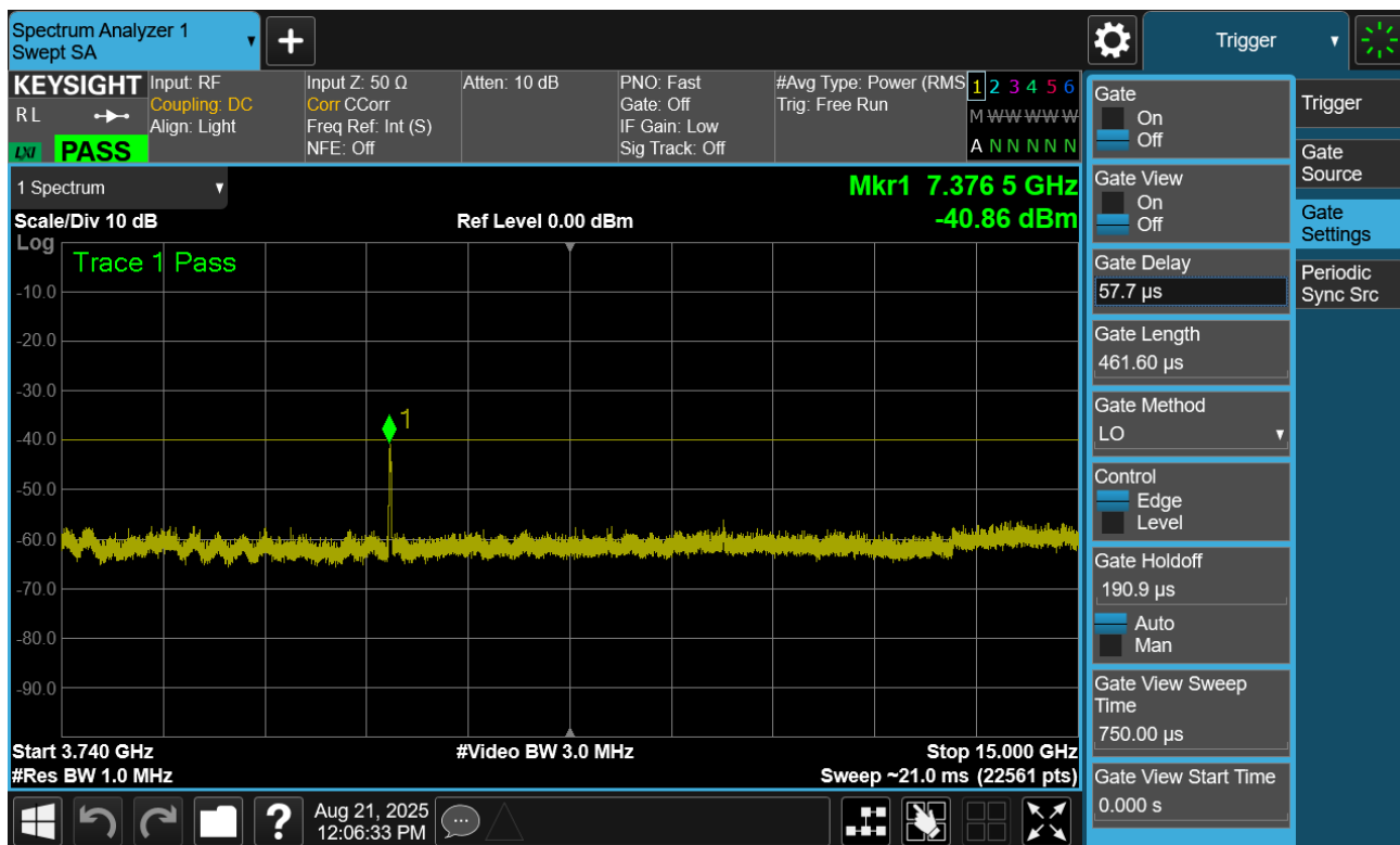
Plot 7.36. Conducted Spurious Plot (20MHz TM1.1, High Channel)
