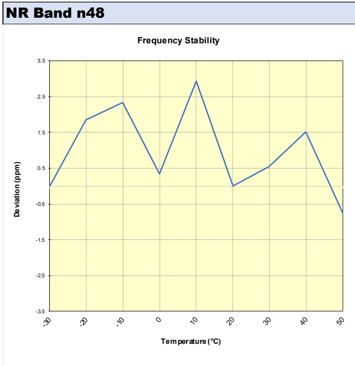
Plot 7.57. Frequency Stability Chart
