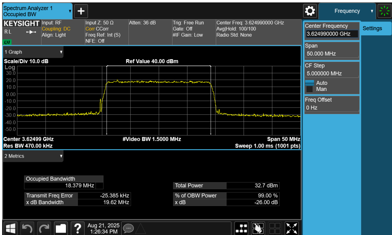
Plot 7.5. Occupied Bandwidth Plot (20MHz TM1.1)
