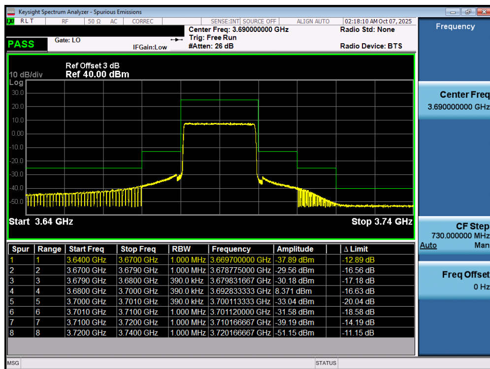
Plot 7.44. Conducted Band Edge Plot (20MHz, TM1.1, High Channel)
