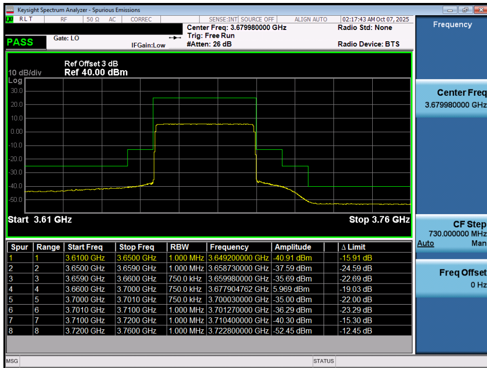
Plot 7.41. Conducted Band Edge Plot (40MHz, TM1.1, High Channel)
