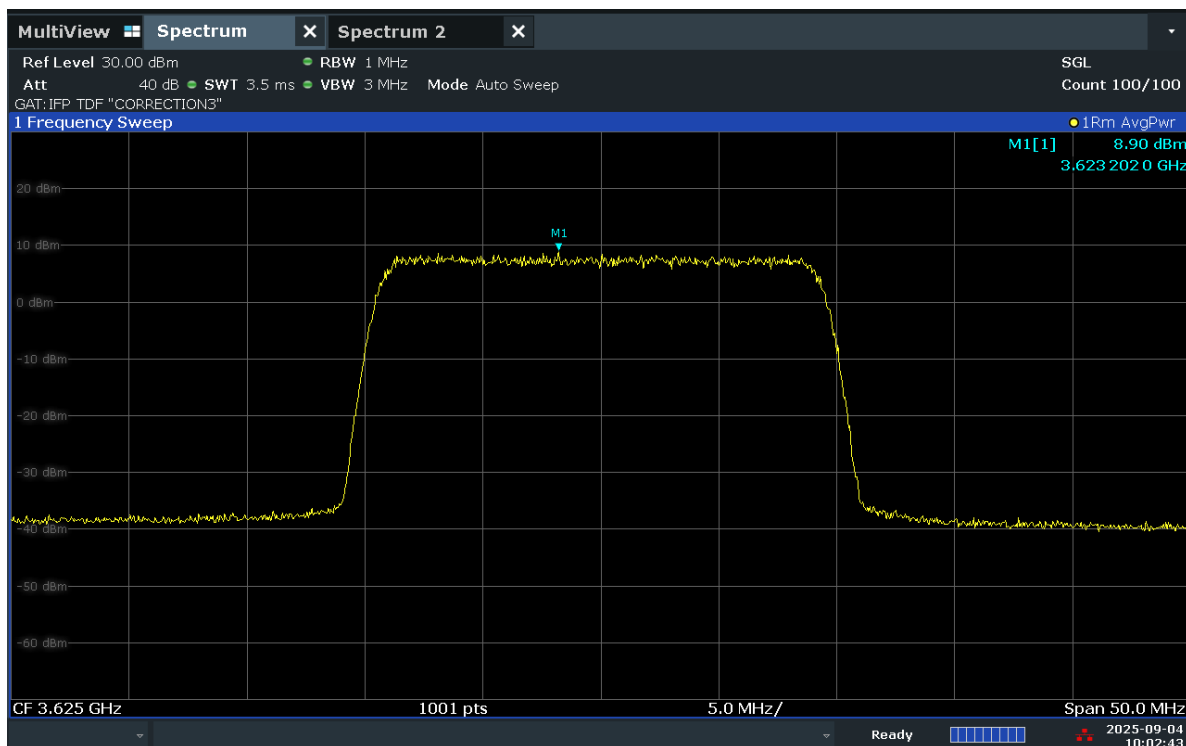
Plot 7.24. Power Spectral Density Plot (20MHz TM3.1a – Mid Channel)
