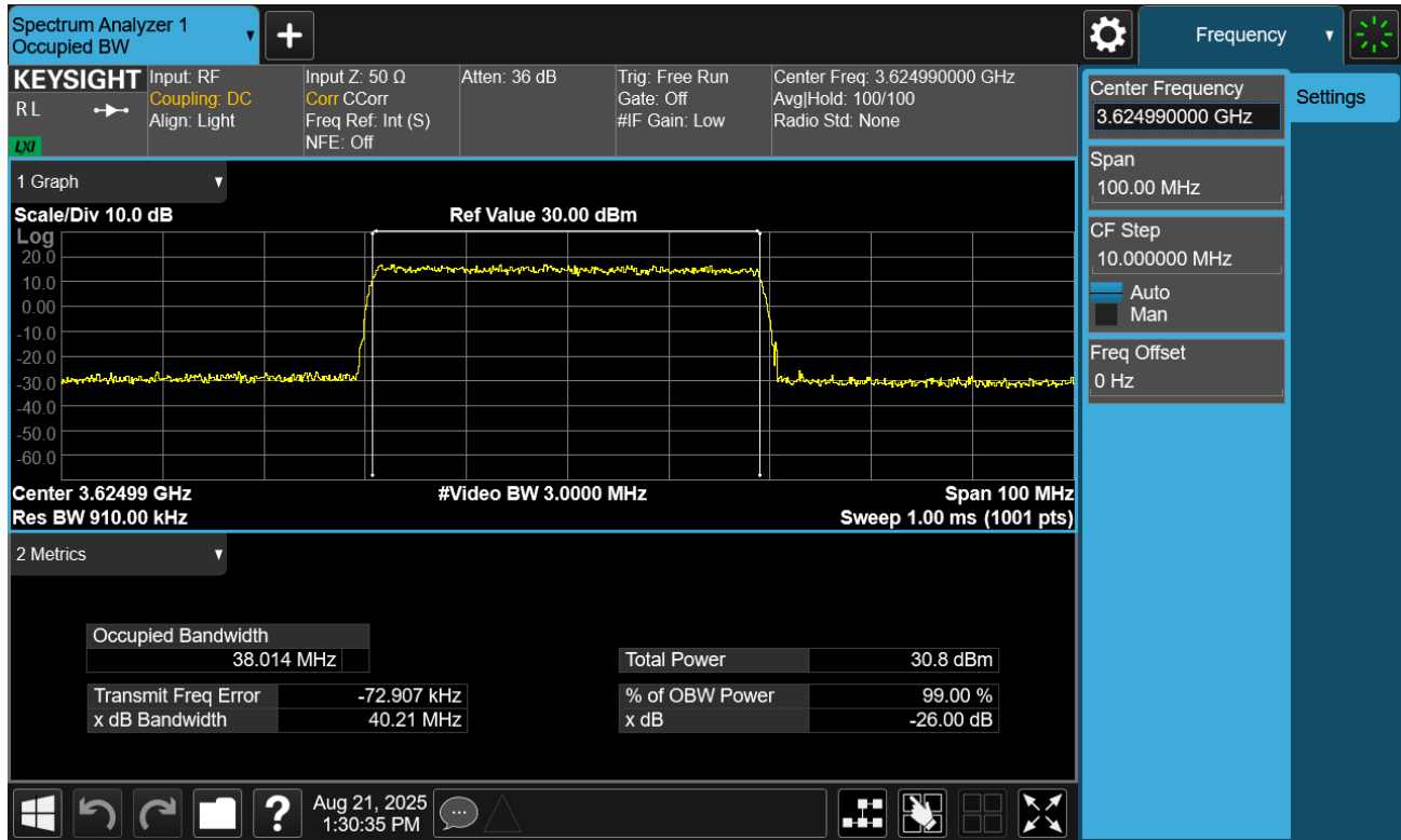
Plot 7.4. Occupied Bandwidth Plot (40MHz TM3.1a)
