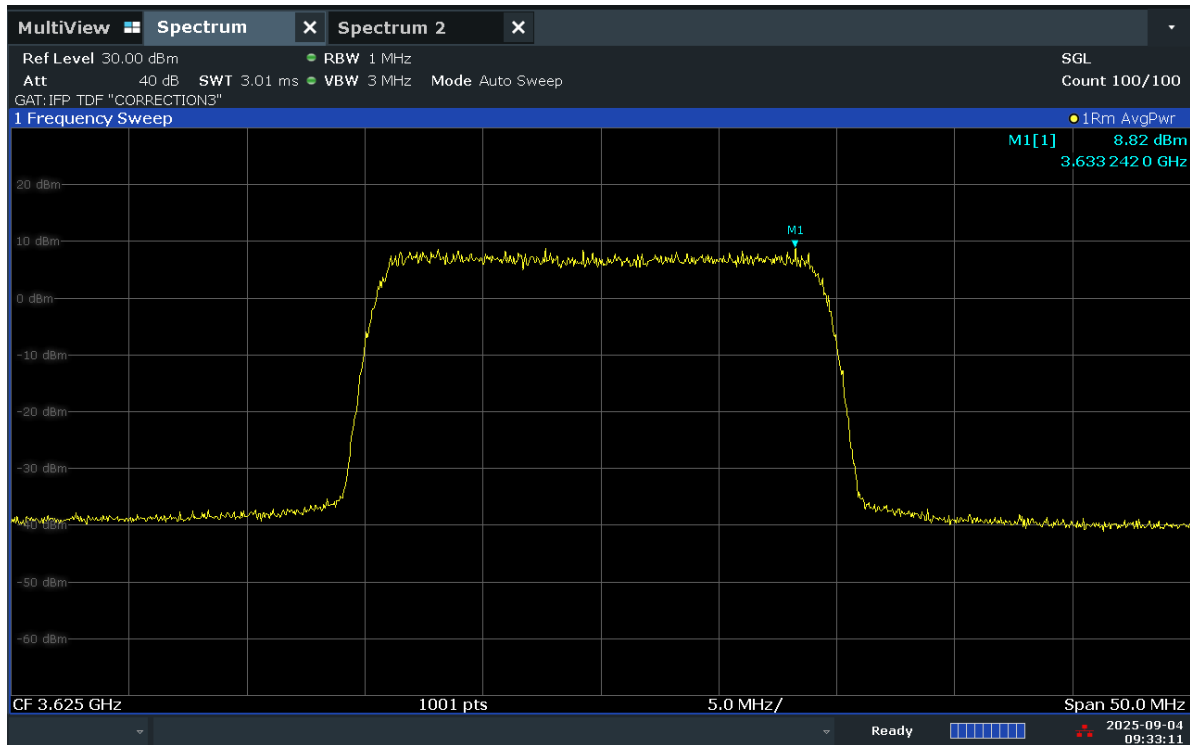
Plot 7.21. Power Spectral Density Plot (20MHz TM1.1- Mid Channel)
