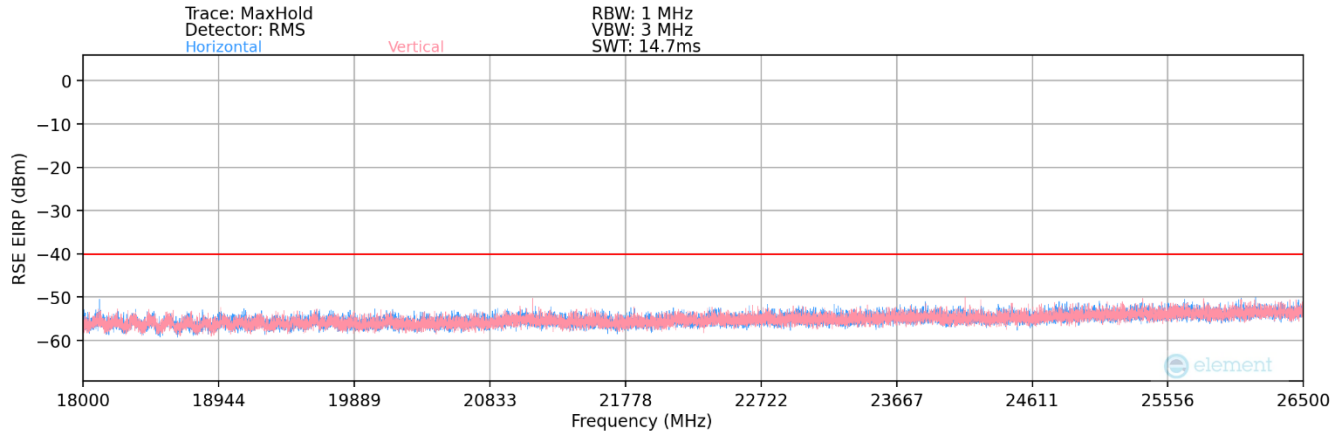
Plot 7.55. Radiated Spurious Plot 18-26.5GHz – Mid Channel
