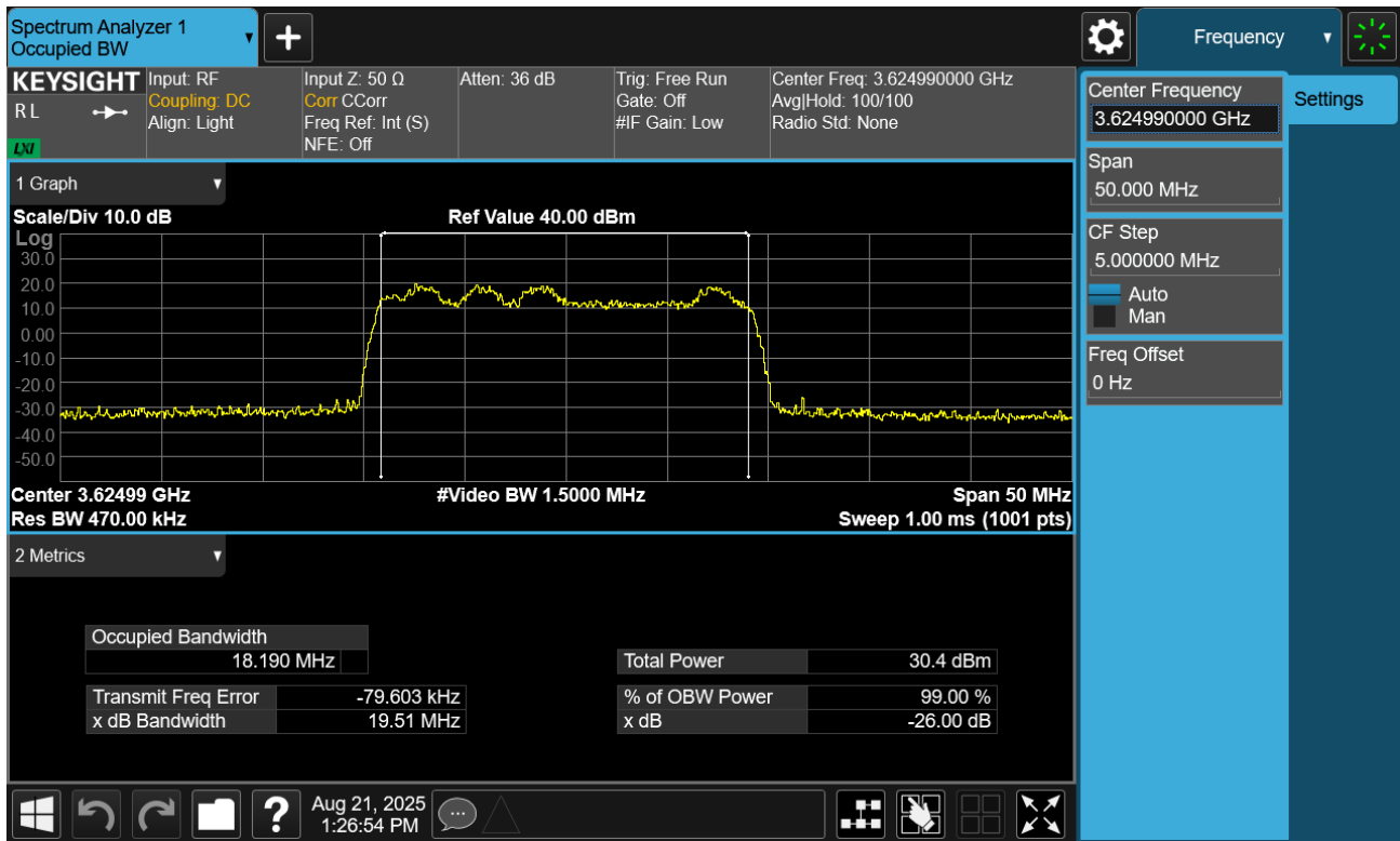
Plot 7.6. Occupied Bandwidth Plot (20MHz TM1.2)
