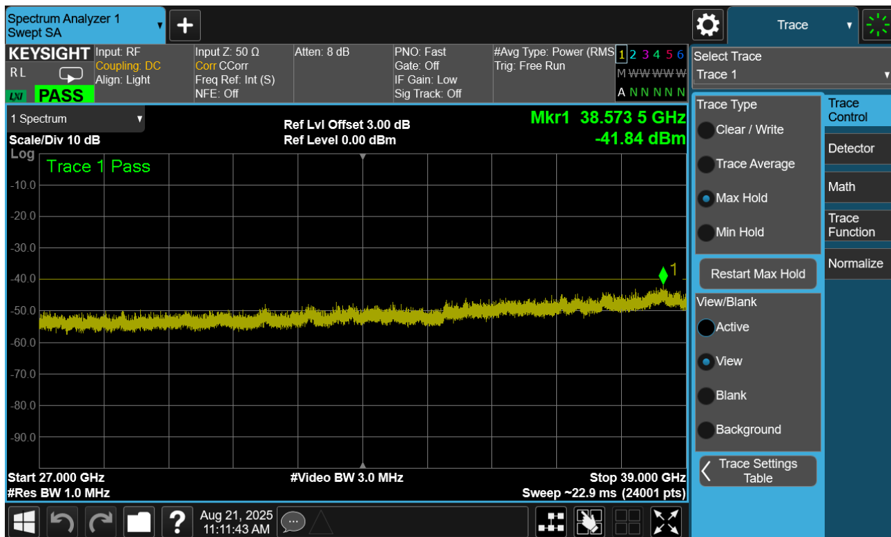
Plot 7.34. Conducted Spurious Plot (20MHz TM1.1, Mid Channel)
