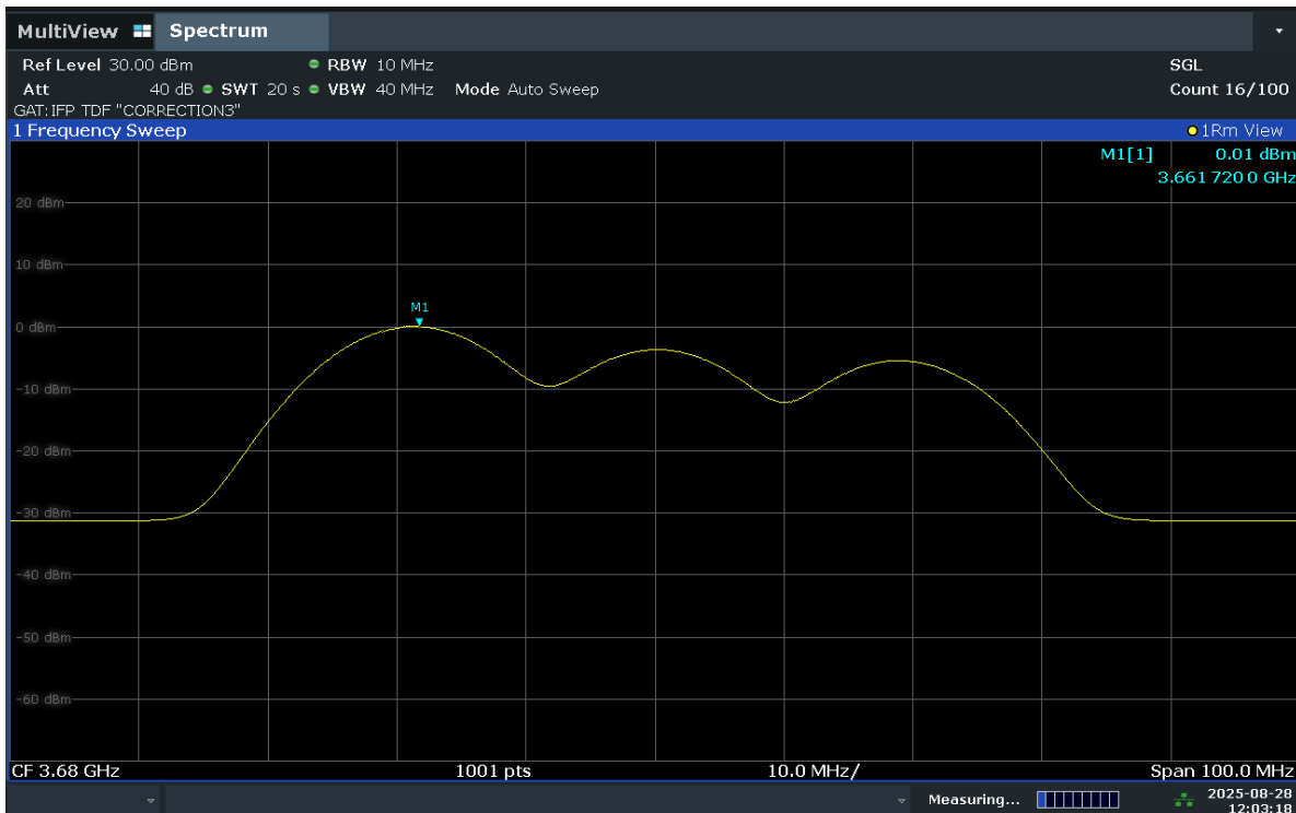
Plot 7.11. Power/10MHz Plot (40MHz TM2a – High Channel)
