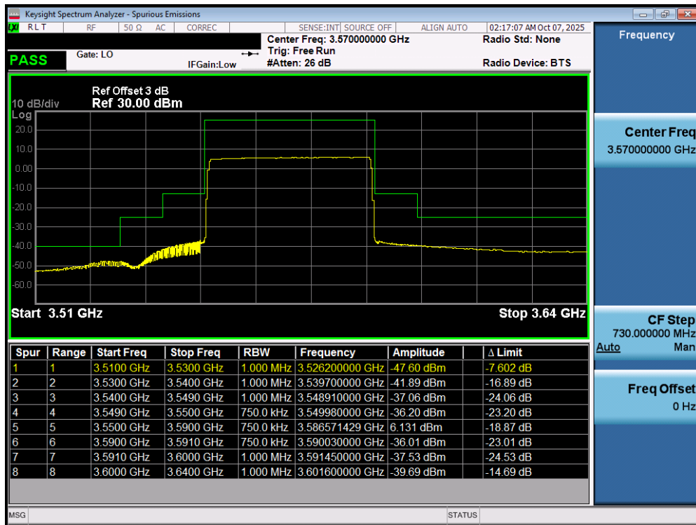
Plot 7.39. Conducted Band Edge Plot (40MHz, TM1.1, Low Channel)
