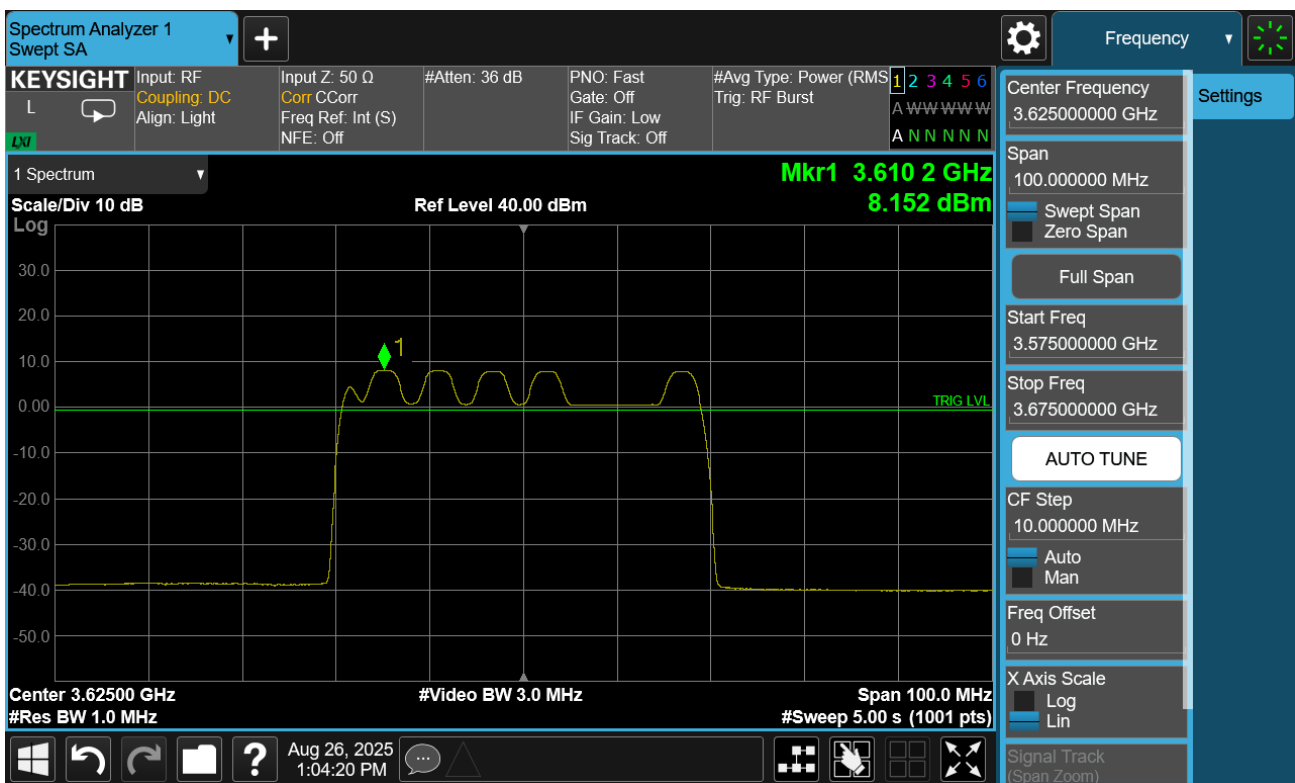
Plot 7.18. Power Spectral Density Plot (40MHz TM1.2 – Mid Channel)
