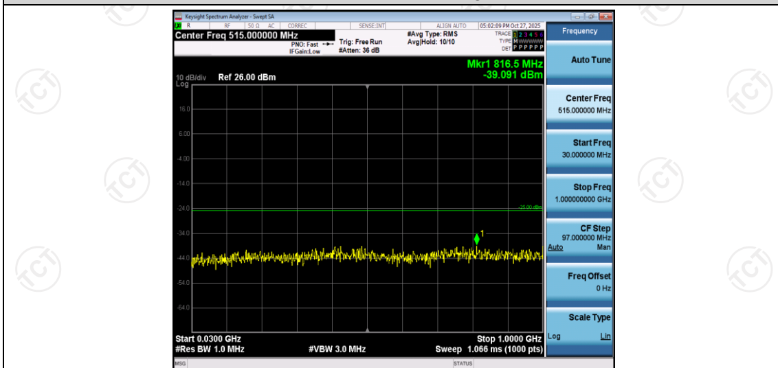
Band7-15MHz-QPSK-20825-1RB#0-Range1:30~1000MHz
