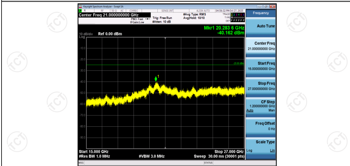
Band7-10MHz-16QAM-21400-1RB#0-Range3:15000~27000MHz
