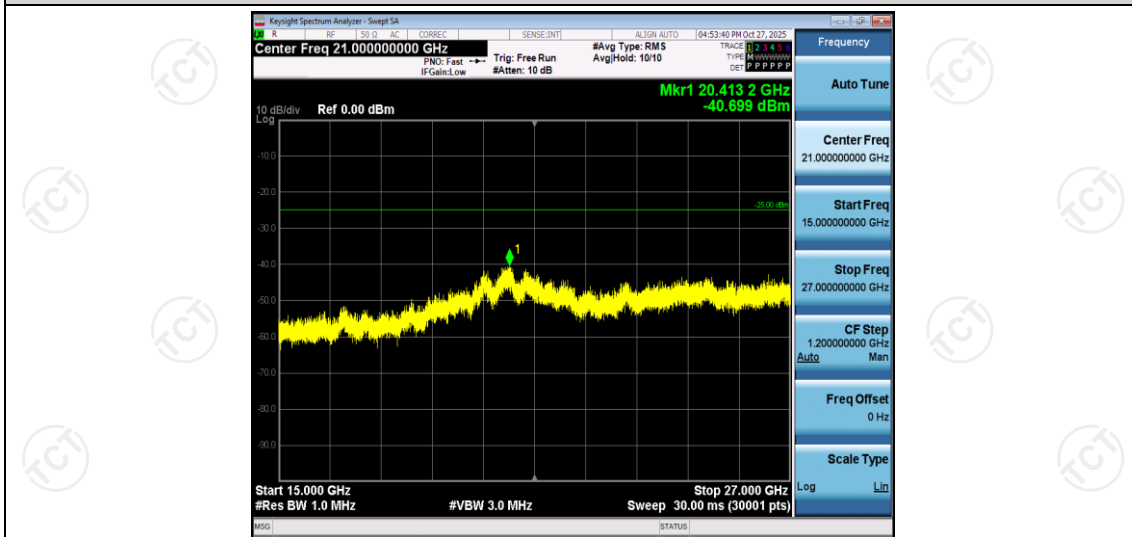
Band7-10MHz-16QAM-20800-1RB#0-Range3:15000~27000MHz
