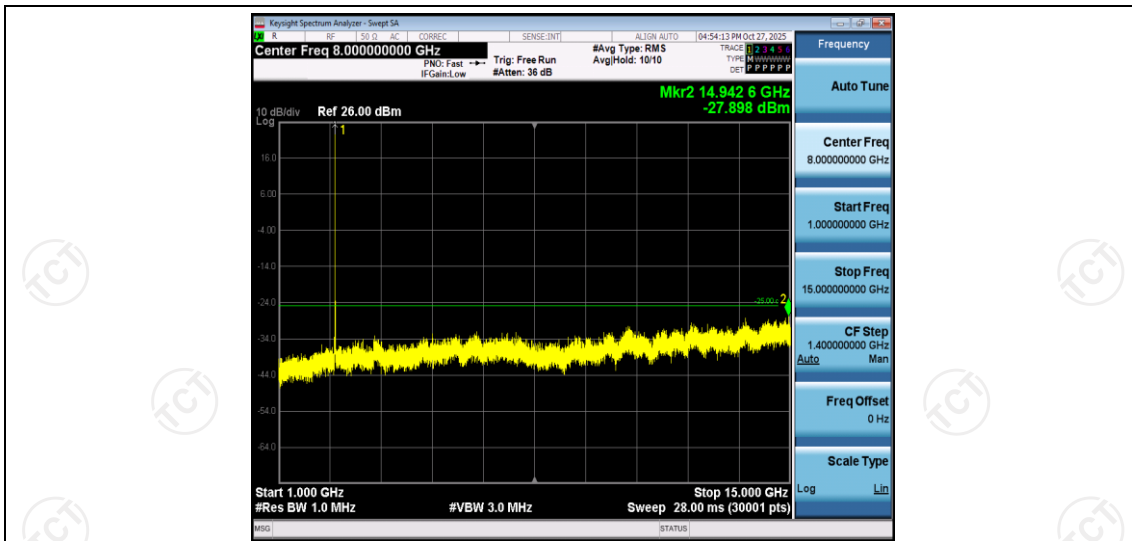
Band7-10MHz-QPSK-21100-1RB#0-Range2:1000~15000MHz
