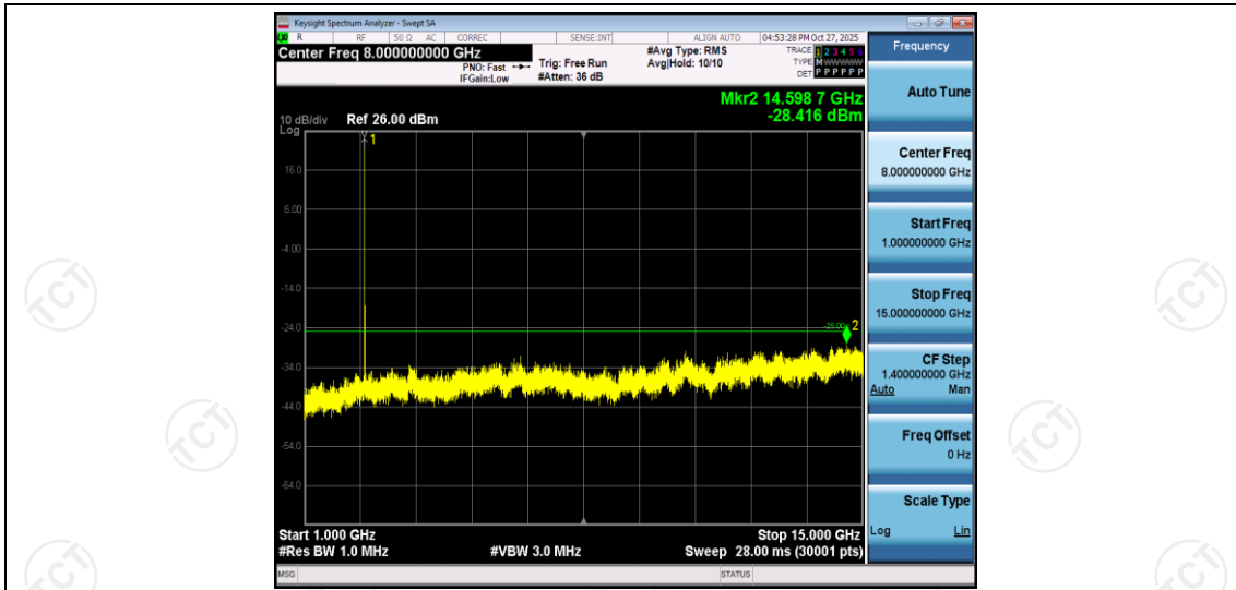
Band7-10MHz-16QAM-20800-1RB#0-Range2:1000~15000MHz
