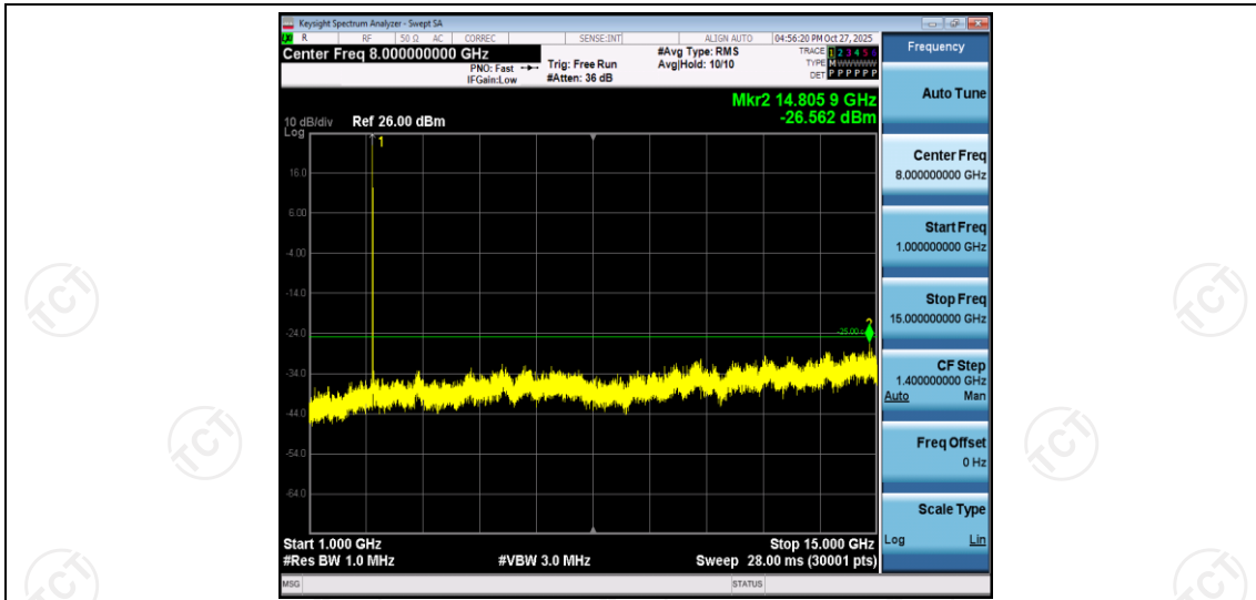
Band7-10MHz-16QAM-21400-1RB#0-Range2:1000~15000MHz
