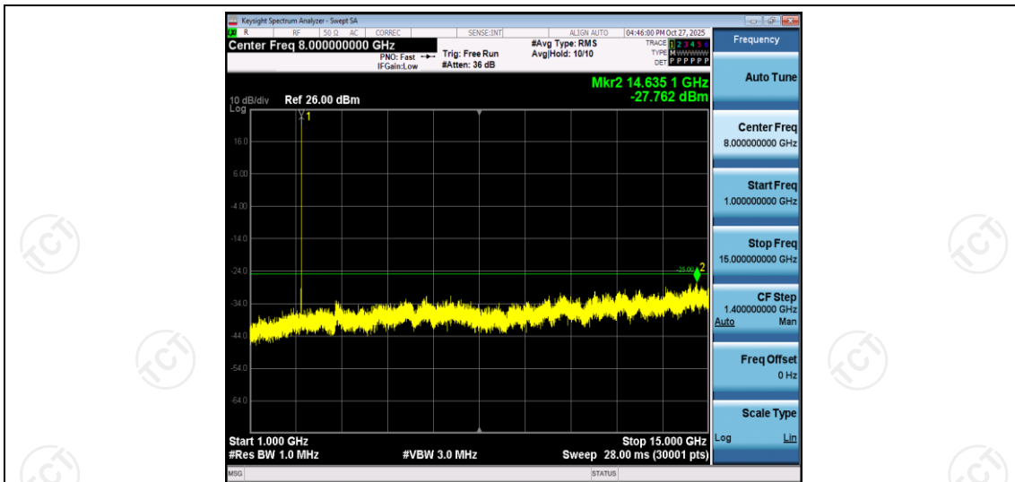
Band7-5MHz-QPSK-21425-1RB#0-Range2:1000~15000MHz
