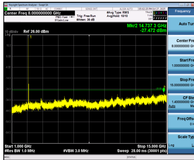
Band7-15MHz-QPSK-20825-1RB#0-Range2:1000~15000MHz
