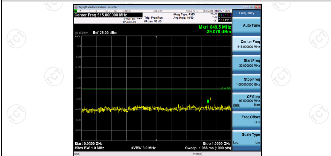
Band7-10MHz-QPSK-21100-1RB#0-Range1:30~1000MHz
