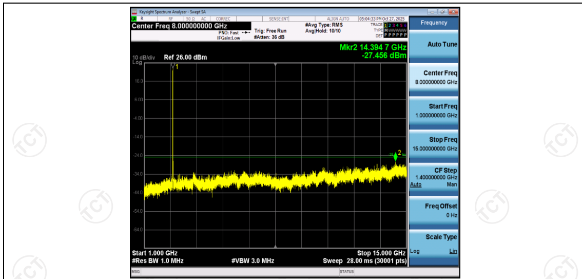
Band7-15MHz-16QAM-21100-1RB#0-Range2:1000~15000MHz
