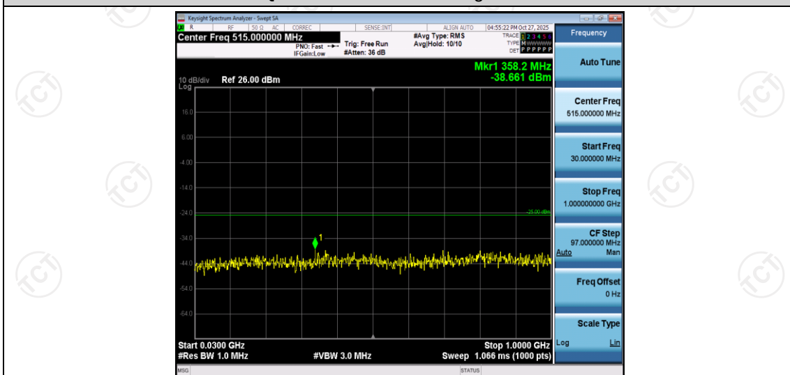
Band7-10MHz-QPSK-21400-1RB#0-Range1:30~1000MHz
