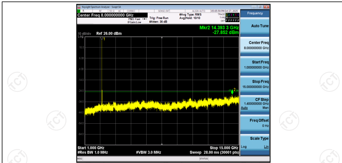
Band7-15MHz-16QAM-21375-1RB#0-Range2:1000~15000MHz
