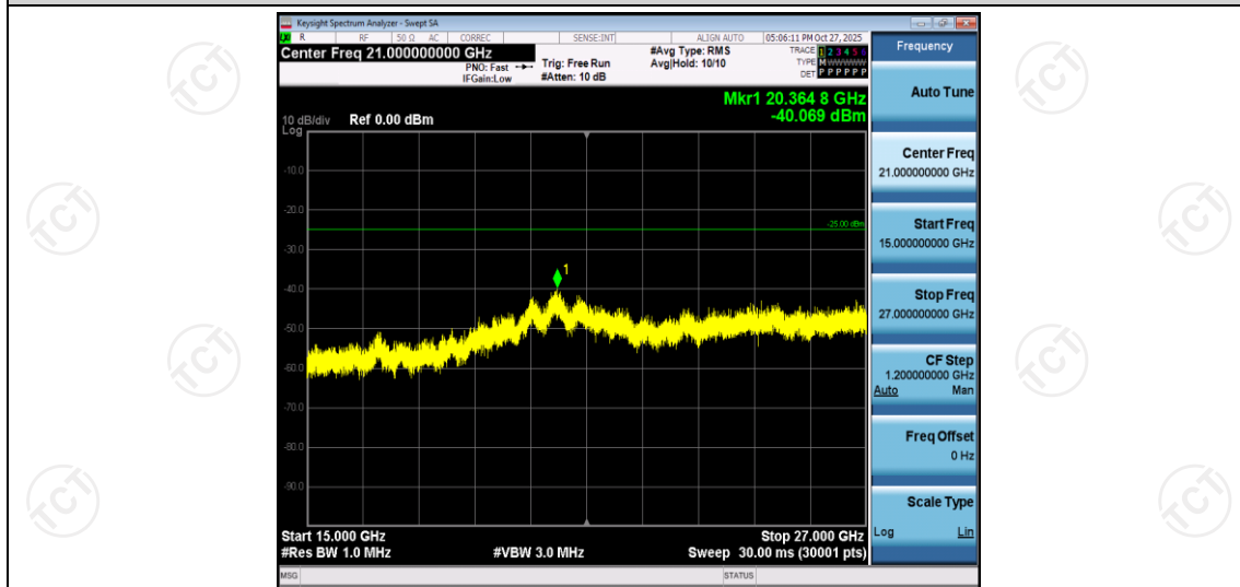
Band7-15MHz-16QAM-21375-1RB#0-Range3:15000~27000MHz
