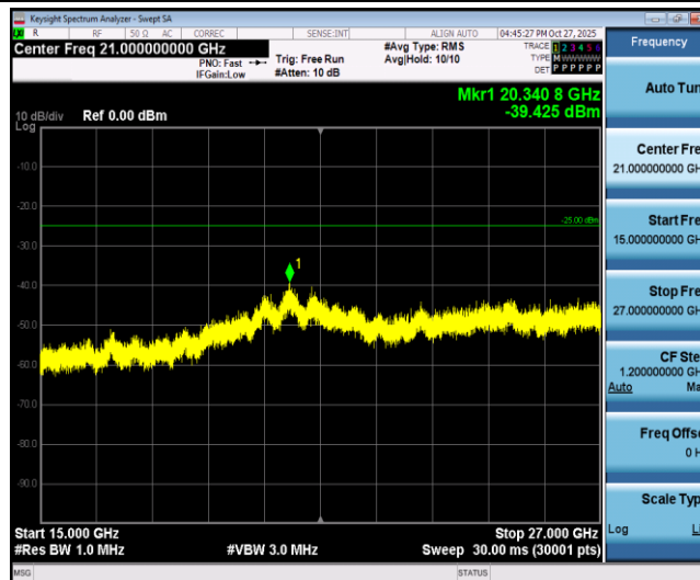
Band7-5MHz-16QAM-21100-1RB#0-Range3:15000~27000MHz
