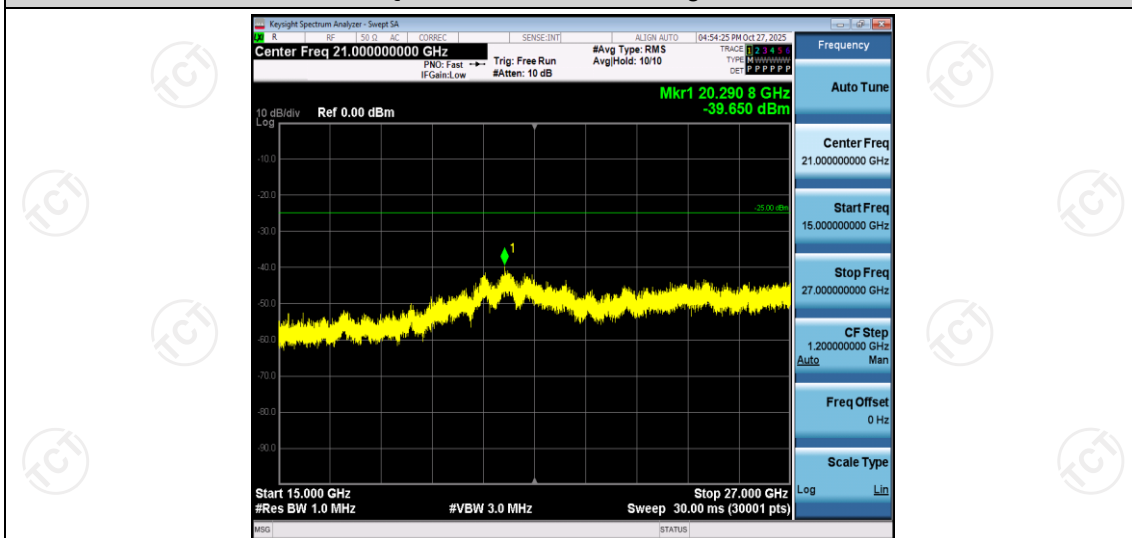
Band7-10MHz-QPSK-21100-1RB#0-Range3:15000~27000MHz
