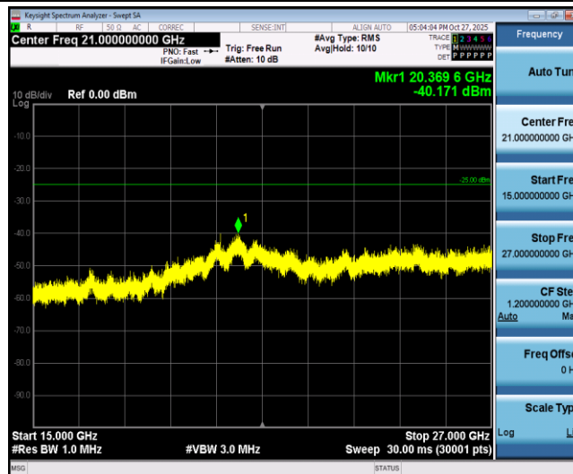
Band7-15MHz-QPSK-21100-1RB#0-Range3:15000~27000MHz
