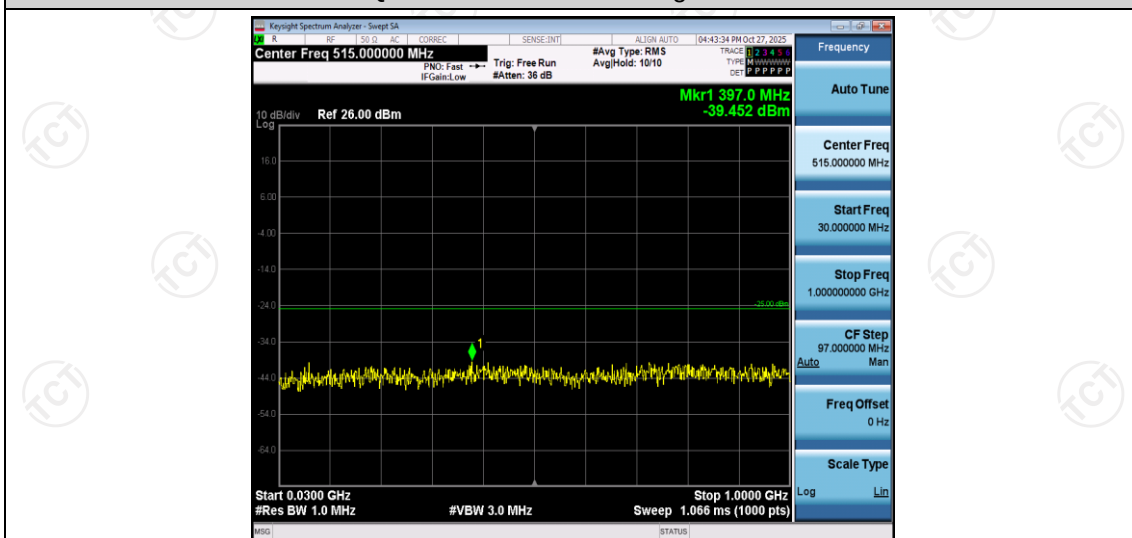
Band7-5MHz-16QAM-20775-1RB#0-Range1:30~1000MHz
