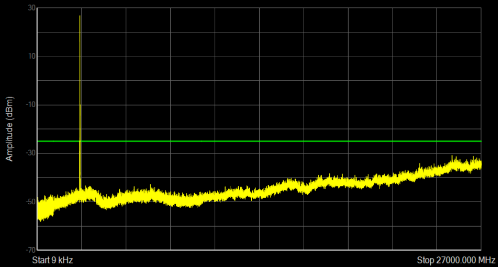
Band38 16QAM BW=10MHz Channel=38200 RB Size=1 Position=#0
