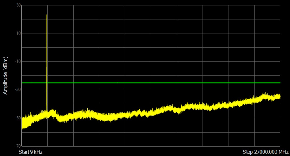
Band38 16QAM BW=10MHz Channel=37800 RB Size=1 Position=#0
