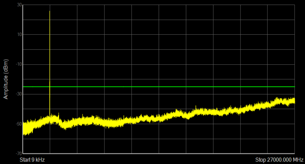
Band41 16QAM BW=5MHz Channel=41565 RB Size=1 Position=#0
