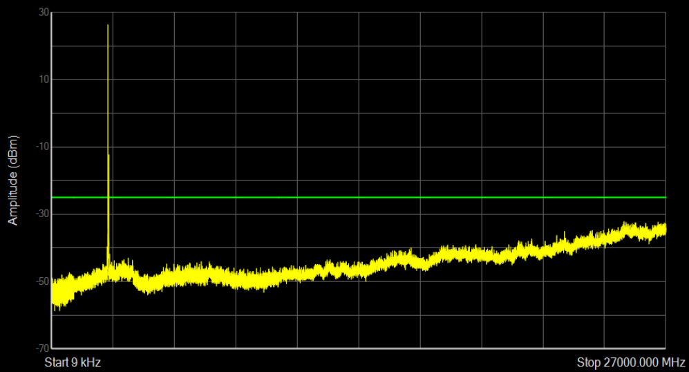
Band41 16QAM BW=20MHz Channel=39750 RB Size=1 Position=#0
