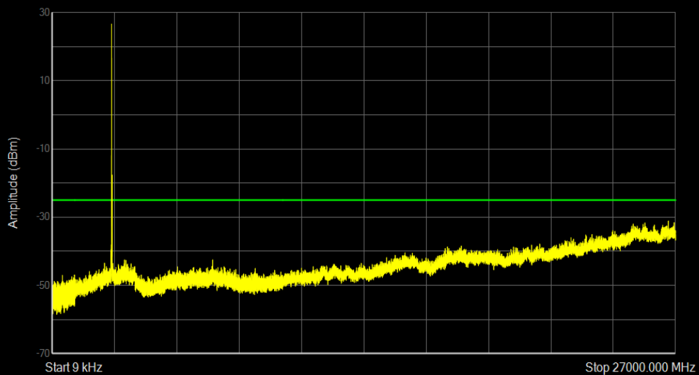
Band41 16QAM BW=15MHz Channel=40620 RB Size=1 Position=#0
