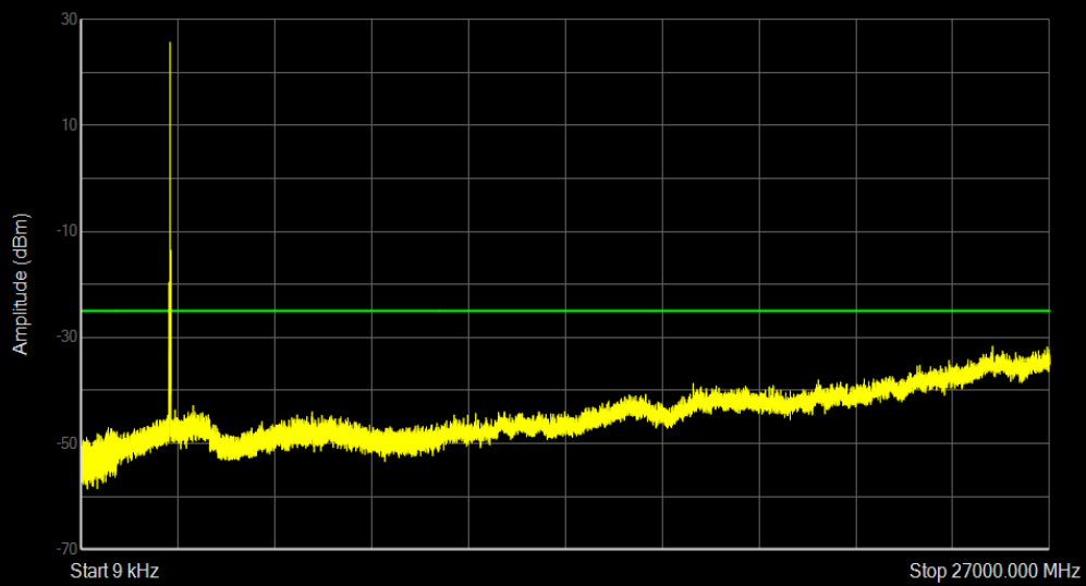
Band41 16QAM BW=15MHz Channel=39725 RB Size=1 Position=#0
