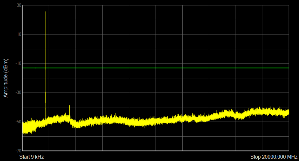
Band66 16QAM BW=3MHz Channel=132657 RB Size=1 Position=#0
