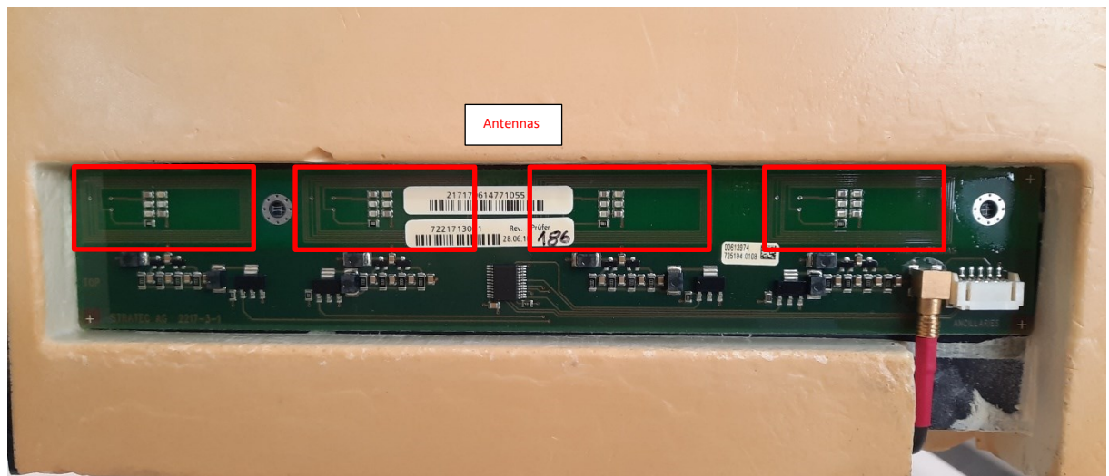
Fig. 3 View on the Quad RFID Antenna PCBA to communicate with the Tags on the Ancillary bottles
