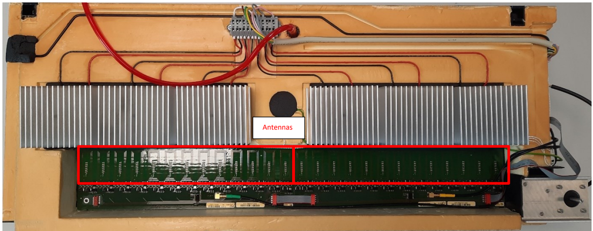
Fig. 2 View on the 13-fold Antenna PCBAs to communicate with the Tags on the Reagent Integrals
