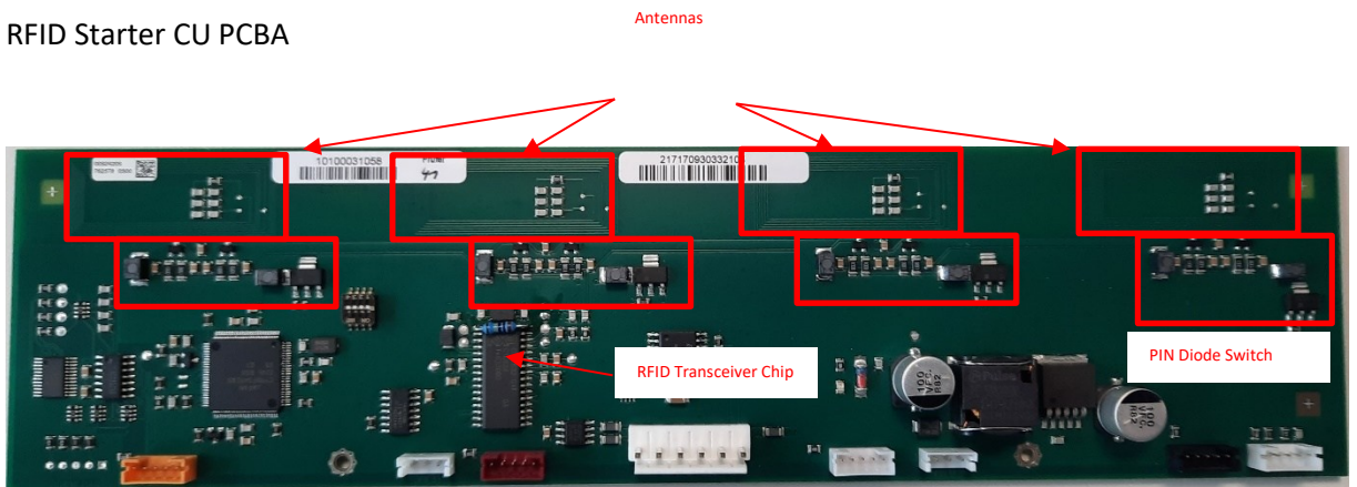
Component Side
