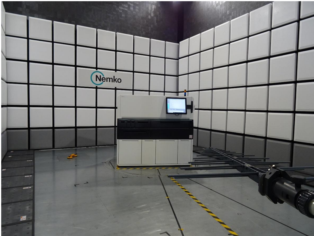
Radiated Spurious Emission from 200 MHz to 1000 MHz
