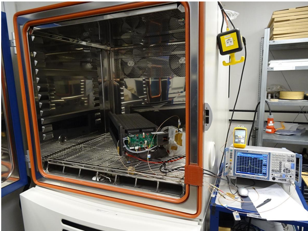
Conducted Emission
