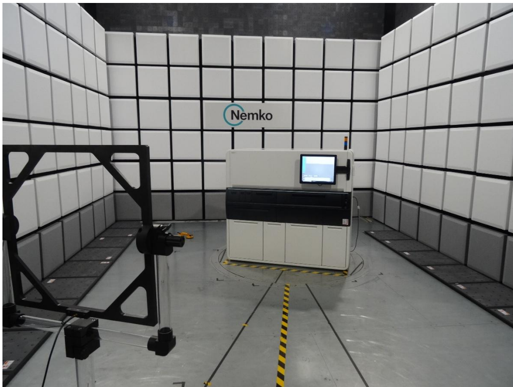
Radiated Spurious Emission from 9 kHz to 30 MHz
