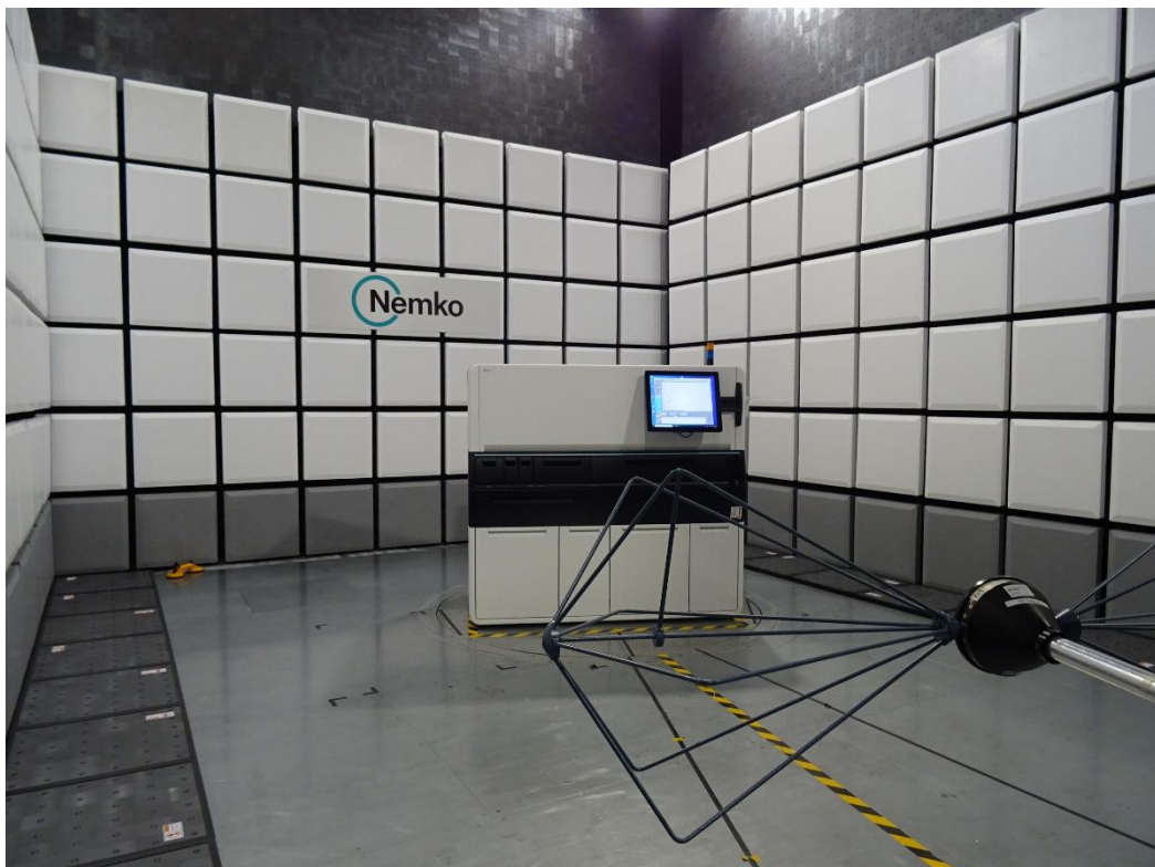
Radiated Spurious Emission from 30 MHz to 200 MHz
