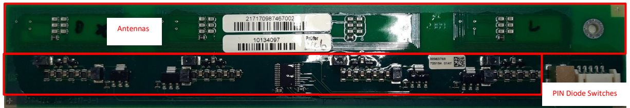
Component Side
