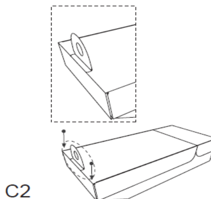
Figure 5–46: LIAISON® EASY Waste assembling instruction step C2
