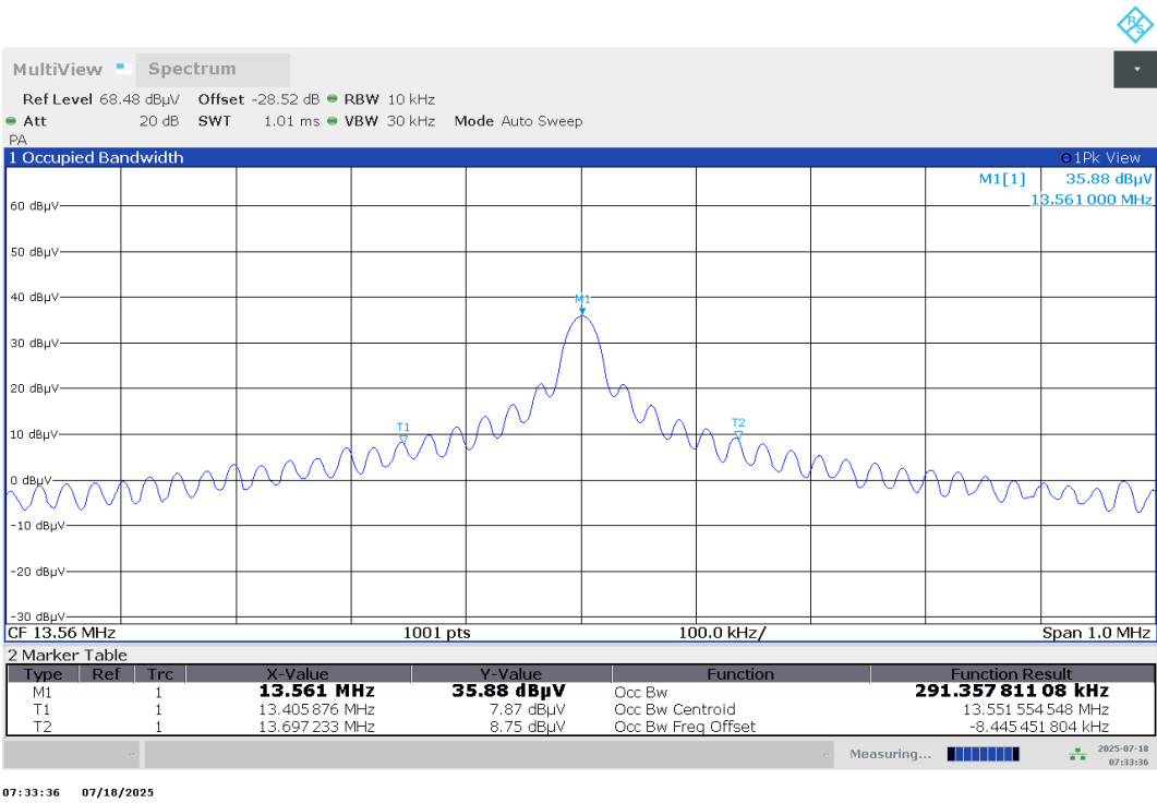
Plot no. 15: Frequency tolerance @ -35 °C, EUT A, Vmin, set-up 2
