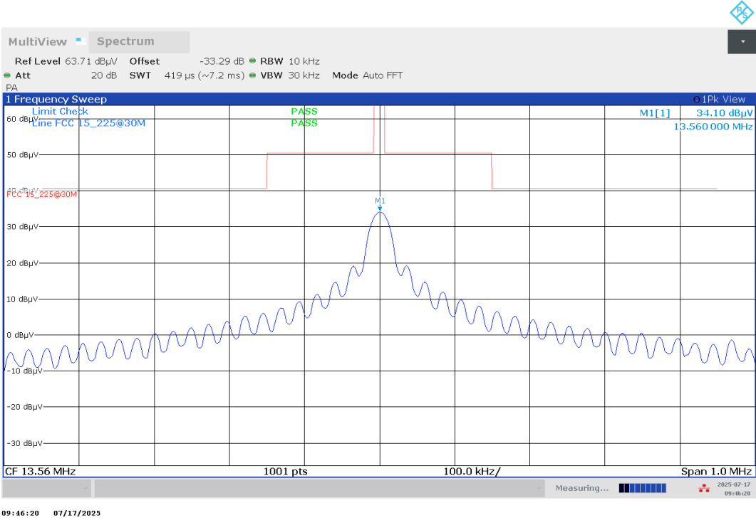
Plot no. 2: Transmitter Spectrum Mask (TSM), set-up 3
