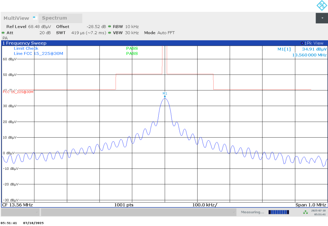
Plot no. 1: Transmitter Spectrum Mask (TSM), set-up 1
