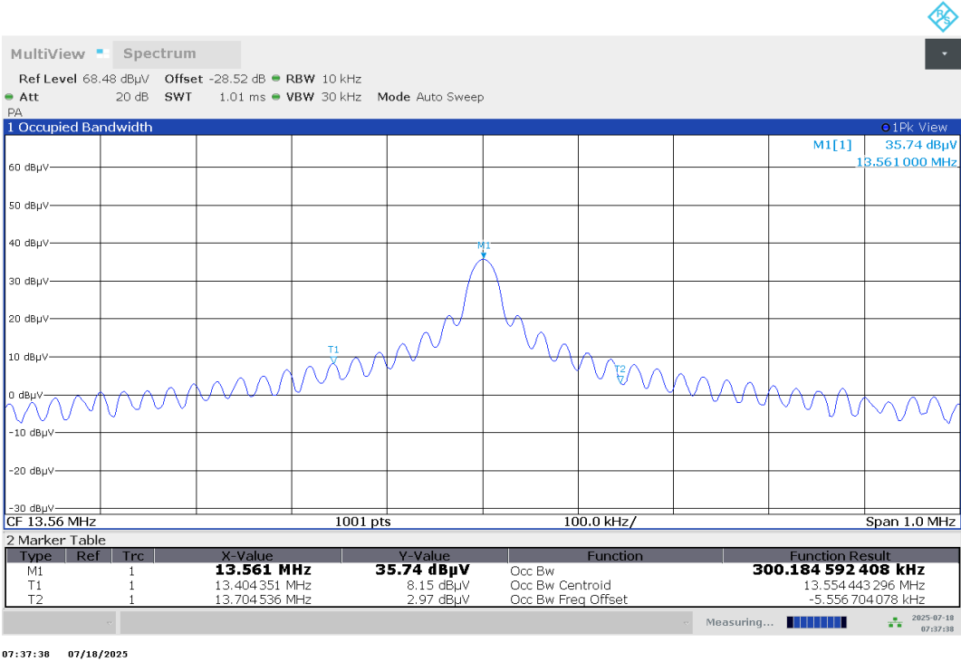
Plot no. 16: Frequency tolerance @ -35 °C, EUT A, Vmax, set-up 2
