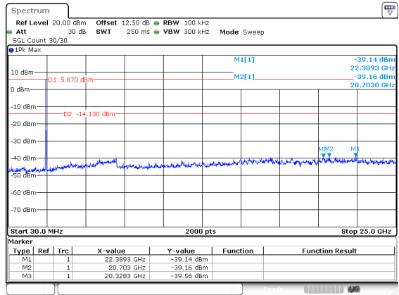
802.11g_2442MHz
