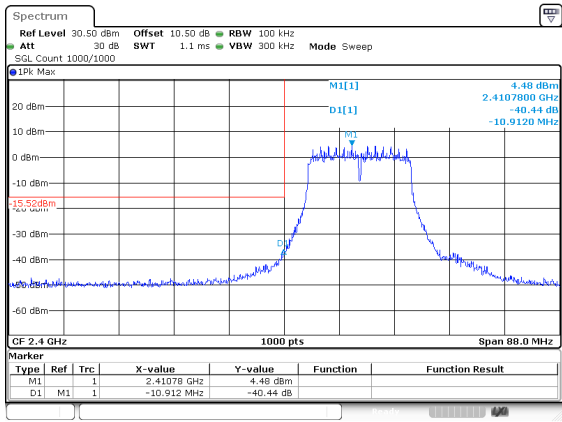
802.11g_2412MHz
