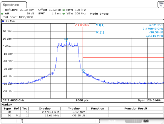
802.11g_2472MHz
