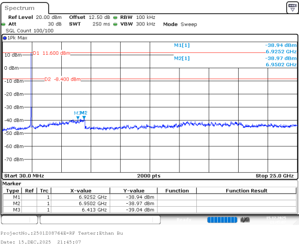
802.11g_2412MHz
