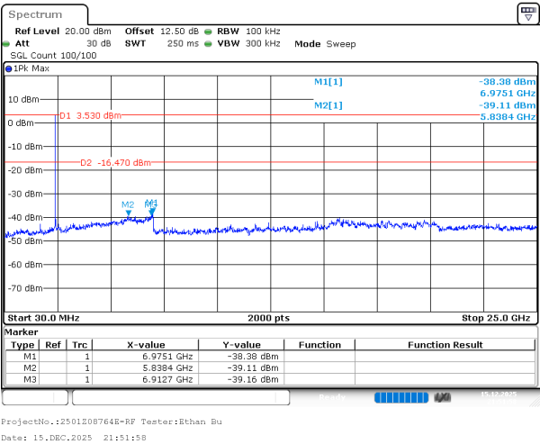
802.11g_2412MHz
