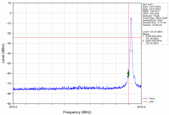
LE: Band edge-left side
