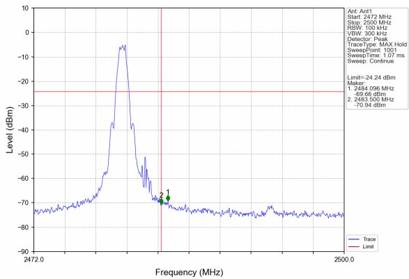
LE: Band edge-right side
