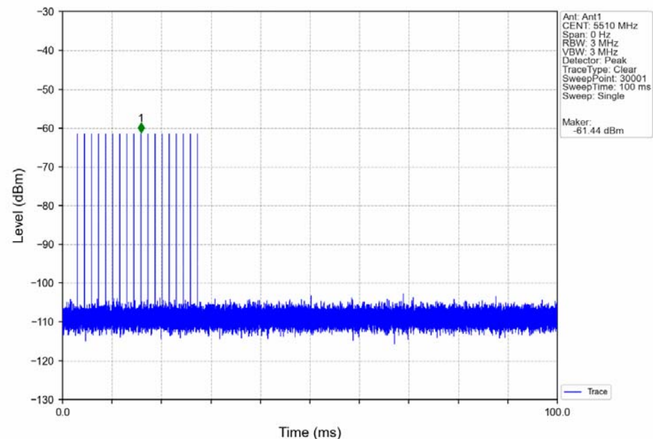
Radar Signal 5510
