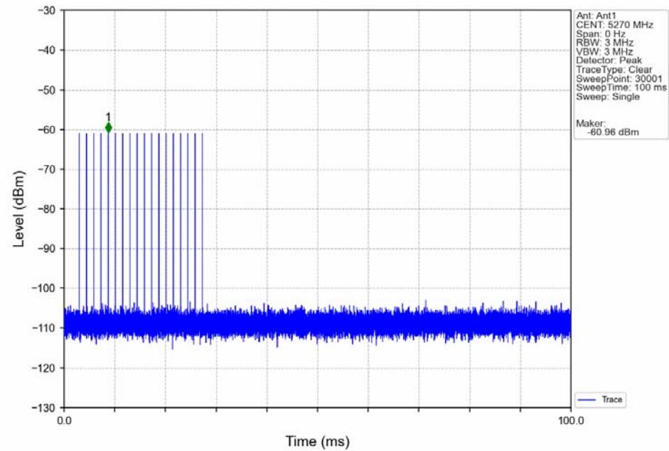
Radar Signal 5270
