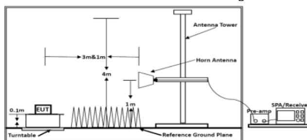
Above 1GHz
