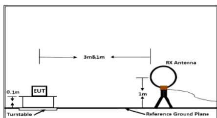
Below 30MHz
