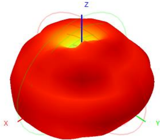
5800.0MHz H+V, Eff: 72.0%
