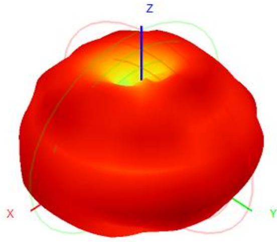
5850.0MHz H+V, Eff: 79.1%
