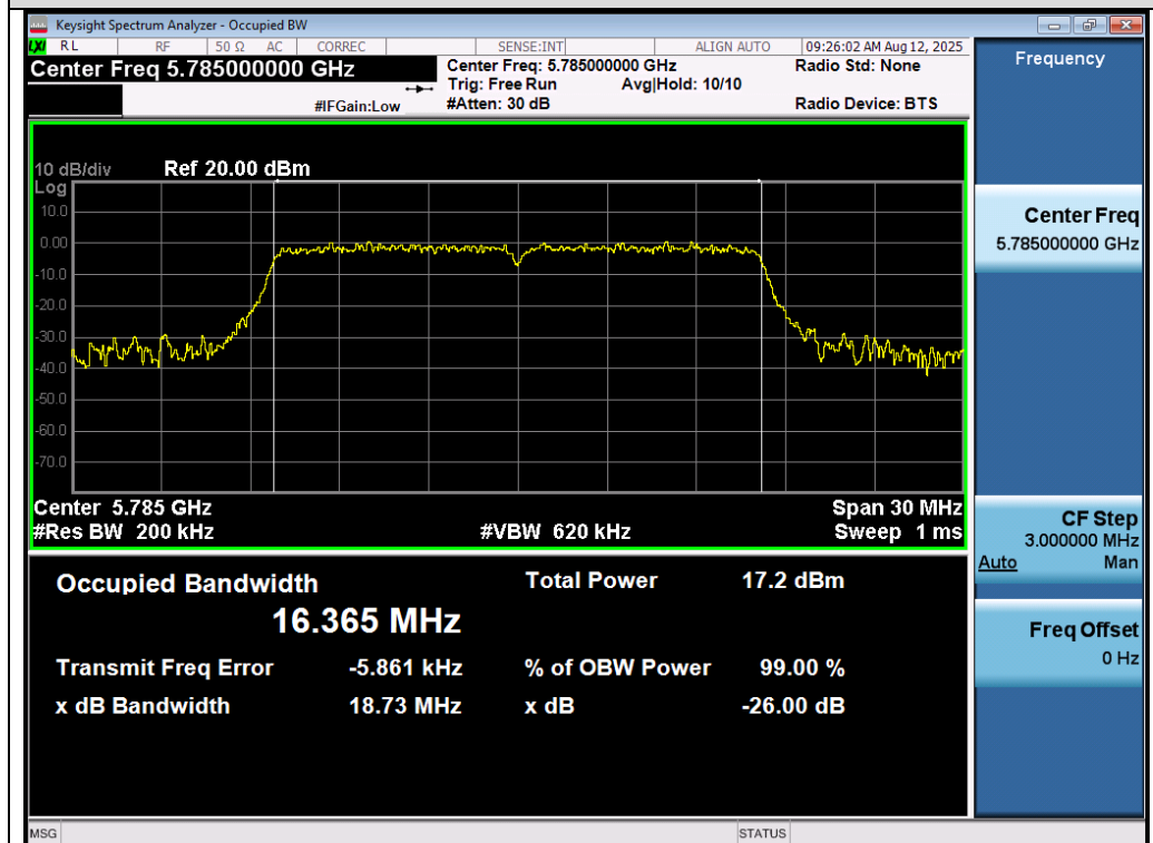
Test_Graph_802.11a_Chain A_5785_6Mbps_OBW
