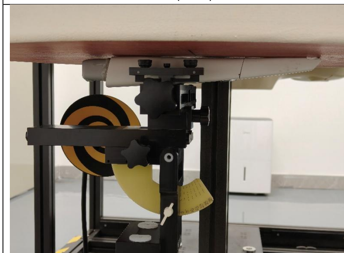
Rear (0mm)
