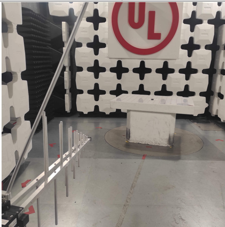
Radiated emission, 30-1000 MHz
