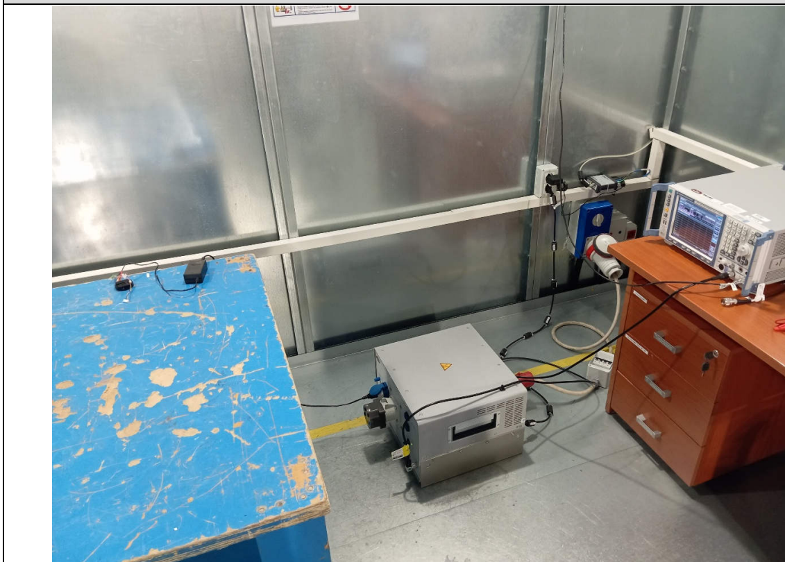
Transmitter AC conducted emissions
