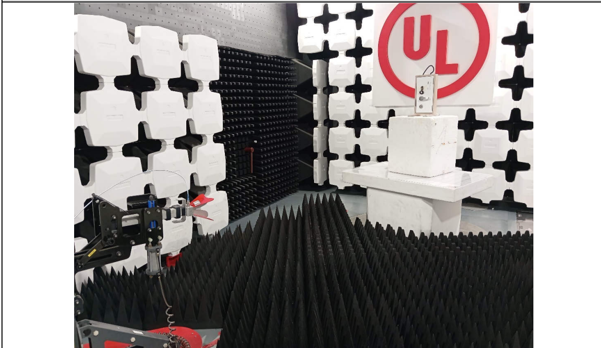
Radiated emission, 1-4 GHz
