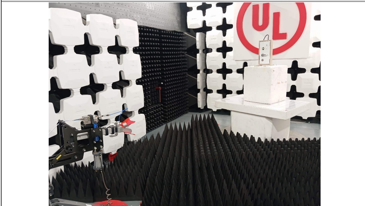
Radiated emission, 4-18 GHz
