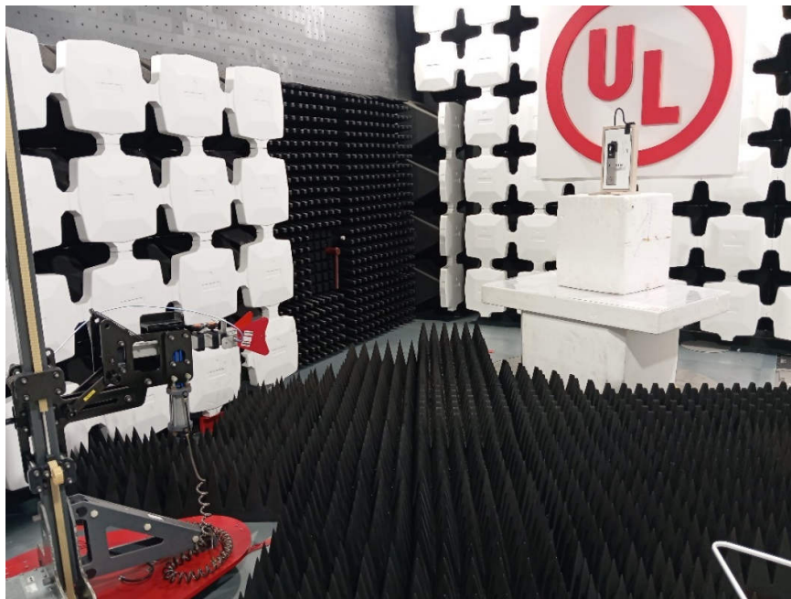
Radiated emission, 4-18 GHz
