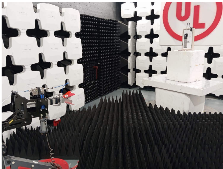
Radiated emission, 4-18 GHz
