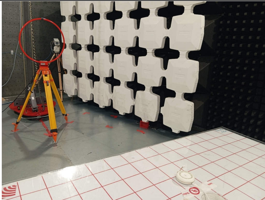
Radiated emission, below 30 MHz CLOSE UP VIEW OF EUT
