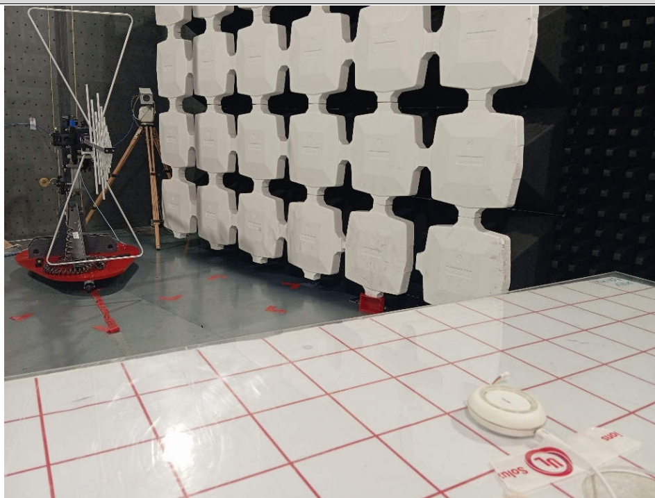
CLOSE UP VIEW OF EUT – 30-1000 MHz
