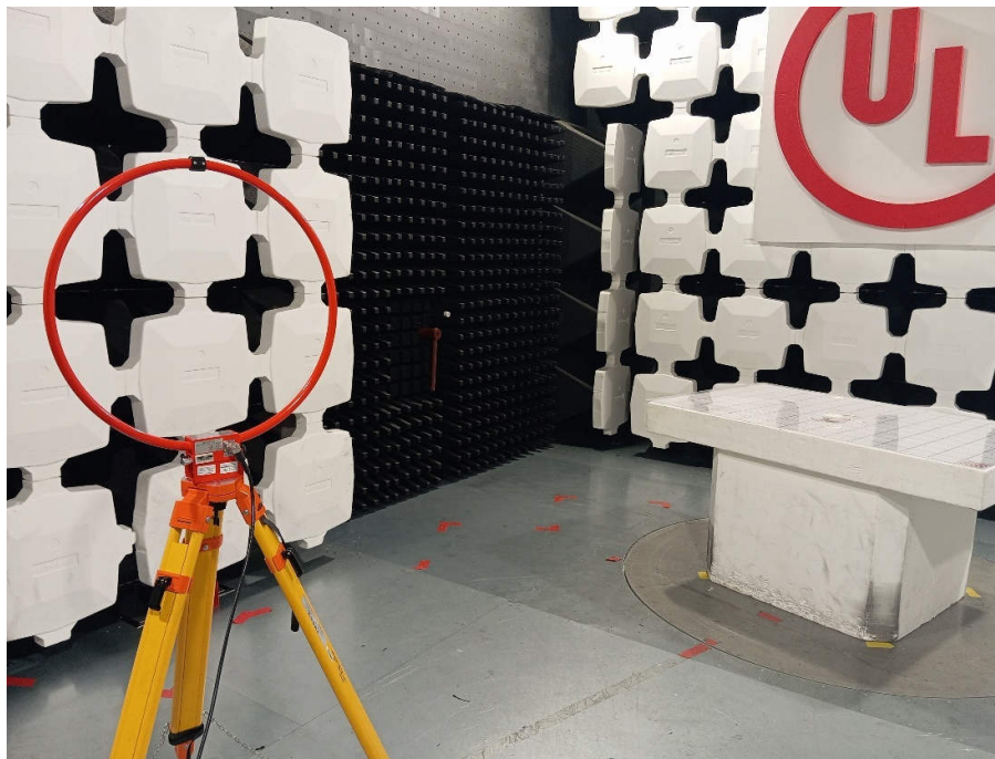
Radiated emission, below 30 MHz AXIS Y
