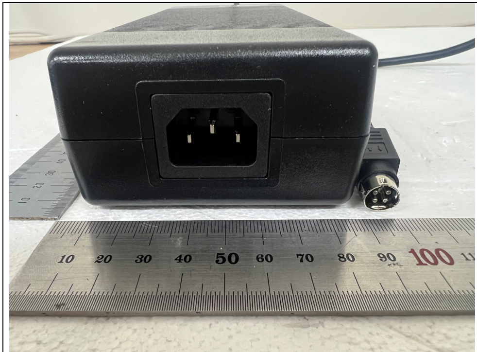
Adapter Port
