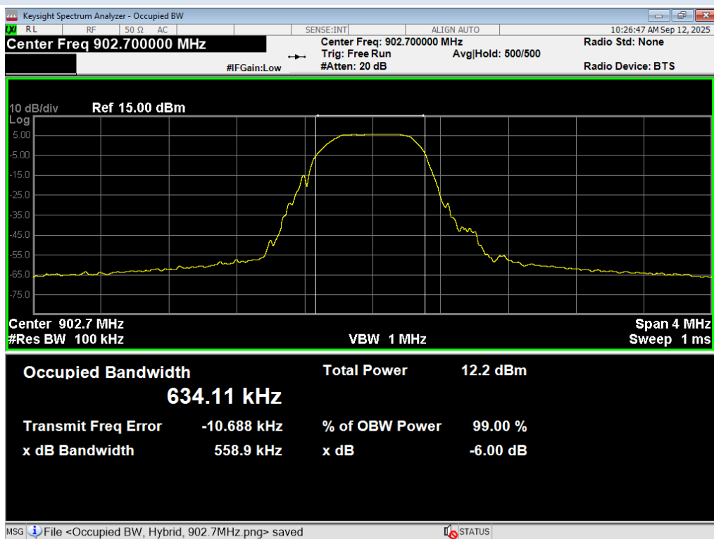
6dB BW, DTS, 902.7MHz
