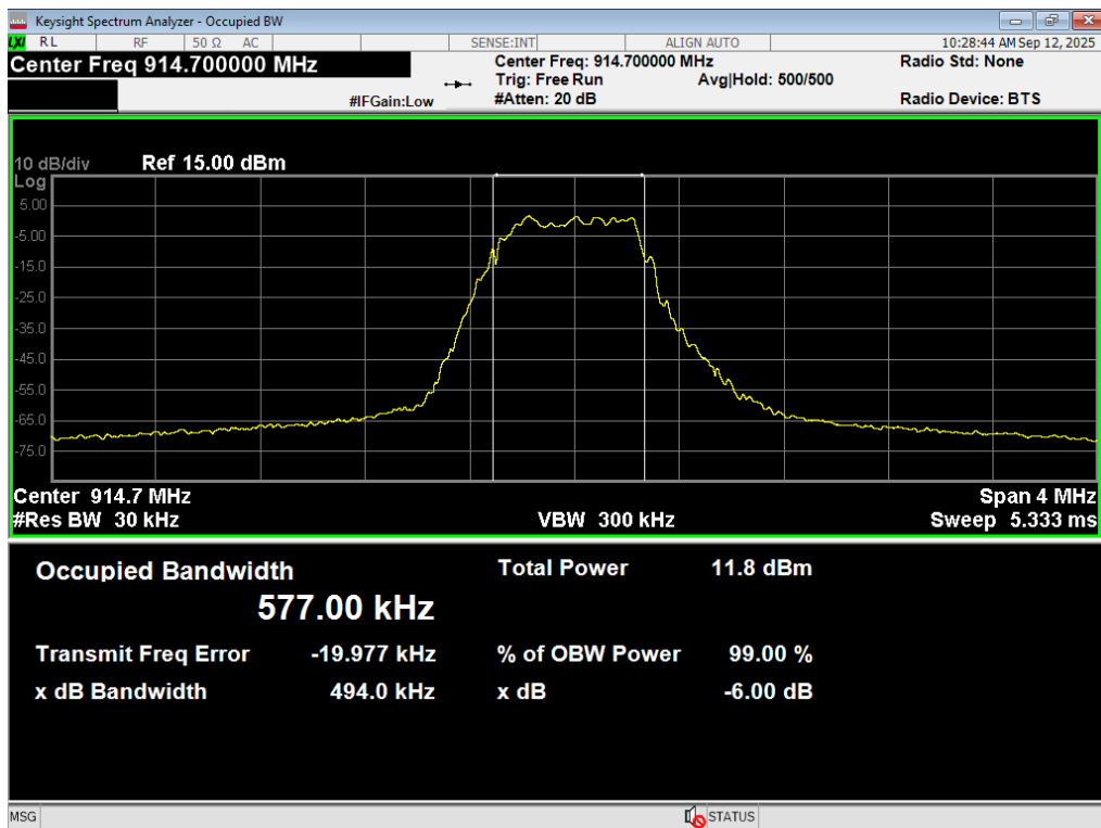
Occupied BW, DTS, 914.7MHz
