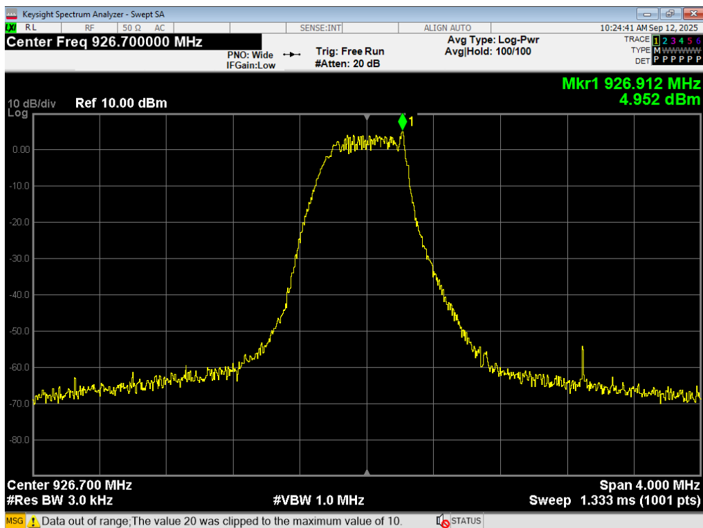
PSD, DTS, 926.7MHz
