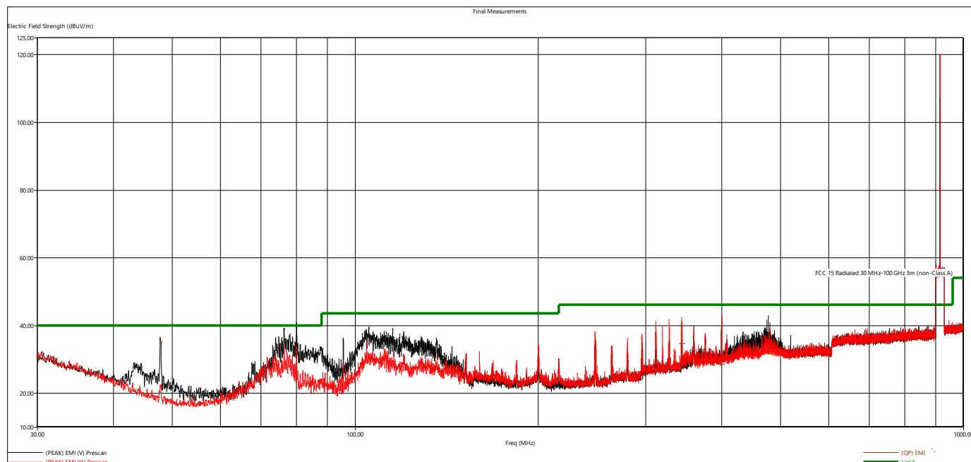
Figure 5 - Radiated Emissions Plot, Mid
