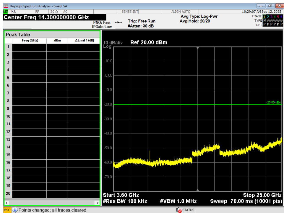
Figure 9 - Conducted Spurious Emissions Plot, LoRa, 3.6GHz – 25GHz
