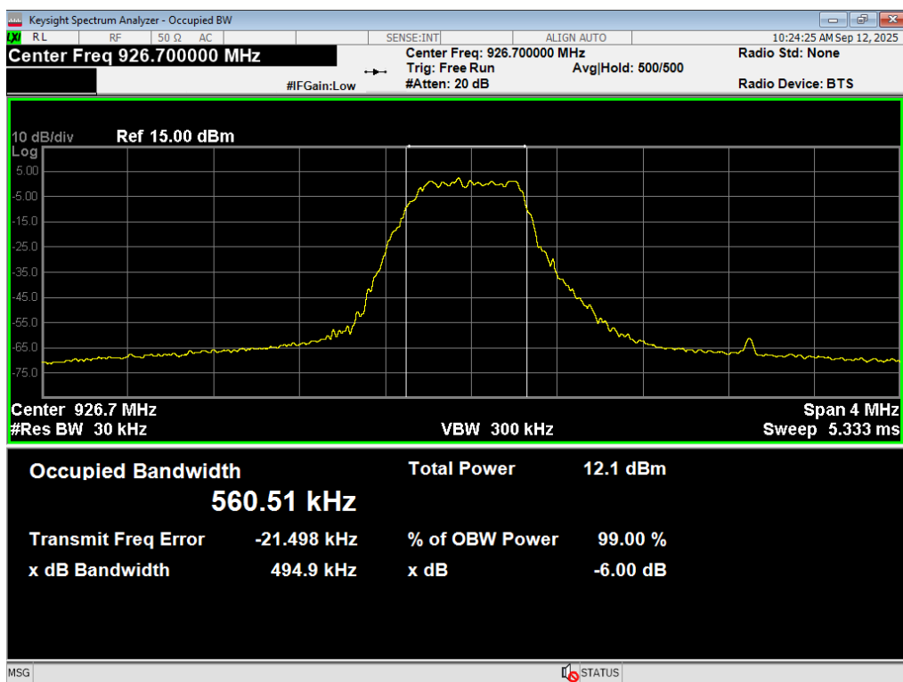
Occupied BW, DTS, 926.7MHz
