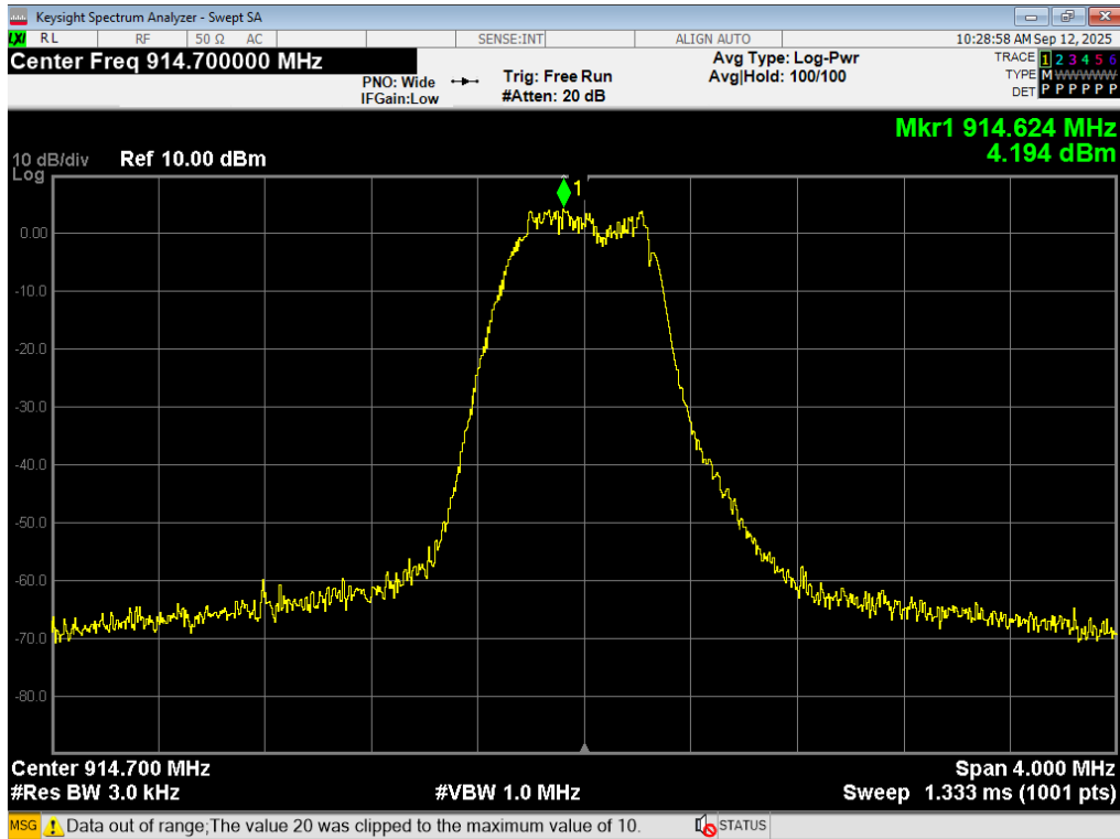
PSD, DTS, 914.7MHz
