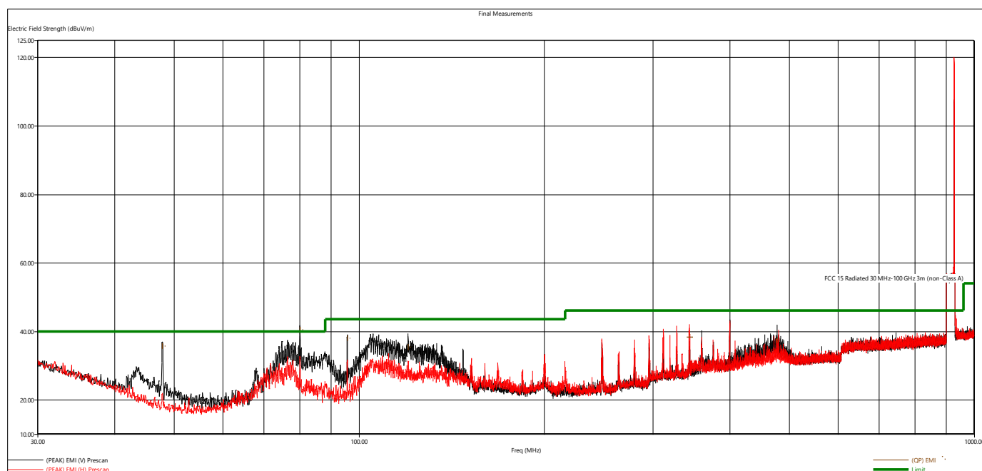
Figure 6 - Radiated Emissions Plot, High
