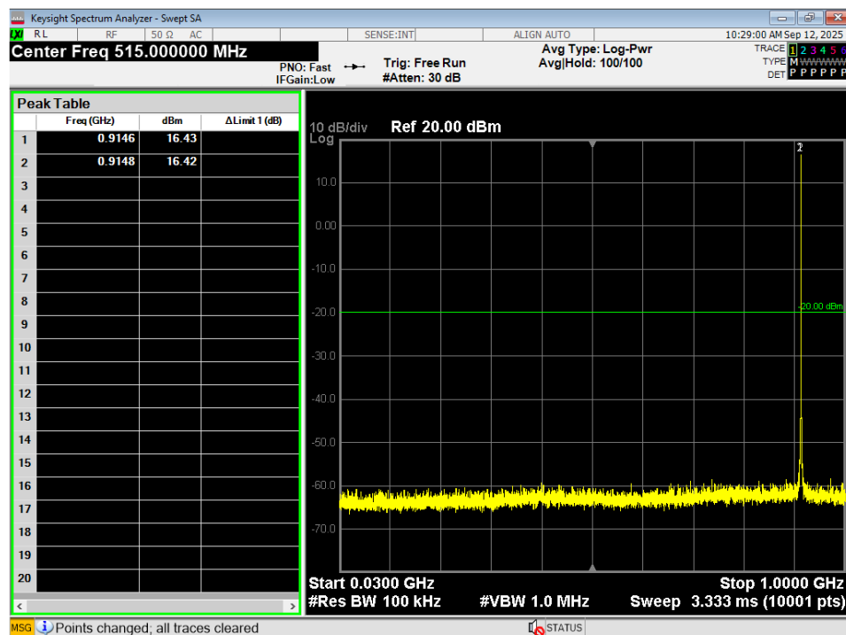
Figure 7 – Conducted Spurious Emissions Plot, LoRa, 30MHz – 1GHz
