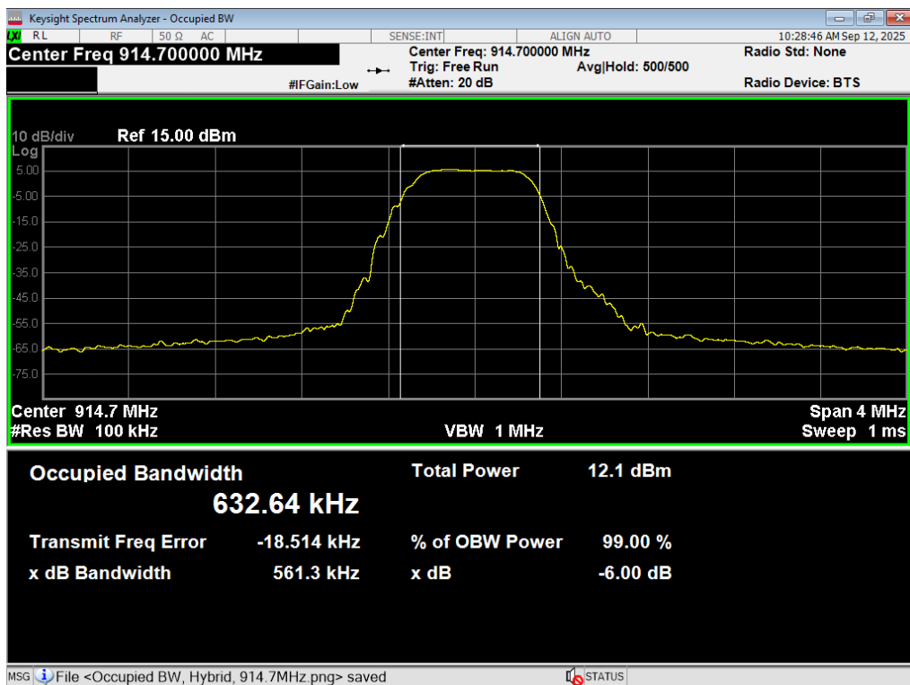
6dB BW, DTS, 914.7MHz
