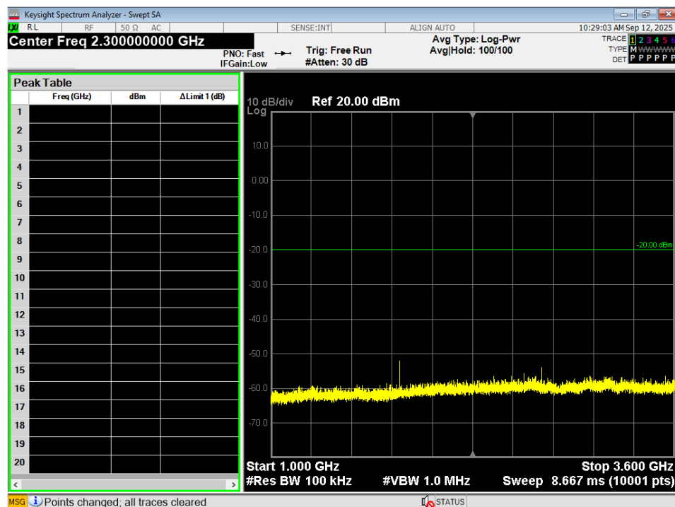
Figure 8 - Conducted Spurious Emissions Plot, LoRa, 1GHz – 3.6GHz
