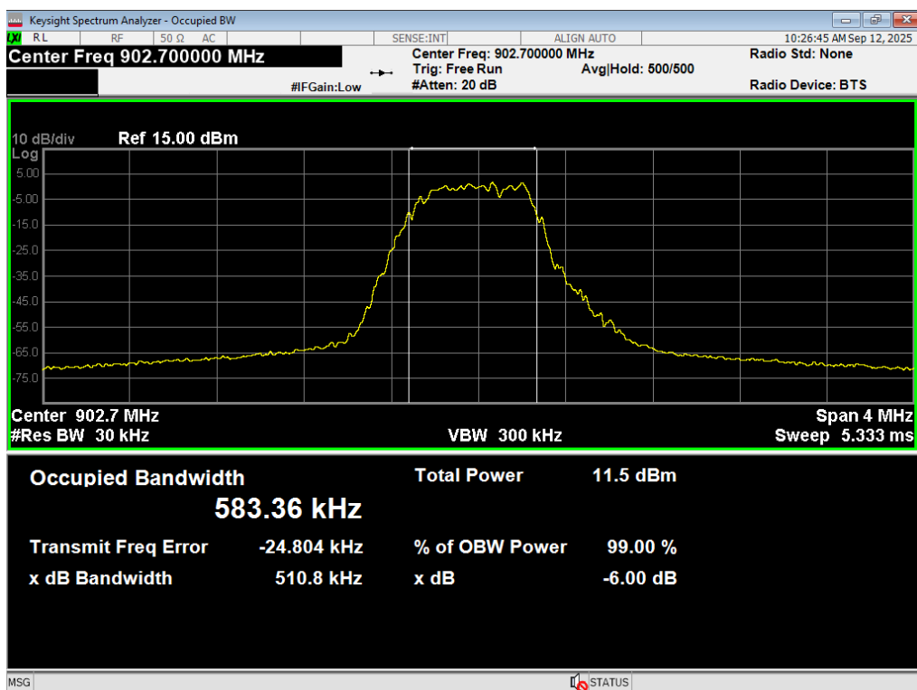
Occupied BW, DTS, 902.7MHz
