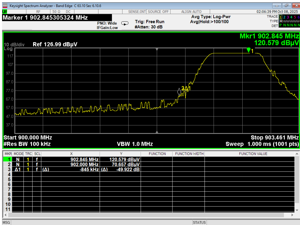
LBE Unrestricted, DTS
