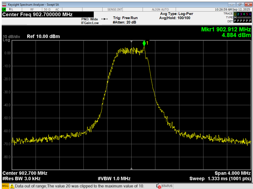
PSD, DTS, 902.7MHz
