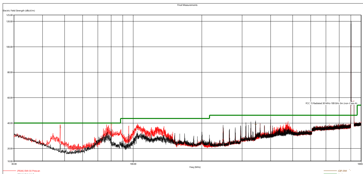
Figure 4 - Radiated Emissions Plot, Low
