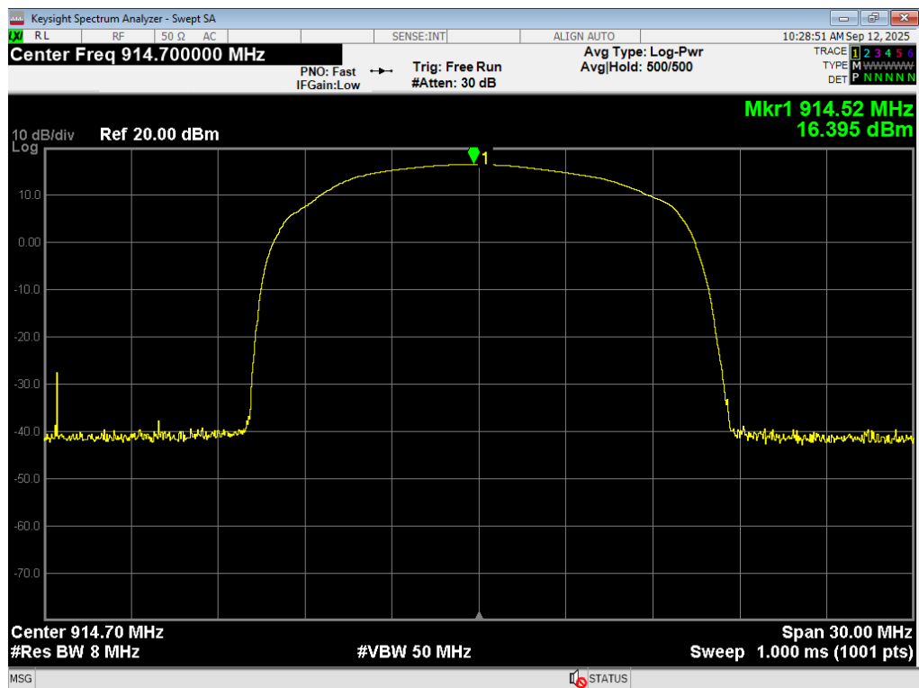
Peak Power, DTS, 914.7MHz
