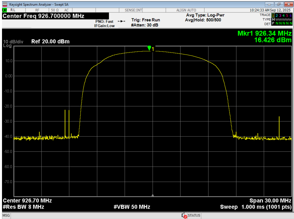
Peak Power, DTS, 926.7MHz
