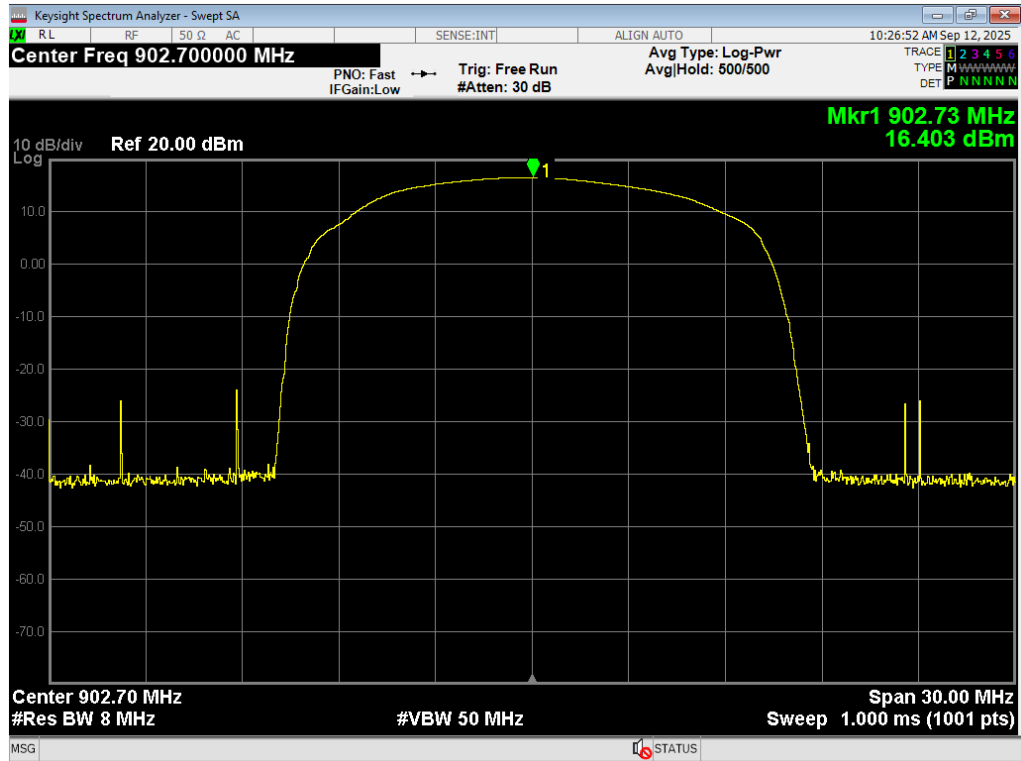
Peak Power, DTS, 902.7MHz
