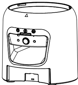
Feeder Base*1
