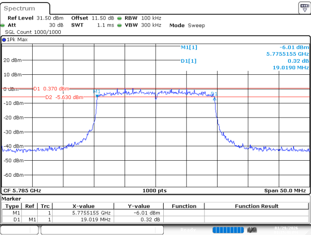
802.11ax20_5785MHz_RU_FULL_Ant 1
