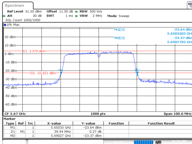
802.11ac40_5670MHz_Ant 1
