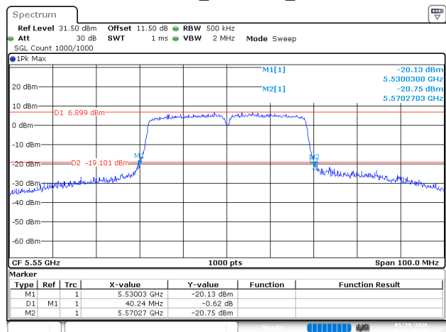
802.11ac40_5550MHz_Ant 2
