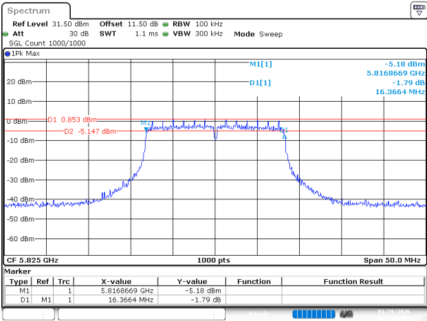
802.11a_5825MHz_Ant 1
