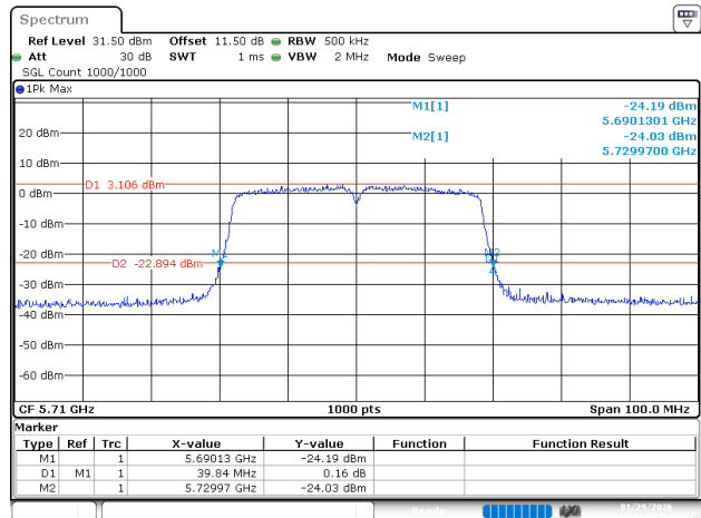
802.11ac40_5710MHz_Ant 1
