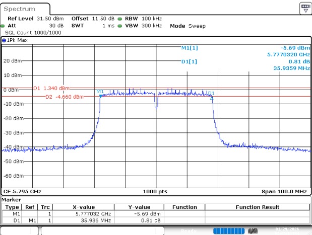
802.11ac40_5795MHz_Ant 2
