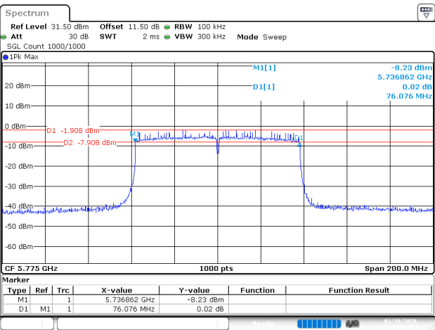
802.11ac80_5775MHz_Ant 2
