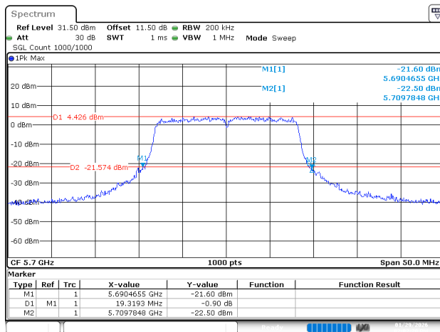
802.11a_5700MHz_Ant 2
