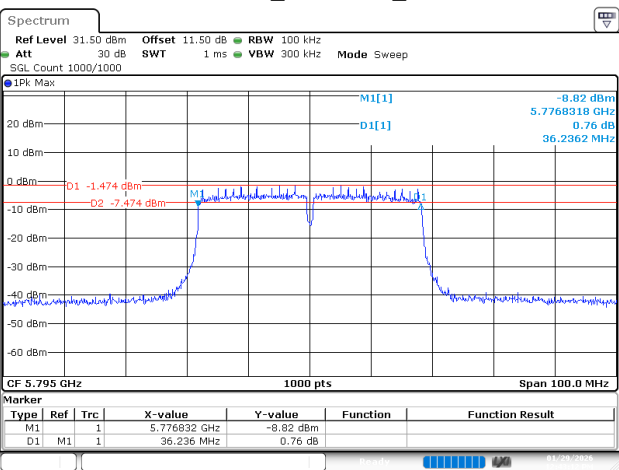
802.11ac40_5795MHz_Ant 1
