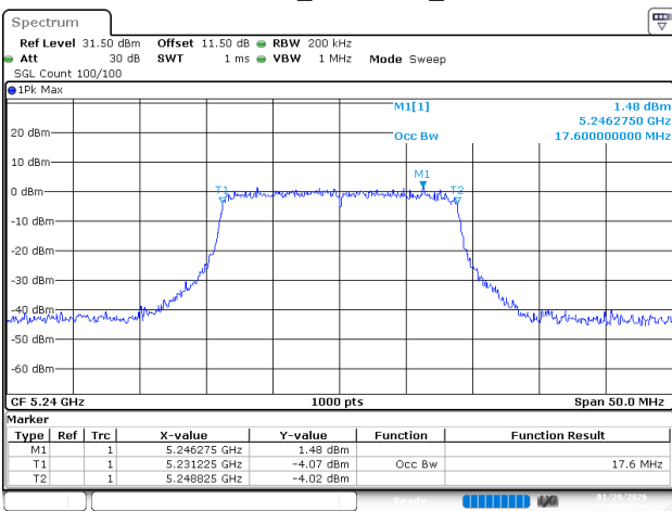
802.11ac20_5240MHz_Ant 1
