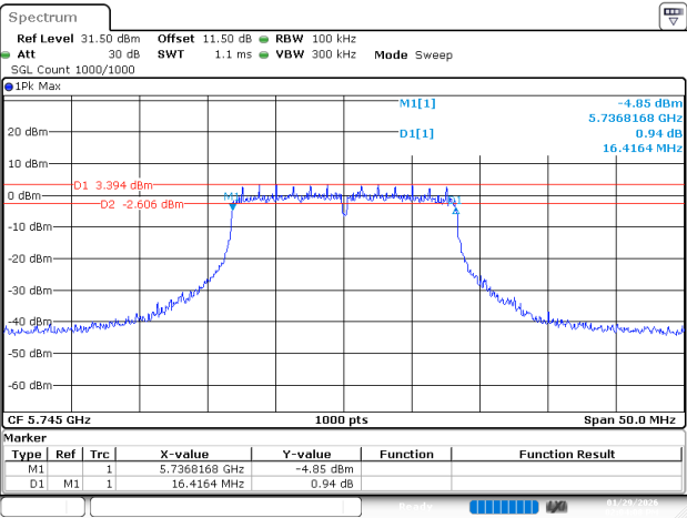
802.11a_5745MHz_Ant 2
