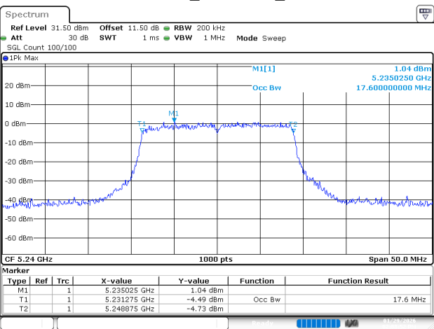
802.11ac20_5240MHz_Ant 2
