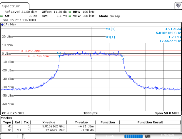
802.11ac20_5825MHz_Ant 2
