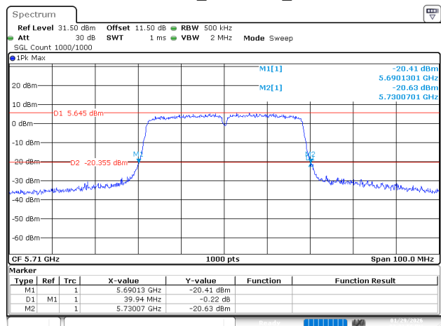
802.11ac40_5710MHz_Ant 2
