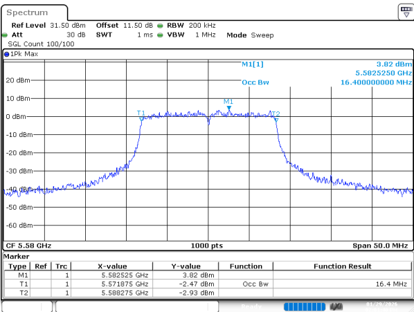
802.11a_5580MHz_Ant 2
