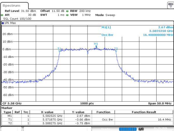
802.11a_5580MHz_Ant 1
