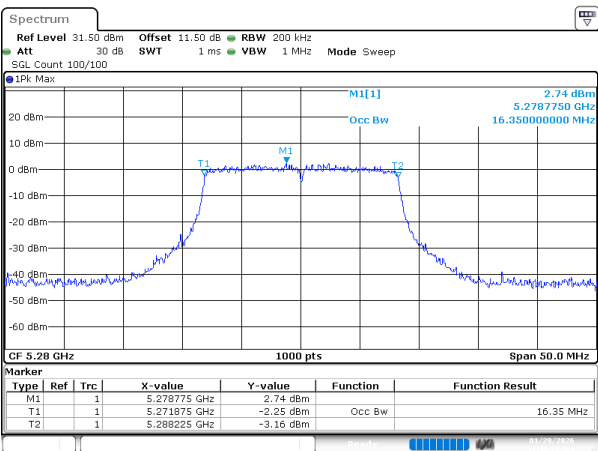
802.11a_5280MHz_Ant 1
