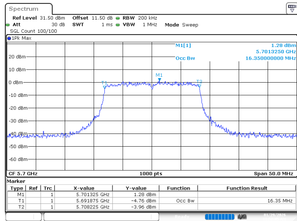
802.11a_5700MHz_Ant 1
