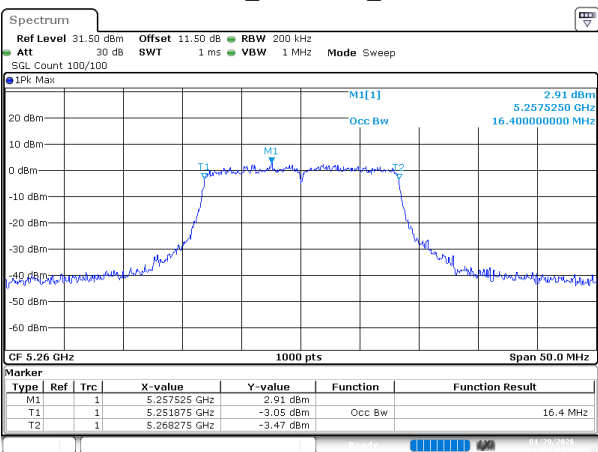
802.11a_5260MHz_Ant 2
