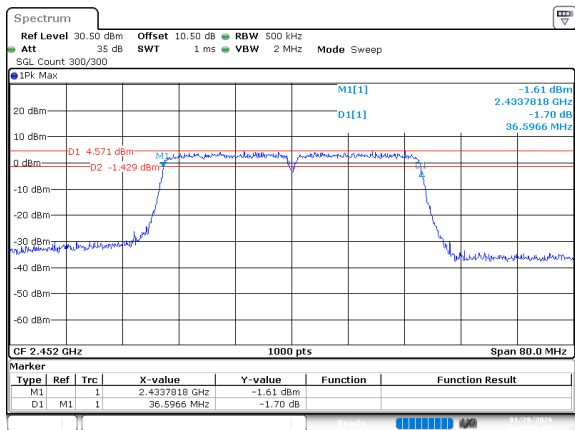
802.11n40_2452MHz_Ant 1
