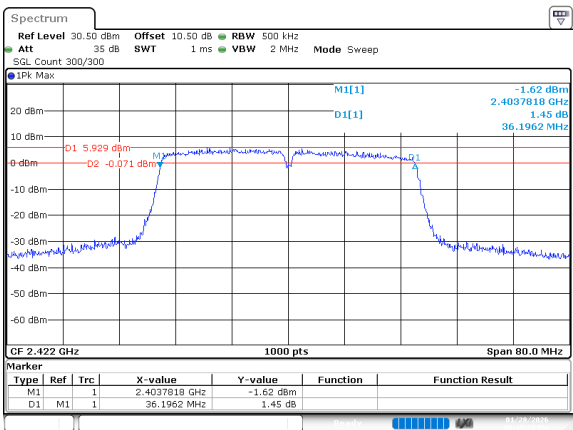
802.11n40_2422MHz_Ant 2
