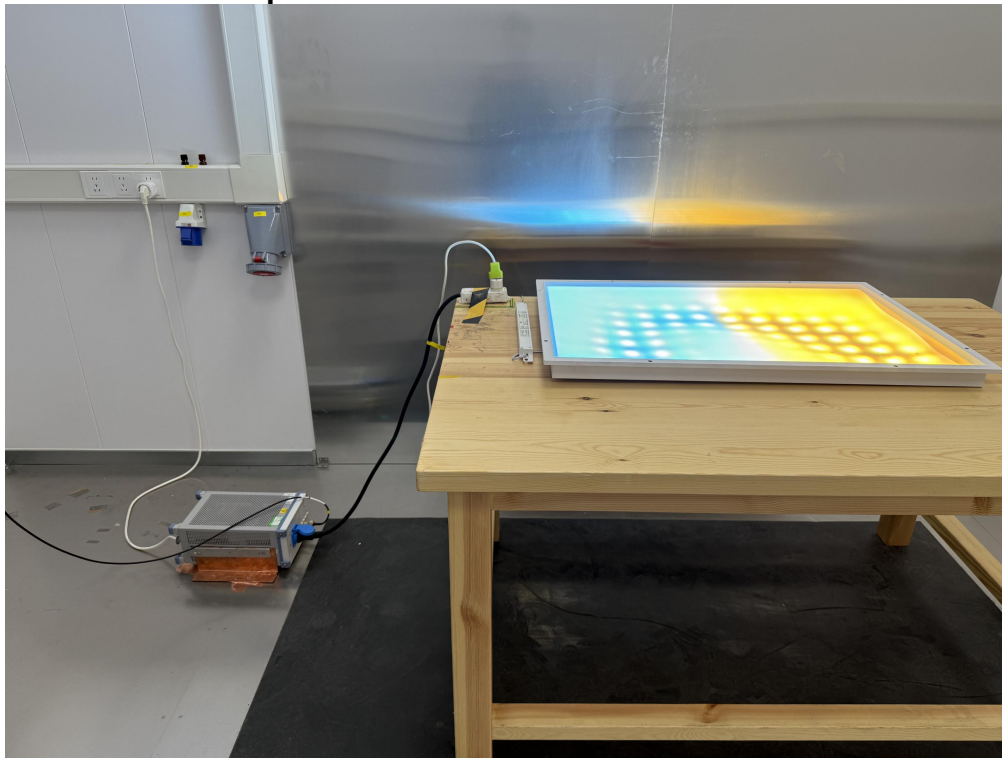
Photo 3 Test Setup Photos of AC Power Line Conducted Emissions
