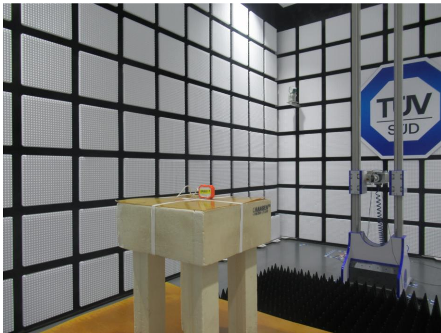
Radiated Emission Test 18GHz – 40GHz
