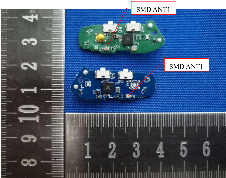
EUT View 2
