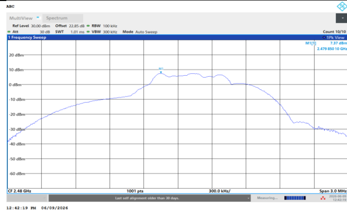
BLE_1M_Ant2_2480_0~Reference
