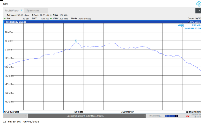
BLE_2M_Ant2_2402_0~Reference
