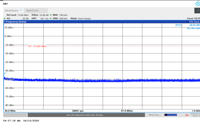
BLE_2M_Ant1_2440_30~1000
