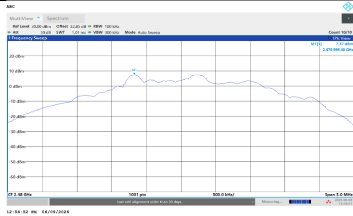
BLE_2M_Ant2_2480_0~Reference
