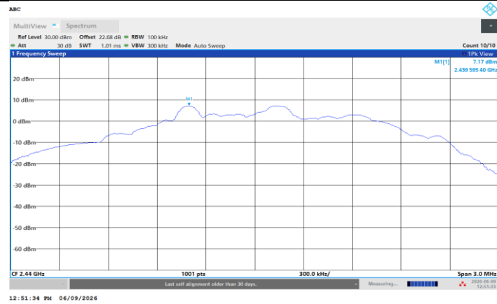
BLE_2M_Ant2_2440_0~Reference
