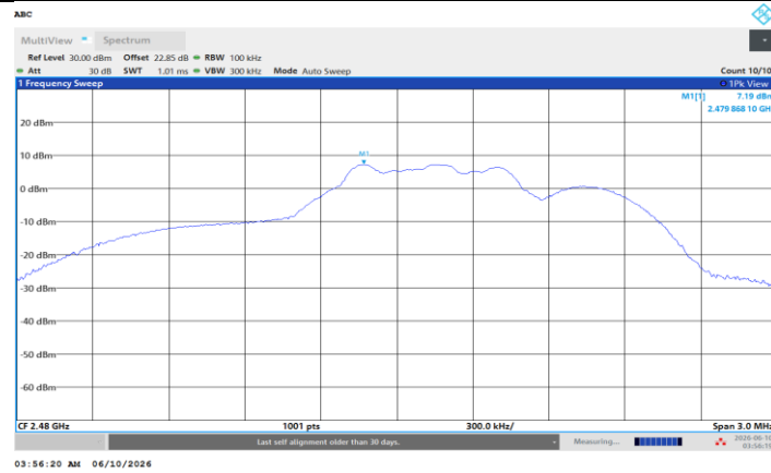
BLE_1M_Ant1_2480_0~Reference
