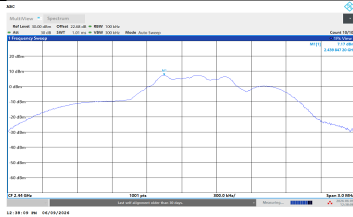
BLE_1M_Ant2_2440_0~Reference
