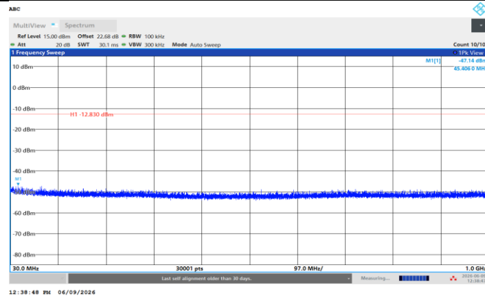
BLE_1M_Ant2_2440_30~1000
