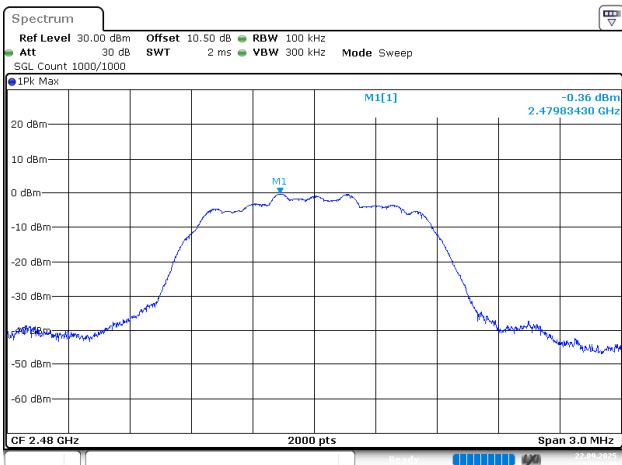
3EDR_DH1_High
