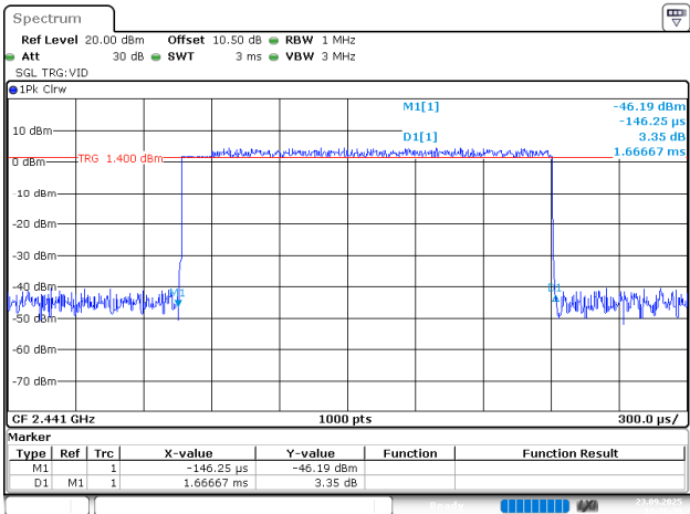
3EDR_DH3_Hopping
