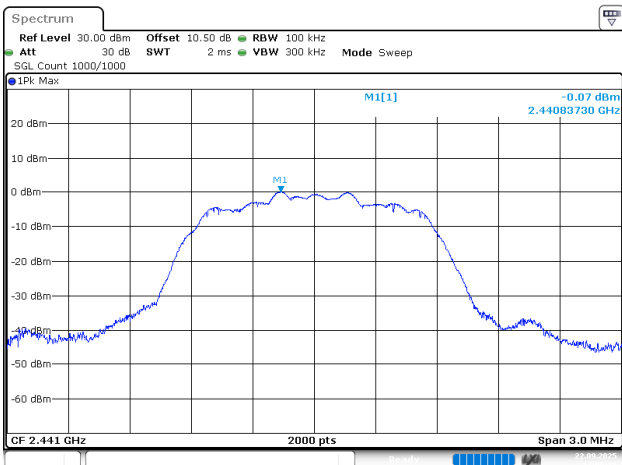
3EDR_DH1_Middle
