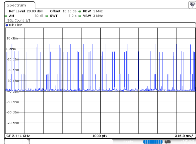
3EDR_DH3_Hopping
