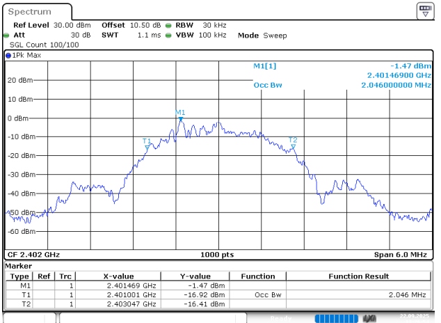
BLE_2M_Low_Channel
