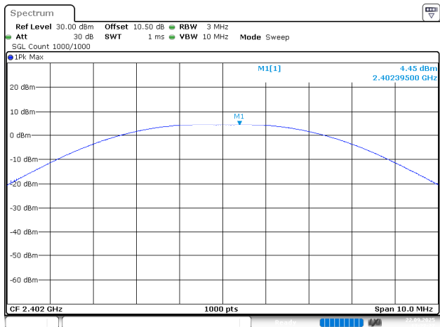
BLE_2M_Low_Channel
