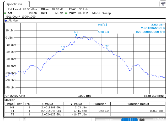
BDR_DH1_Low
