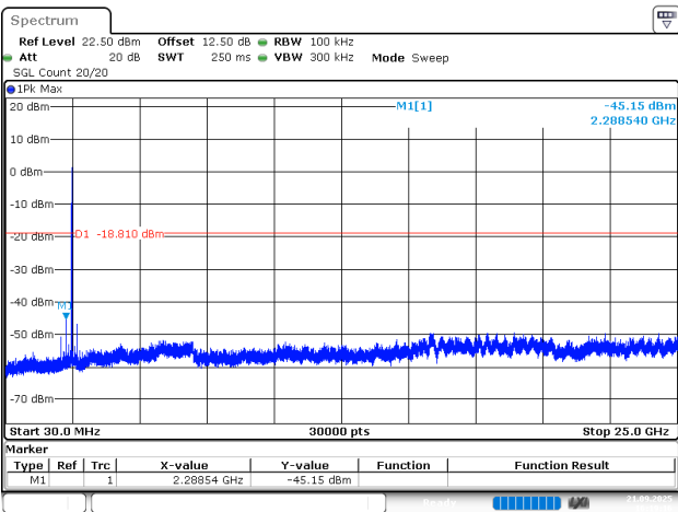
3EDR_DH1_High
