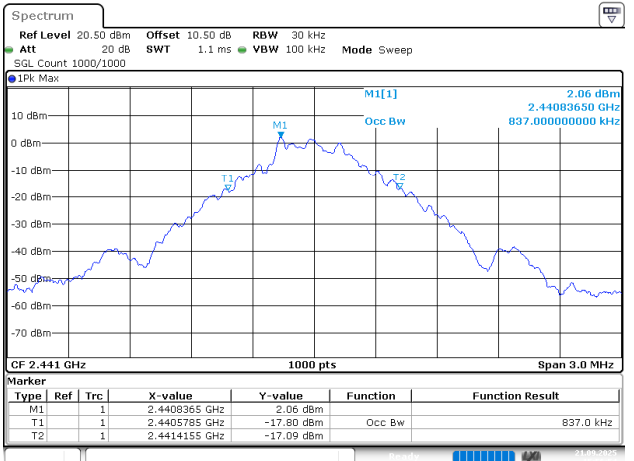
BDR_DH1_Middle
