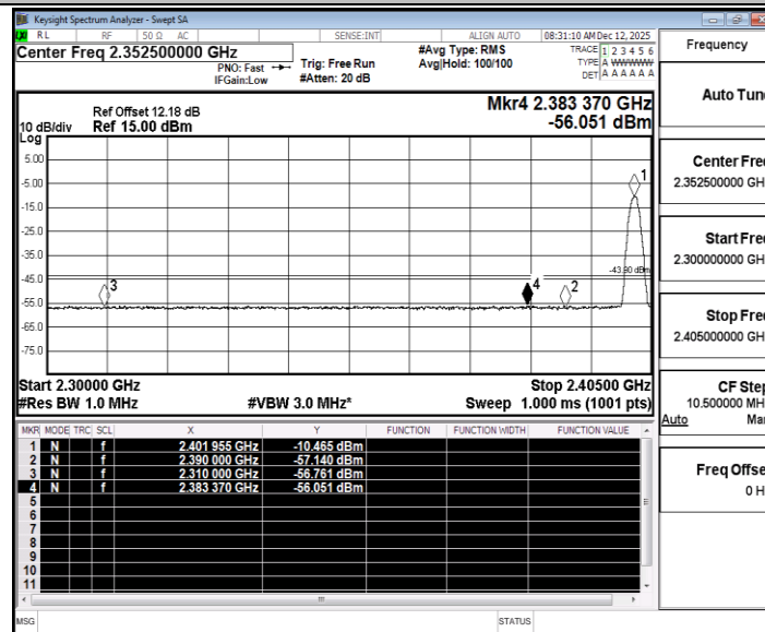
2.4G_Ant1_Low_2402_Peak
