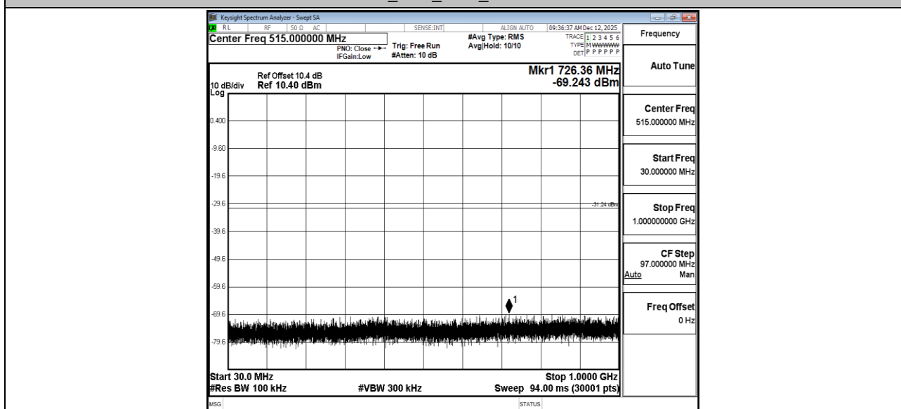
2.4G_Ant1_2440_30~1000
