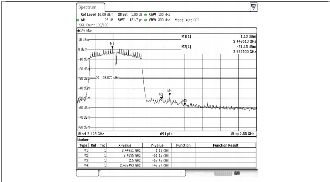
11N40MIMO-Ant0-2452-PASS
