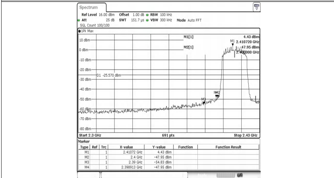
11N20MIMO-Ant0-2412-PASS
