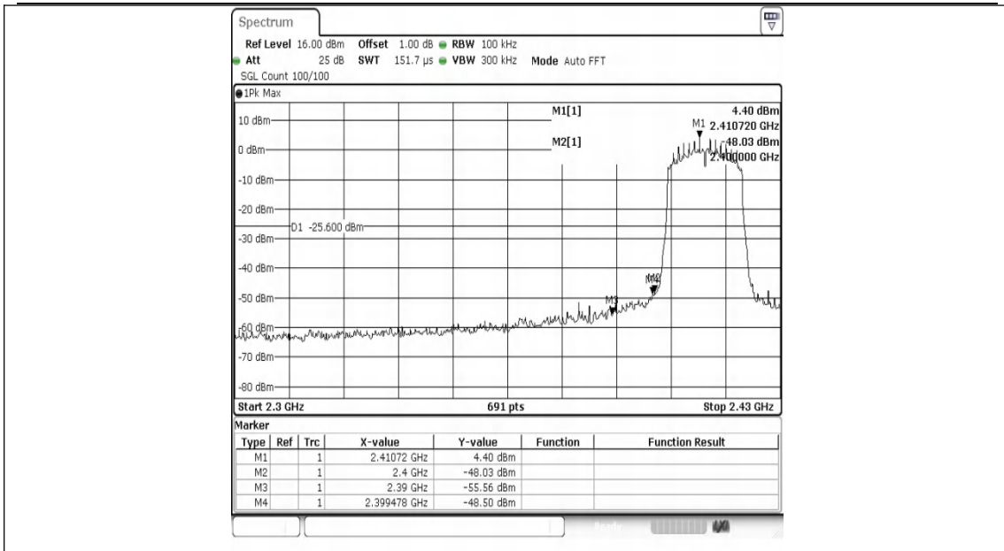
11N20MIMO-Ant0-2412-PASS
