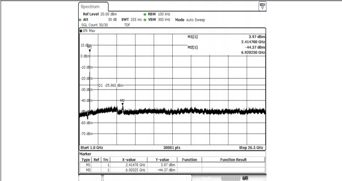
11B-Ant2-2412-1000~26500-PASS
